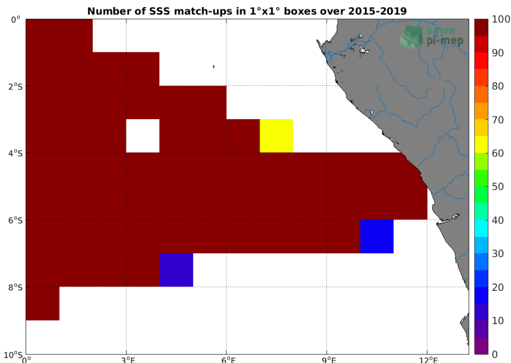
Figure 4: Number of SSS match-ups between TSG (GOSUD-Research-vessel) SSS and the SMAP SSS L3 v4 - Monthly (RSS) SSS product for the Congo river plume Pi-MEP region over 1°x1° boxes and for the full satellite product period.
