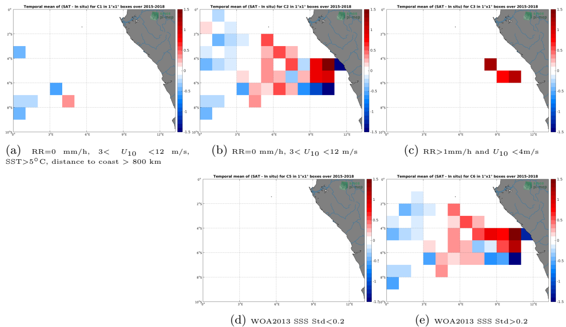
Figure 12: Temporal mean gridded over spatial boxes of size 1^\circ \times 1^\circ of \Delta SSS (SMAP-L3-RSS-V4-MONTHLY - TSG-GOSUD-Research-vessel) for 5 different subdatasets corresponding to:RR=0 mm/h, 3 < U_{10} < 12 m/s, SST > 5°C, distance to coast > 800 km (a), RR=0 mm/h, 3 < U_{10} < 12 m/s (b), RR > 1mm/h and U_{10} < 4 m/s (c), WOA2013 SSS Std < 0.2 (d), WOA2013 SSS Std > 0.2 (e).
