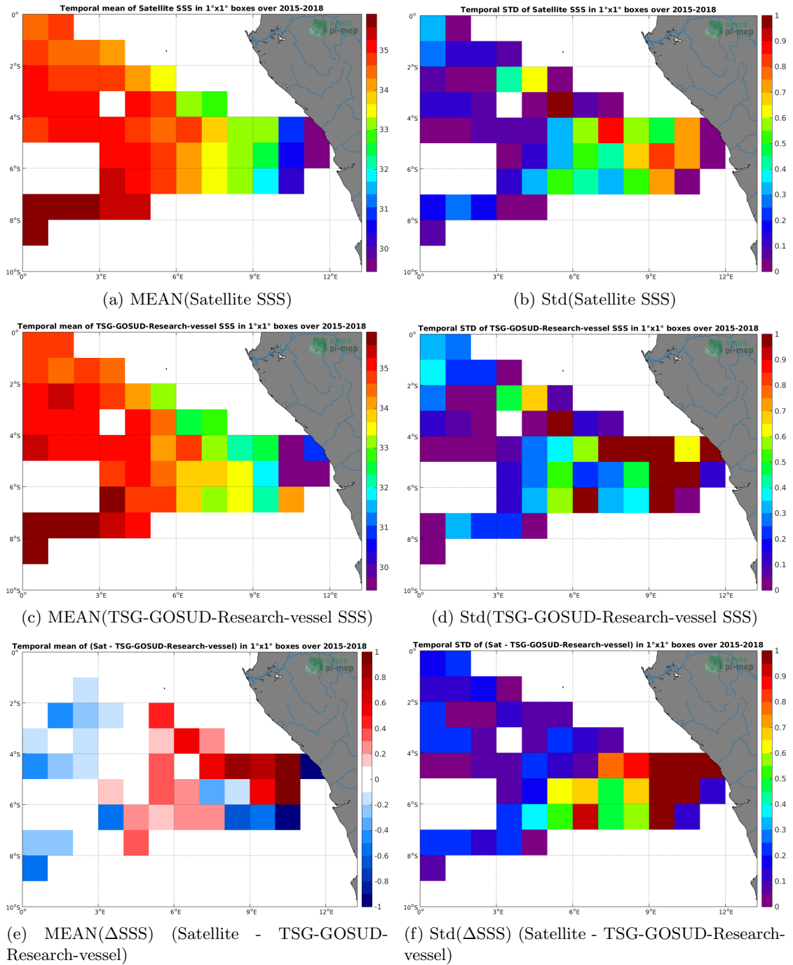
Figure 6: Temporal mean (left) and Std (right) of SSS from SMAP-L3-RSS-V4-MONTHLY (top), TSG-GOSUD-Research-vessel (middle), and of \Delta SSS (Satellite - TSG-GOSUD-Research-vessel). Only match-up pairs are used to generate these maps.
