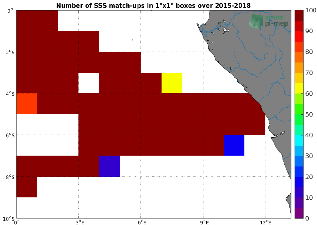
Figure 4: Number of SSS match-ups between TSG-GOSUD-Research-vessel SSS and the SMAP-L3-RSS-V4-MONTHLY SSS product for the Congo river plume Pi-MEP region over 1°x1° boxes and for the full satellite product period.
