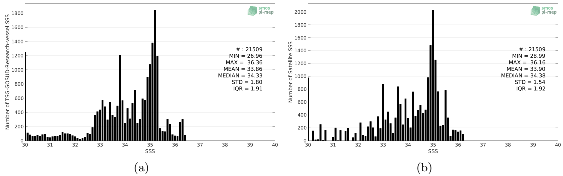
Figure 2: Histograms of SSS from TSG-GOSUD-Research-vessel (a) and SMAP-L3-RSS-V4-MONTHLY (b) considering all match-up pairs per bins of 0.1 over the Congo river plume Pi-MEP region and for the full satellite product period.
