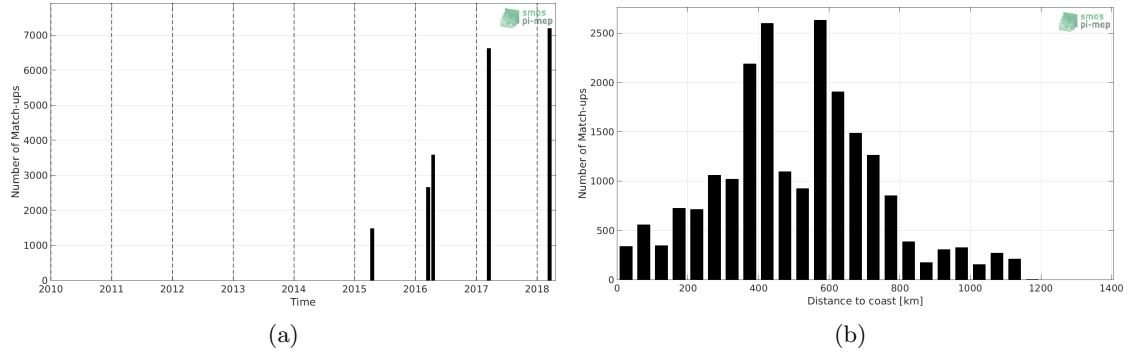
Figure 1: Number of match-ups between TSG-GOSUD-Research-vessel and SMAP-L3-RSS-V4-MONTHLY SSS as a function of time (a) and as function of the distance to coast (b) over the Congo river plume Pi-MEP region and for the full satellite product period.
