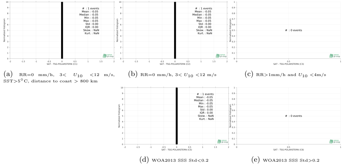
Figure 13: Normalized histogram of \Delta SSS (SMAP-L3-RSS-V3-8DAY-RUNNING-70KM - TSG-POLARSTERN) for 5 different subdatasets corresponding to: RR=0 mm/h, 3 < U_{10} < 12 m/s, SST>5°C, distance to coast > 800 km (a), RR=0 mm/h, 3 < U_{10} < 12 m/s (b), RR>1mm/h and U_{10} < 4 m/s (c), WOA2013 SSS Std<0.2 (d), WOA2013 SSS Std>0.2 (e).
