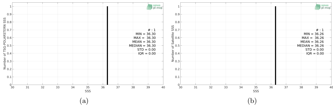
Figure 2: Histograms of SSS from TSG-POLARSTERN (a) and SMAP-L3-RSS-V3-8DAY-RUNNING-70KM (b) considering all match-up pairs per bins of 0.1 over the Congo river plume Pi-MEP region and for the full satellite product period.
