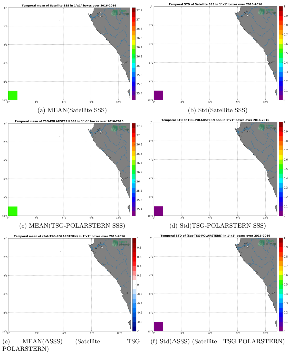
Figure 6: Temporal mean (left) and Std (right) of SSS from SMAP-L3-RSS-V3-8DAY-RUNNING-70KM (top), TSG-POLARSTERN (middle), and of \Delta SSS (Satellite - TSG-POLARSTERN). Only match-up pairs are used to generate these maps.
