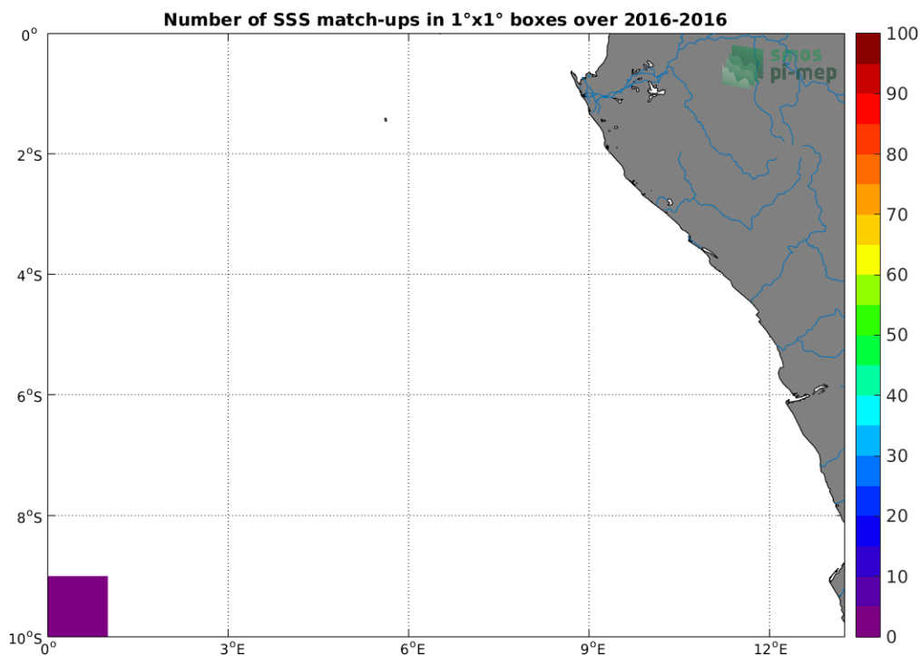
Figure 4: Number of SSS match-ups between TSG-POLARSTERN SSS and the SMAP-L3-RSS-V3-8DAY-RUNNING-70KM SSS product for the Congo river plume Pi-MEP region over 1^\circ \times 1^\circ boxes and for the full satellite product period.
