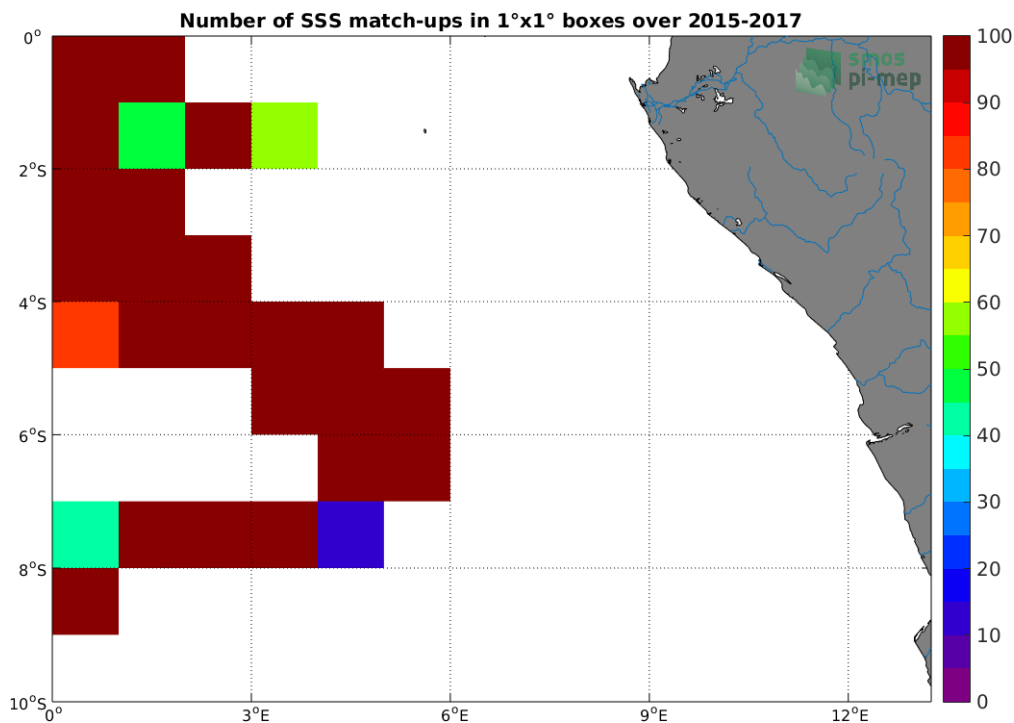
Figure 4: Number of SSS match-ups between TSG-GOSUD-Research-vessel and the SMAP-L3-RSS-V3-8DAY-RUNNING-70KM SSS product for the Congo river plume Pi-MEP region over 1^{\circ} \times 1^{\circ} boxes and for the full satellite product period.
