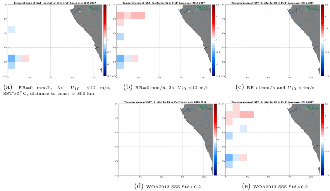
Figure 12: Temporal mean gridded over spatial boxes of size 1^\circ \times 1^\circ of \Delta SSS (SMAP-L3-RSS-V3-8DAY-RUNNING-70KM - TSG-GOSUD-Research-vessel) for 5 different subdatasets corresponding to:RR=0 mm/h, 3 < U_{10} < 12 m/s, SST >5^\circ C, distance to coast > 800 km (a), RR=0 mm/h, 3 < U_{10} < 12 m/s (b), RR >1 mm/h and U_{10} < 4 m/s (c), WOA2013 SSS Std <0.2 (d), WOA2013 SSS Std >0.2 (e).
