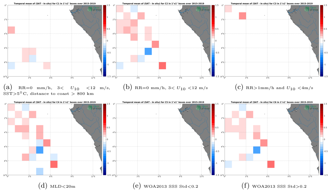
Figure 12: Temporal mean gridded over spatial boxes of size 1^\circ \times 1^\circ of \Delta SSS (SMAP-L3-RSS-V3-8DAY-RUNNING-70KM - Argo) for 6 different subdatasets corresponding to:RR=0 mm/h, 3 < U_{10} < 12 m/s, SST >5^\circ C, distance to coast > 800 km (a), RR=0 mm/h, 3 < U_{10} < 12 m/s (b), RR >1 mm/h and U_{10} < 4 m/s (c),MLD <20 m (d),WOA2013 SSS Std <0.2 (e),WOA2013 SSS Std >0.2 (f).
