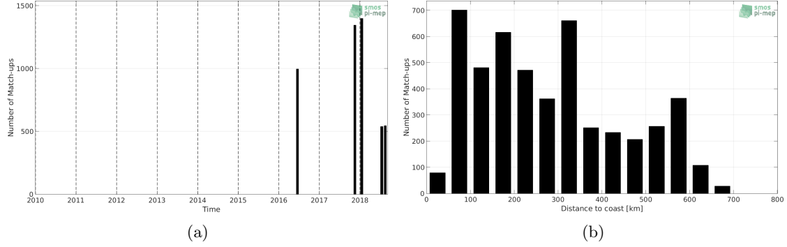
Figure 1: Number of match-ups between TSG-LEGOS-DM and SMAP-L3-RSS-V3-8DAY-RUNNING-40KM SSS as a function of time (a) and as function of the distance to coast (b) over the Congo river plume Pi-MEP region and for the full satellite product period.
