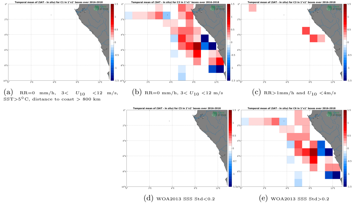
Figure 12: Temporal mean gridded over spatial boxes of size 1^\circ \times 1^\circ of \Delta SSS (SMAP-L3-RSS-V3-8DAY-RUNNING-40KM - TSG-LEGOS-DM) for 5 different subdatasets corresponding to: RR=0 mm/h, 3 < U_{10} < 12 m/s, SST > 5^\circ C , distance to coast > 800 km (a), RR=0 mm/h, 3 < U_{10} < 12 m/s (b), RR > 1 mm/h and U_{10} < 4 m/s (c), WOA2013 SSS Std < 0.2 (d), WOA2013 SSS Std > 0.2 (e).
