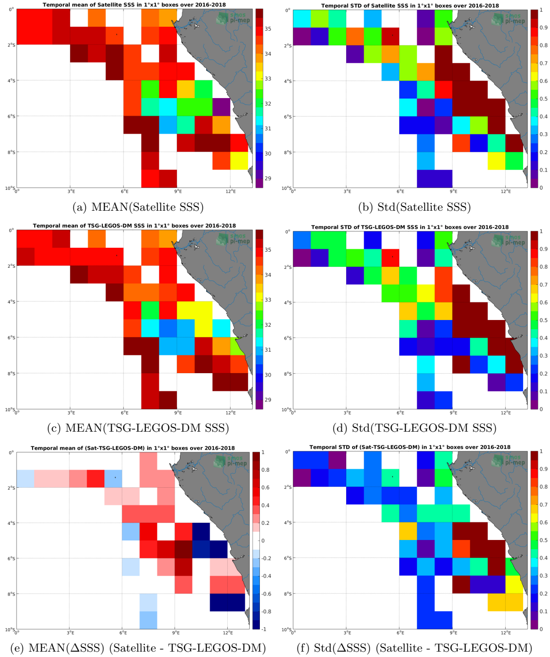
Figure 6: Temporal mean (left) and Std (right) of SSS from SMAP-L3-RSS-V3-8DAY-RUNNING-40KM (top), TSG-LEGOS-DM (middle), and of \Delta SSS (Satellite - TSG-LEGOS-DM). Only match-up pairs are used to generate these maps.
