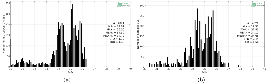
Figure 2: Histograms of SSS from TSG-LEGOS-DM (a) and SMAP-L3-RSS-V3-8DAY-RUNNING-40KM (b) considering all match-up pairs per bins of 0.1 over the Congo river plume Pi-MEP region and for the full satellite product period.
