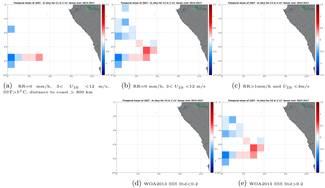
Figure 12: Temporal mean gridded over spatial boxes of size 1^\circ \times 1^\circ of \Delta SSS (SMAP-L3-RSS-V3-MONTHLY-70KM - TSG-GOSUD-Research-vessel) for 5 different subdatasets corresponding to:RR=0 mm/h, 3 < U_{10} < 12 m/s, SST > 5^\circ\text{C} , distance to coast > 800 km (a), RR=0 mm/h, 3 < U_{10} < 12 m/s (b), RR > 1 mm/h and U_{10} < 4 m/s (c), WOA2013 SSS Std < 0.2 (d), WOA2013 SSS Std > 0.2 (e).
