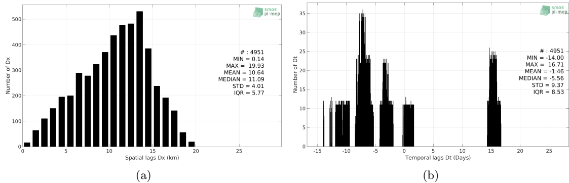
Figure 5: Histograms of the spatial (a) and temporal (b) lags between the time of the TSG-LEGOS-DM measurements and the date of the corresponding SMAP-L3-RSS-V3-MONTHLY-0.25DEG-40KM SSS product.
