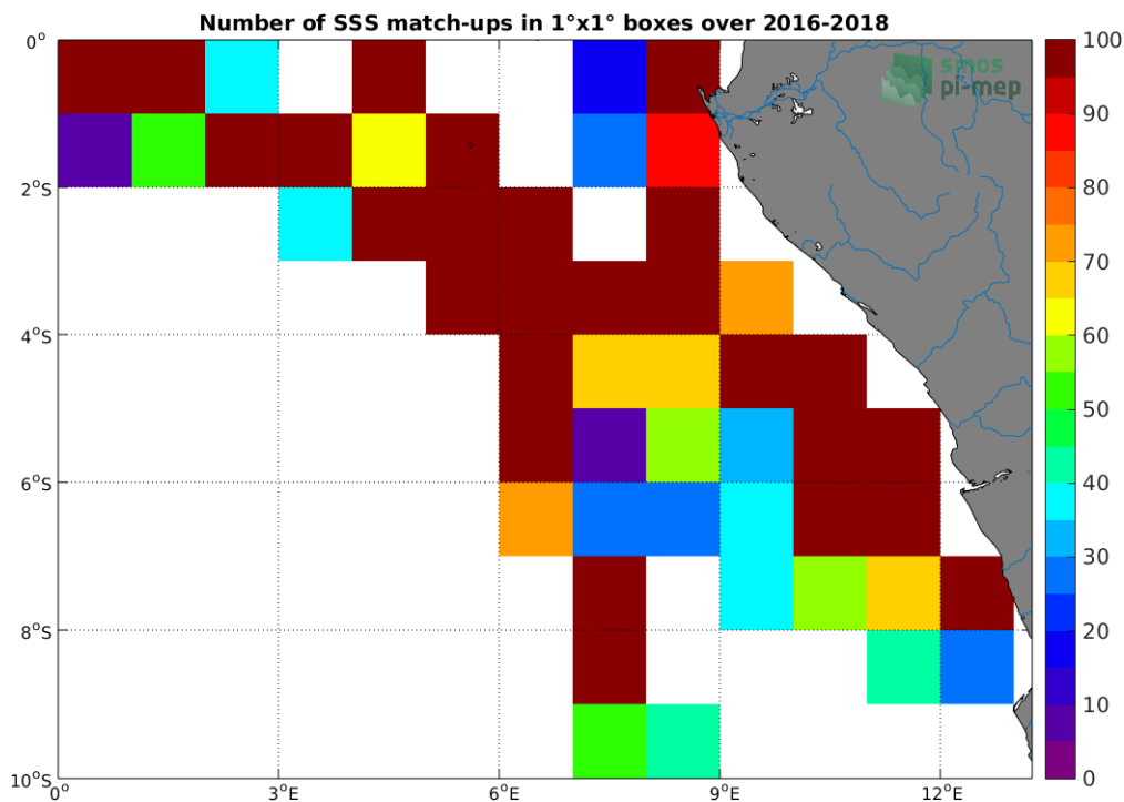
Figure 4: Number of SSS match-ups between TSG-LEGOS-DM SSS and the SMAP-L3-RSS-V3-MONTHLY-0.25DEG-40KM SSS product for the Congo river plume Pi-MEP region over 1^\circ \times 1^\circ boxes and for the full satellite product period.
