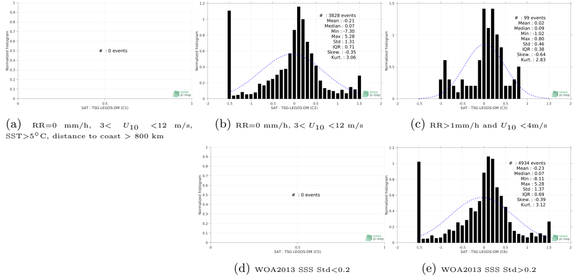
Figure 13: Normalized histogram of \Delta SSS (SMAP-L3-RSS-V3-MONTHLY-0.25DEG-40KM - TSG-LEGOS-DM) for 5 different subdatasets corresponding to: RR=0 mm/h, 3 < U_{10} < 12 m/s, SST > 5°C, distance to coast > 800 km (a), RR=0 mm/h, 3 < U_{10} < 12 m/s (b), RR > 1mm/h and U_{10} < 4 m/s (c), WOA2013 SSS Std < 0.2 (d), WOA2013 SSS Std > 0.2 (e).
