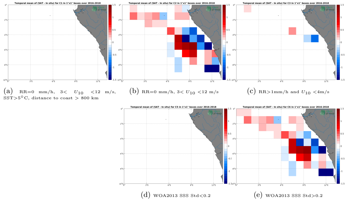
Figure 12: Temporal mean gridded over spatial boxes of size 1^\circ \times 1^\circ of \Delta SSS (SMAP-L3-RSS-V3-MONTHLY-0.25DEG-40KM - TSG-LEGOS-DM) for 5 different subdatasets corresponding to:RR=0 mm/h, 3 < U_{10} < 12 m/s, SST >5^\circ C, distance to coast > 800 km (a), RR=0 mm/h, 3 < U_{10} < 12 m/s (b), RR >1 mm/h and U_{10} < 4 m/s (c), WOA2013 SSS Std <0.2 (d), WOA2013 SSS Std >0.2 (e).
