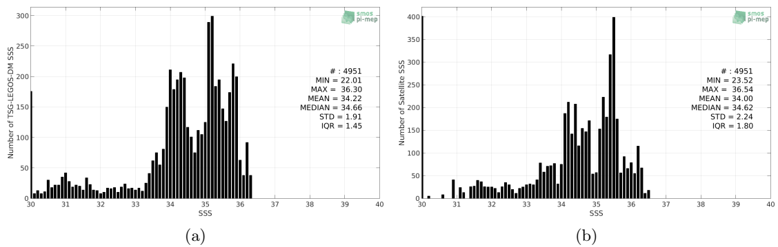
Figure 2: Histograms of SSS from TSG-LEGOS-DM (a) and SMAP-L3-RSS-V3-MONTHLY-0.25DEG-40KM (b) considering all match-up pairs per bins of 0.1 over the Congo river plume Pi-MEP region and for the full satellite product period.
