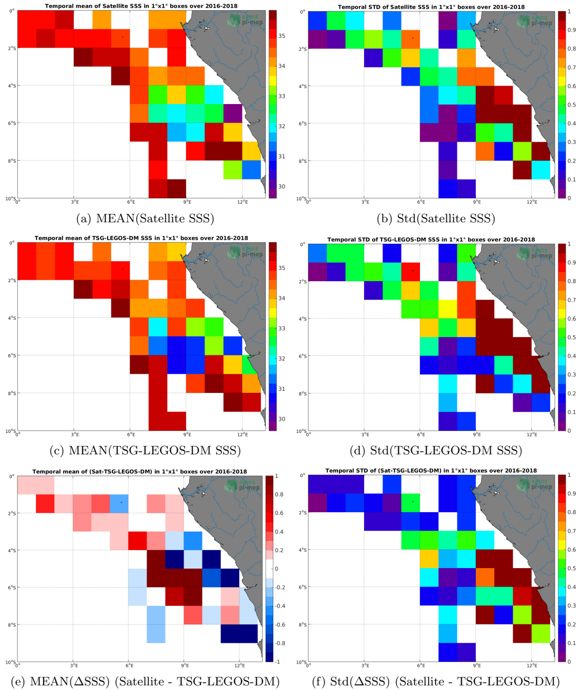
Figure 6: Temporal mean (left) and Std (right) of SSS from SMAP-L3-RSS-V3-MONTHLY-0.25DEG-40KM (top), TSG-LEGOS-DM (middle), and of \Delta SSS (Satellite - TSG-LEGOS-DM). Only match-up pairs are used to generate these maps.
