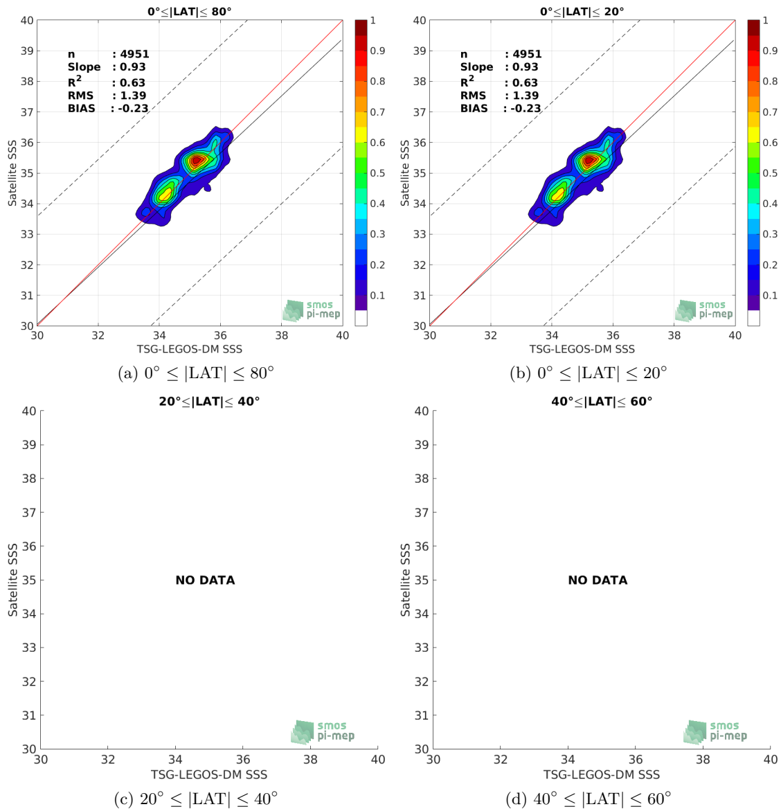
Figure 9: Contour maps of the concentration of SMAP-L3-RSS-V3-MONTHLY-0.25DEG-40KM SSS (y-axis) versus TSG-LEGOS-DM SSS (x-axis) at match-up pairs for different latitude bands. For each plot, the red line shows x=y . The black thin and dashed lines indicate a linear fit through the data cloud and the \pm 95\% confidence levels, respectively. The number match-up pairs n , the slope and R^2 coefficient of the linear fit, the root mean square (RMS) and the mean bias between satellite and in situ data are indicated for each latitude band in each plots.
