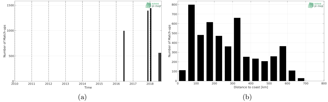
Figure 1: Number of match-ups between TSG-LEGOS-DM and SMAP-L3-RSS-V3-MONTHLY-0.25DEG-40KM SSS as a function of time (a) and as function of the distance to coast (b) over the Congo river plume Pi-MEP region and for the full satellite product period.
