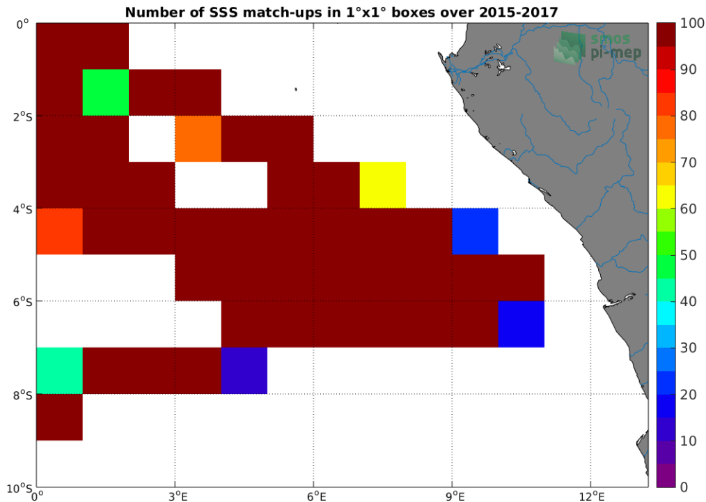
Figure 4: Number of SSS match-ups between TSG-GOSUD-Research-vessel SSS and the SMAP-L3-RSS-V3-MONTHLY-0.25DEG-40KM SSS product for the Congo river plume Pi-MEP region over 1^{\circ} \times 1^{\circ} boxes and for the full satellite product period.
