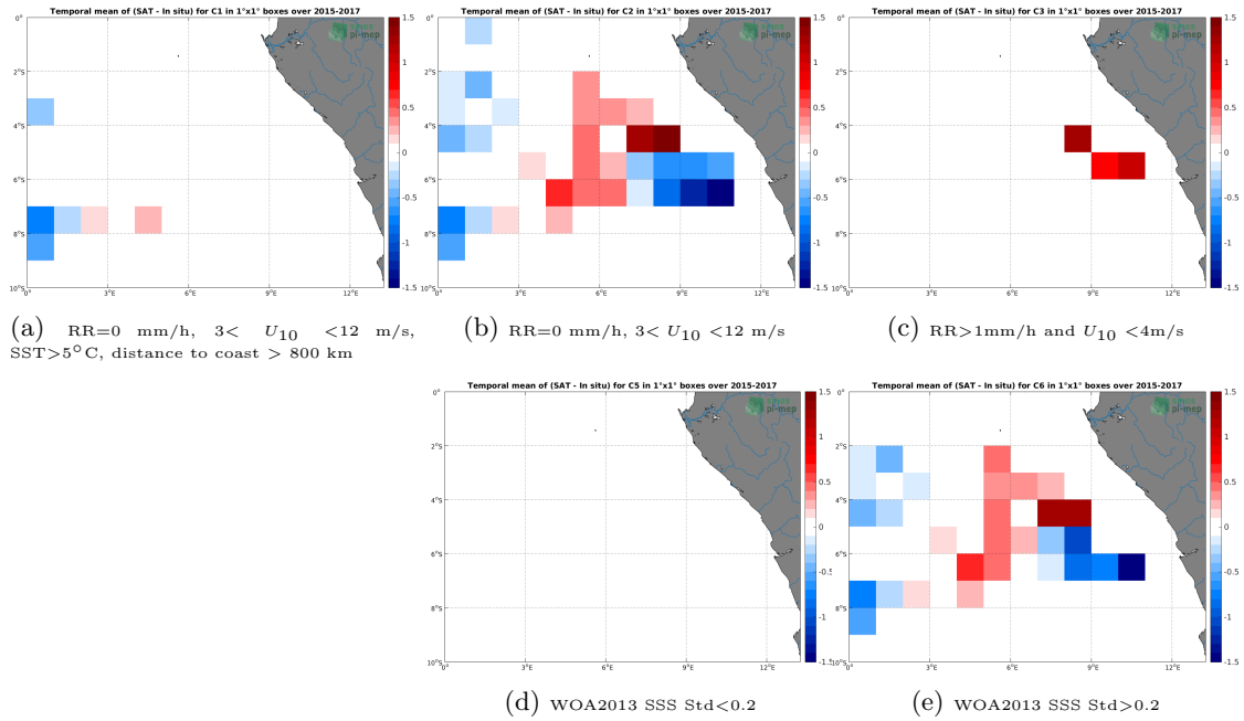
Figure 12: Temporal mean gridded over spatial boxes of size 1^\circ \times 1^\circ of \Delta SSS (SMAP-L3-RSS-V3-MONTHLY-0.25DEG-40KM - TSG-GOSUD-Research-vessel) for 5 different subdatasets corresponding to:RR=0 mm/h, 3 < U_{10} < 12 m/s, SST >5^\circ C, distance to coast > 800 km (a), RR=0 mm/h, 3 < U_{10} < 12 m/s (b), RR >1 mm/h and U_{10} < 4 m/s (c), WOA2013 SSS Std <0.2 (d), WOA2013 SSS Std >0.2 (e).
