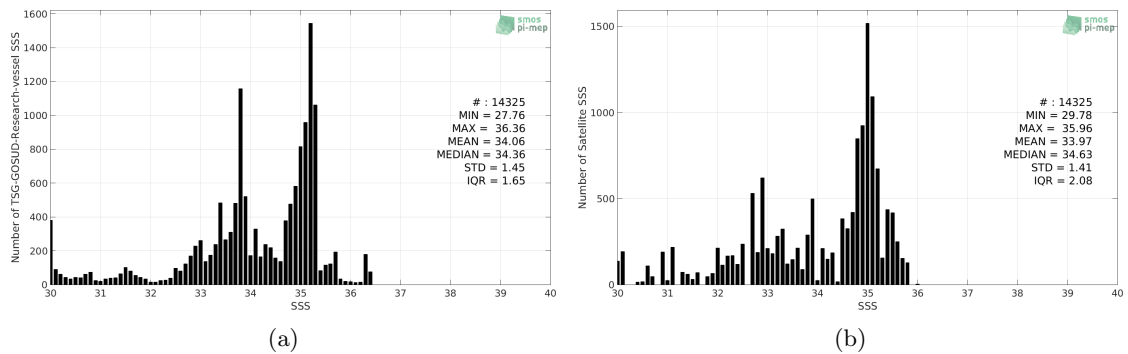
Figure 2: Histograms of SSS from TSG-GOSUD-Research-vessel (a) and SMAP-L3-RSS-V3-MONTHLY-0.25DEG-40KM (b) considering all match-up pairs per bins of 0.1 over the Congo river plume Pi-MEP region and for the full satellite product period.
