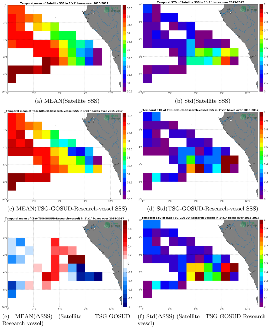
Figure 6: Temporal mean (left) and Std (right) of SSS from SMAP-L3-RSS-V3-MONTHLY-0.25DEG-40KM (top), TSG-GOSUD-Research-vessel (middle), and of \Delta SSS (Satellite - TSG-GOSUD-Research-vessel). Only match-up pairs are used to generate these maps.
