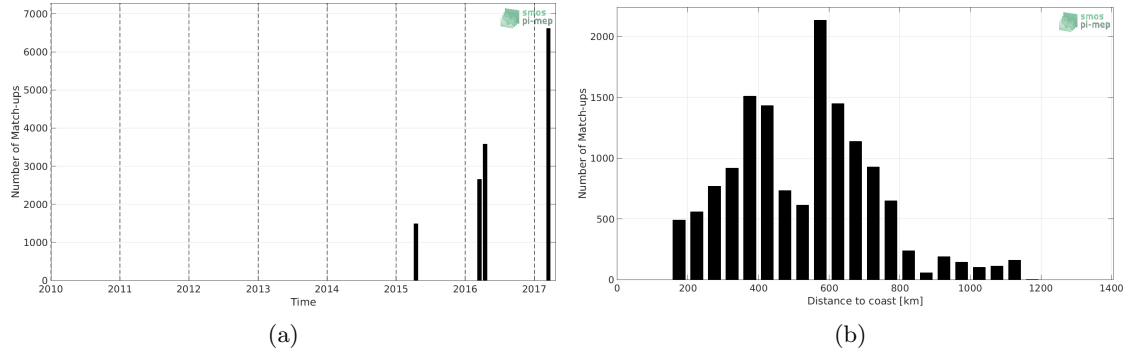
Figure 1: Number of match-ups between TSG-GOSUD-Research-vessel and SMAP-L3-RSS-V3-MONTHLY-0.25DEG-40KM SSS as a function of time (a) and as function of the distance to coast (b) over the Congo river plume Pi-MEP region and for the full satellite product period.
