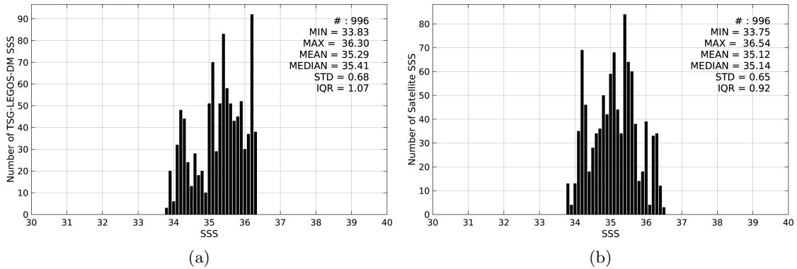
Figure 2: Histograms of SSS from TSG-LEGOS-DM (a) and SMAP-L3-RSS-V2-8DAY-RUNNING-40KM (b) considering all match-up pairs per bins of 0.1 over the Congo river plume Pi-MEP region and for the full satellite product period.
