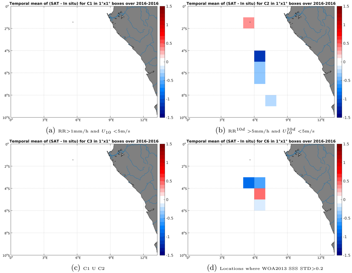
Figure 12: Temporal mean gridded over spatial boxes of size 1^\circ \times 1^\circ of \Delta SSS (SMAP-L3-RSS-V2-8DAY-RUNNING-40KM - TSG-LEGOS-DM) for 4 different subdatasets corresponding to: RR > 1mm/h and U_{10} < 5m/s (a), RR^{10d} > 5mm/h and U_{10}^{10d} < 5m/s (b), C1 U C2 (c), Locations where WOA2013 SSS STD > 0.2 (d).
