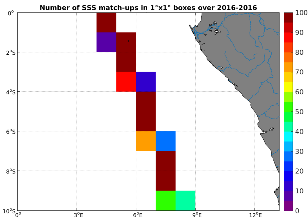
Figure 4: Number of SSS match-ups between TSG-LEGOS-DM SSS and the SMAP-L3-RSS-V2-8DAY-RUNNING-40KM SSS product for the Congo river plume Pi-MEP region over 1°x1° boxes and for the full satellite product period.
