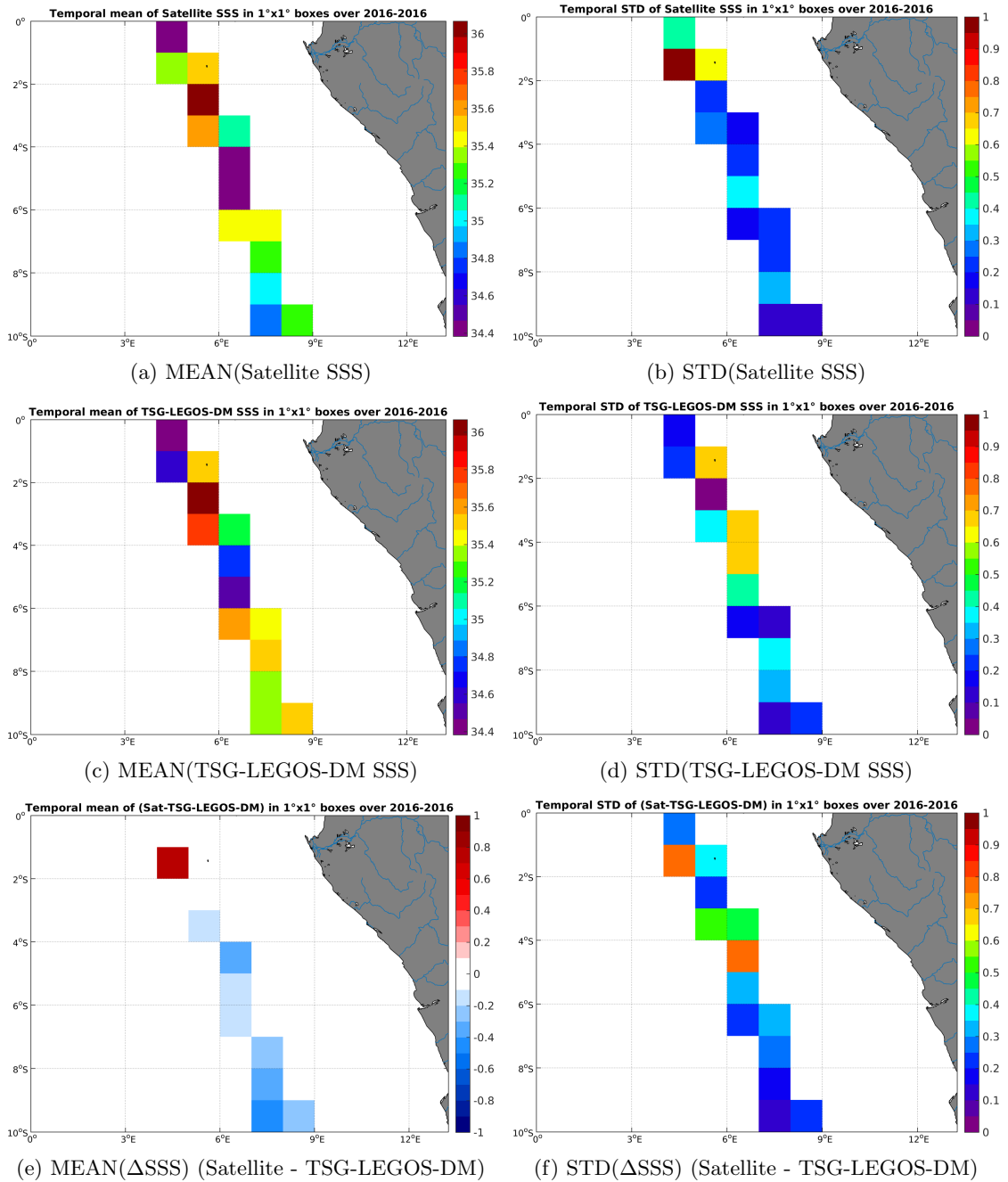
Figure 6: Temporal mean (left) and STD (right) of SSS from SMAP-L3-RSS-V2-8DAY-RUNNING-40KM (top), TSG-LEGOS-DM (middle), and of \Delta SSS (Satellite - TSG-LEGOS-DM). Only match-up pairs are used to generate these maps.
