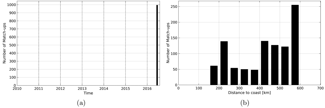
Figure 1: Number of match-ups between TSG-LEGOS-DM and SMAP-L3-RSS-V2-8DAY-RUNNING-40KM SSS as a function of time (a) and as function of the distance to coast (b) over the Congo river plume Pi-MEP region and for the full satellite product period.
