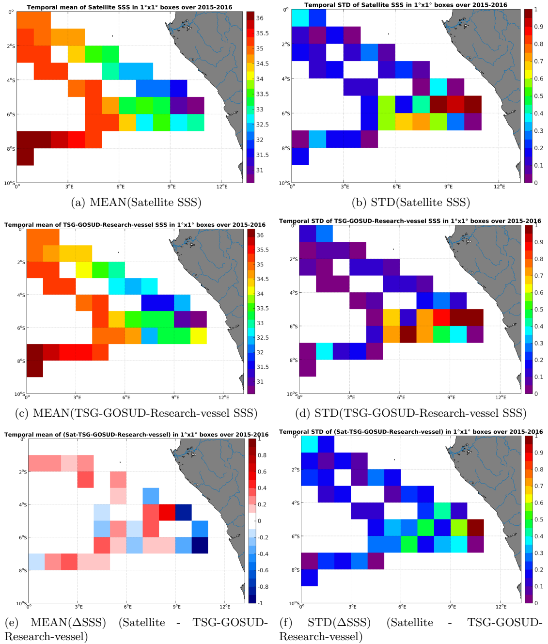
Figure 6: Temporal mean (left) and STD (right) of SSS from SMAP-L3-RSS-V2-8DAY-RUNNING-40KM (top), TSG-GOSUD-Research-vessel (middle), and of \Delta SSS (Satellite - TSG-GOSUD-Research-vessel). Only match-up pairs are used to generate these maps.
