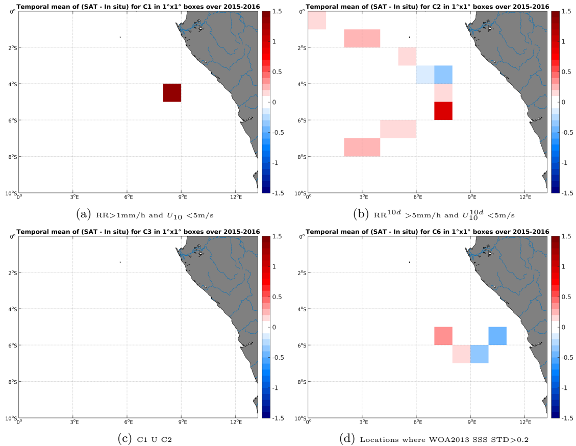
Figure 12: Temporal mean gridded over spatial boxes of size 1^\circ \times 1^\circ of \Delta SSS (SMAP-L3-RSS-V2-8DAY-RUNNING-40KM - TSG-GOSUD-Research-vessel) for 4 different subdatasets corresponding to: RR > 1\text{mm/h} and U_{10} < 5\text{m/s} (a), RR^{10d} > 5\text{mm/h} and U_{10}^{10d} < 5\text{m/s} (b), C1 U C2 (c), Locations where WOA2013 SSS STD > 0.2 (d).
