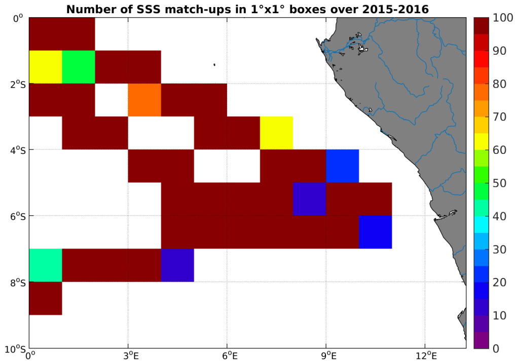
Figure 4: Number of SSS match-ups between TSG-GOSUD-Research-vessel SSS and the SMAP-L3-RSS-V2-8DAY-RUNNING-40KM SSS product for the Congo river plume Pi-MEP region over 1°x1° boxes and for the full satellite product period.
