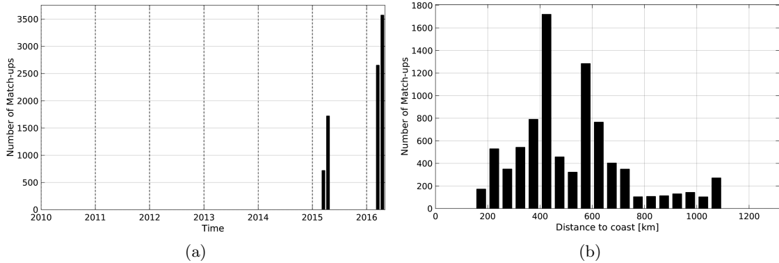
Figure 1: Number of match-ups between TSG-GOSUD-Research-vessel and SMAP-L3-RSS-V2-8DAY-RUNNING-40KM SSS as a function of time (a) and as function of the distance to coast (b) over the Congo river plume Pi-MEP region and for the full satellite product period.
