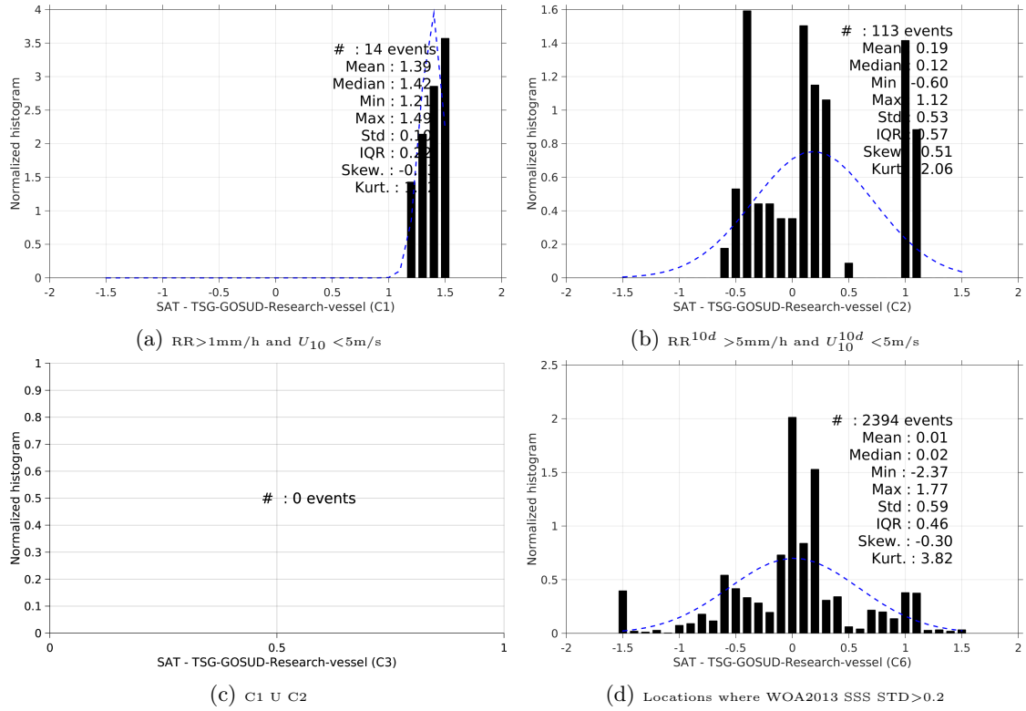
Figure 13: Normalized histogram of \Delta\text{SSS} (SMAP-L3-RSS-V2-8DAY-RUNNING-40KM - TSG-GOSUD-Research-vessel) for 6 different subdatasets corresponding to: RR > 1mm/h and U_{10} < 5\text{m/s} (a), RR^{10d} > 5\text{mm/h} and U_{10}^{10d} < 5\text{m/s} (b), C1 U C2 (c), Locations where WOA2013 SSS STD > 0.2 (d).
