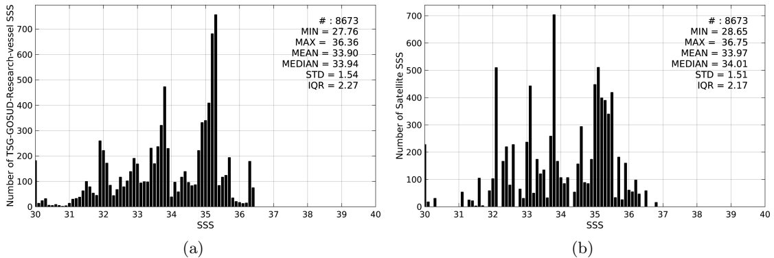
Figure 2: Histograms of SSS from TSG-GOSUD-Research-vessel (a) and SMAP-L3-RSS-V2-8DAY-RUNNING-40KM (b) considering all match-up pairs per bins of 0.1 over the Congo river plume Pi-MEP region and for the full satellite product period.
