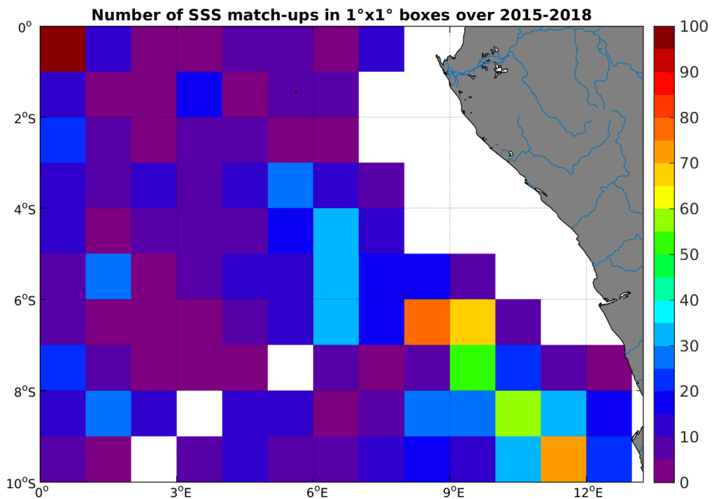
Figure 4: Number of SSS match-ups between Argo SSS and the SMAP-L3-RSS-V2-8DAY-RUNNING-40KM SSS product for the Congo river plume Pi-MEP region over 1^\circ \times 1^\circ boxes and for the full satellite product period.
