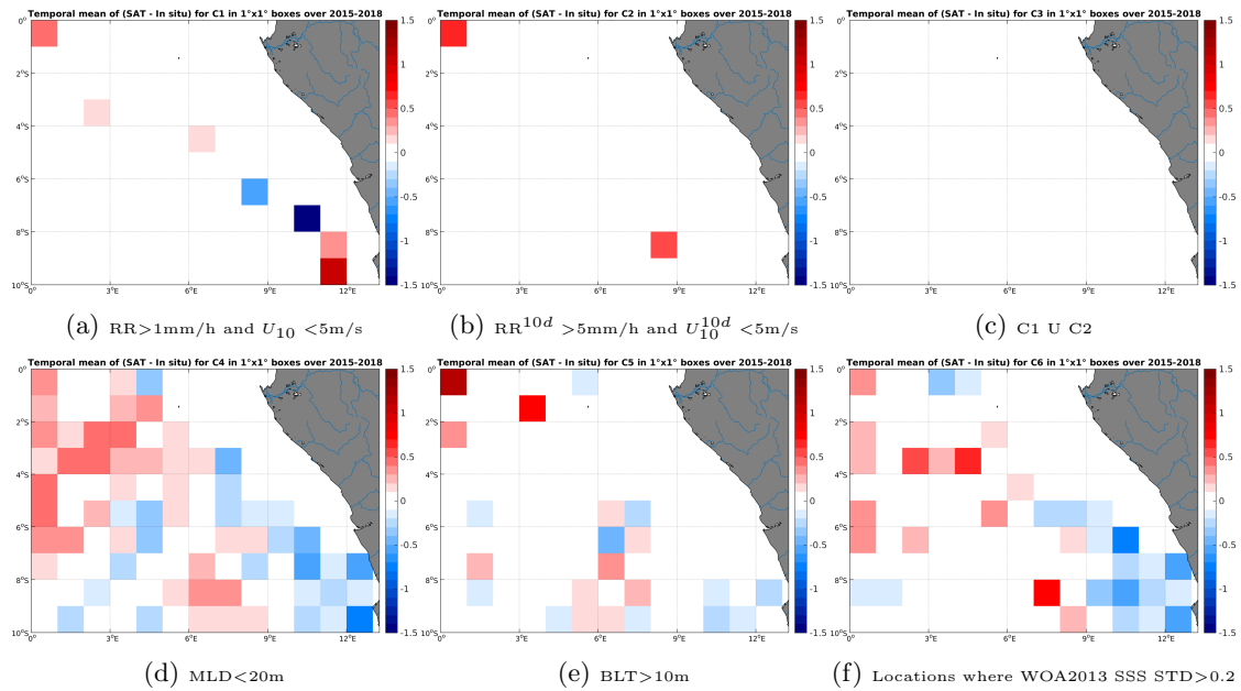
Figure 12: Temporal mean gridded over spatial boxes of size 1^\circ \times 1^\circ of \Delta SSS (SMAP-L3-RSS-V2-8DAY-RUNNING-40KM - Argo) for 6 different subdatasets corresponding to: RR > 1\text{mm/h} and U_{10} < 5\text{m/s} (a), RR^{10d} > 5\text{mm/h} and U_{10}^{10d} < 5\text{m/s} (b), C1 U C2 (c), MLD < 20\text{m} (d), BLT > 10\text{m} (e), Locations where WOA2013 SSS STD > 0.2 (f).
