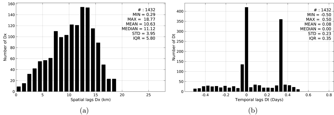
Figure 5: Histograms of the spatial (a) and temporal (b) lags between the time of the Argo measurements and the date of the corresponding SMAP-L3-RSS-V2-8DAY-RUNNING-40KM SSS product.
