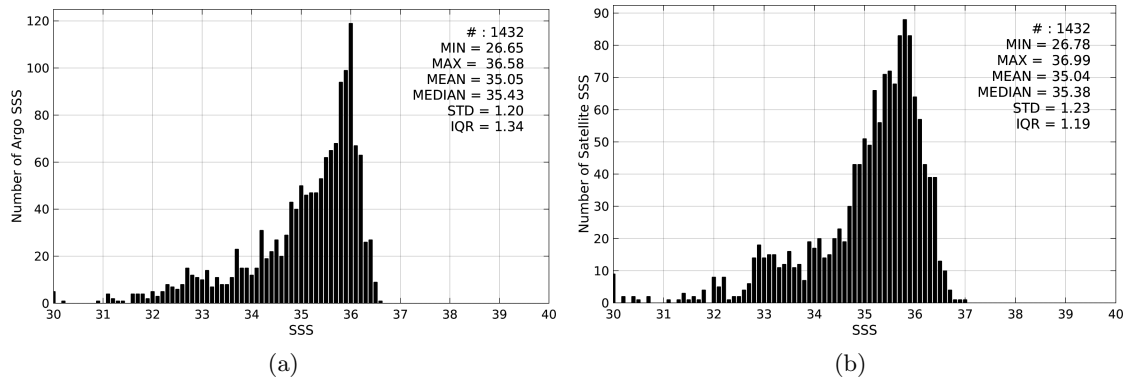
Figure 2: Histograms of SSS from Argo (a) and SMAP-L3-RSS-V2-8DAY-RUNNING-40KM (b) considering all match-up pairs per bins of 0.1 over the Congo river plume Pi-MEP region and for the full satellite product period.
