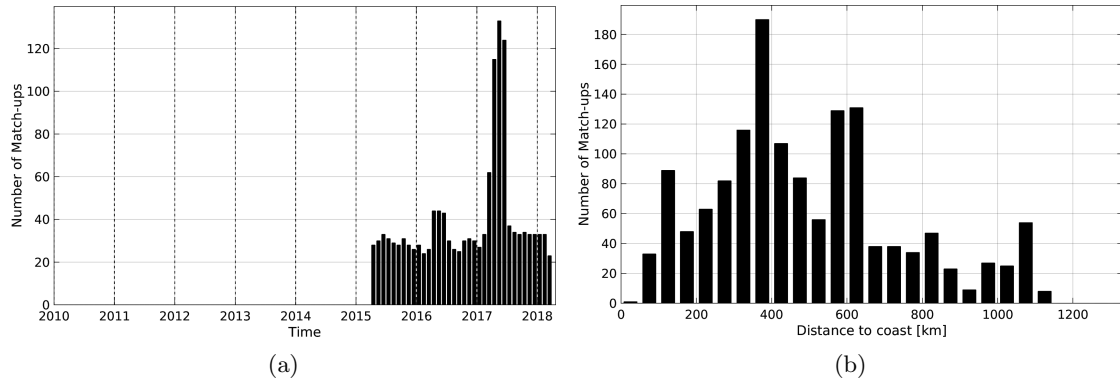
Figure 1: Number of match-ups between Argo and SMAP-L3-RSS-V2-8DAY-RUNNING-40KM SSS as a function of time (a) and as function of the distance to coast (b) over the Congo river plume Pi-MEP region and for the full satellite product period.
