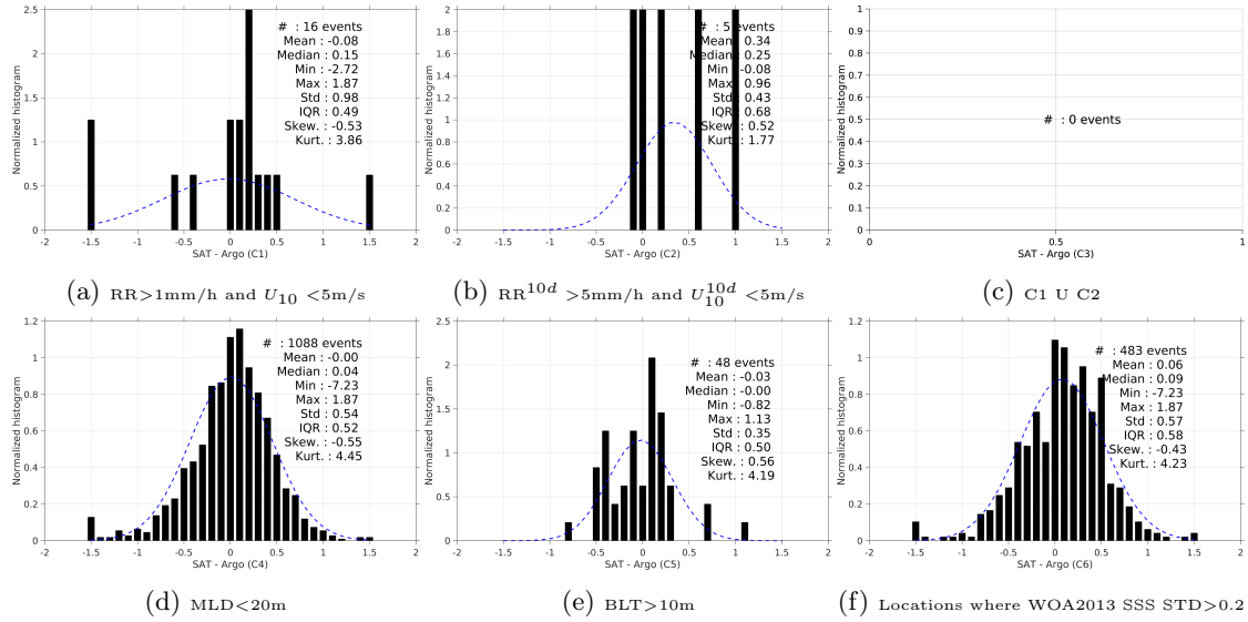
Figure 13: Normalized histogram of \Delta SSS (SMAP-L3-RSS-V2-8DAY-RUNNING-40KM - Argo) for 6 different subdatasets corresponding to: RR>1mm/h and U_{10} < 5\text{m/s} (a), RR^{10d} > 5\text{mm/h} and U_{10}^{10d} < 5\text{m/s} (b), C1 U C2 (c), MLD<20m (d), BLT>10m (e), Locations where WOA2013 SSS STD>0.2 (f).
