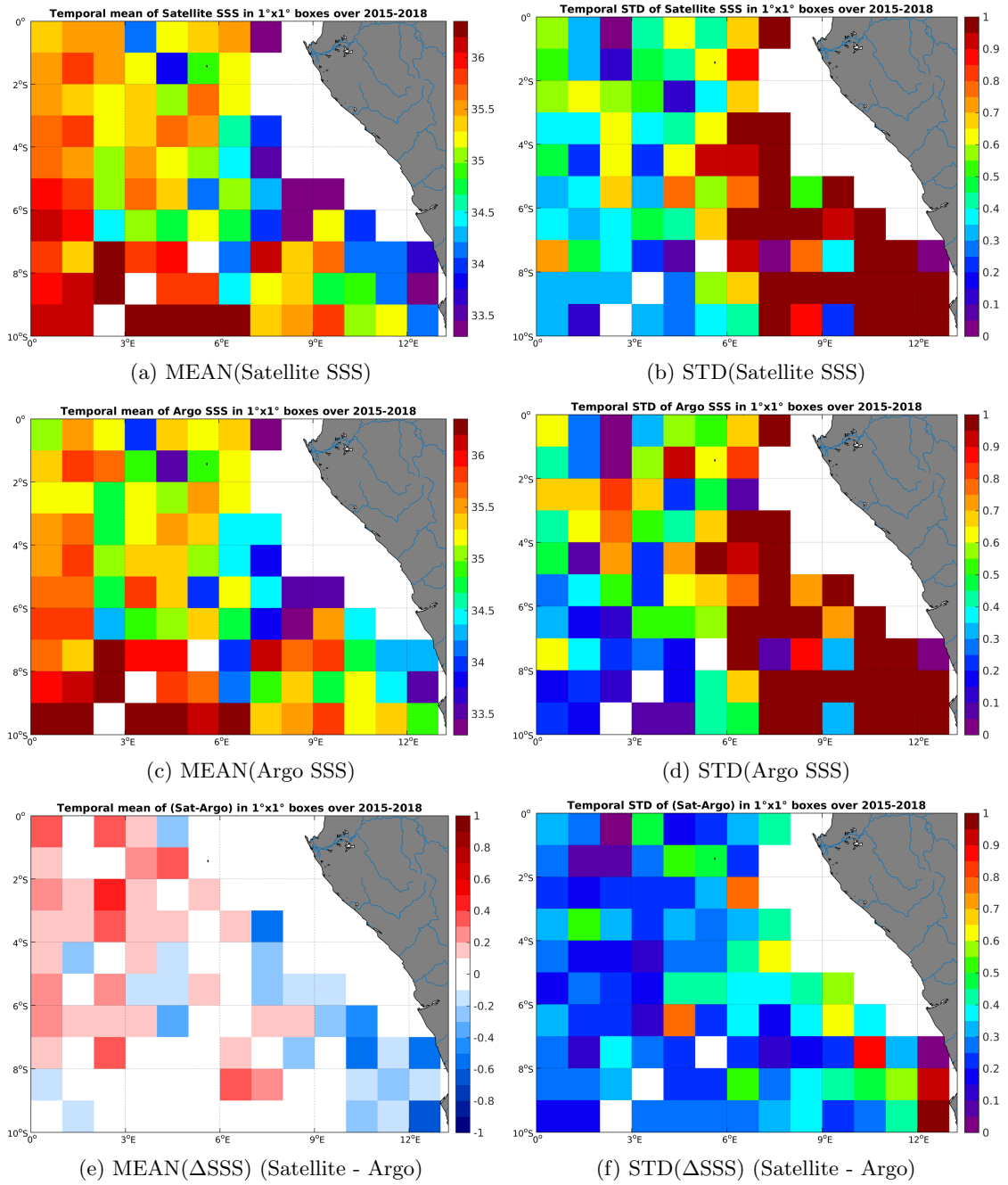
Figure 6: Temporal mean (left) and STD (right) of SSS from SMAP-L3-RSS-V2-8DAY-RUNNING-40KM (top), Argo (middle), and of \Delta SSS (Satellite - Argo). Only match-up pairs are used to generate these maps.
