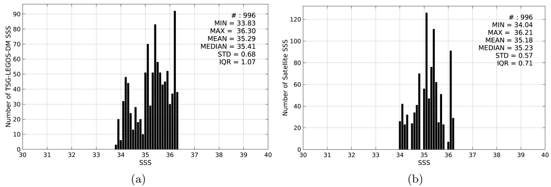
Figure 2: Histograms of SSS from TSG-LEGOS-DM (a) and SMAP-L3-RSS-V2-MONTHLY-0.25DEG-40KM (b) considering all match-up pairs per bins of 0.1 over the Congo river plume Pi-MEP region and for the full satellite product period.
