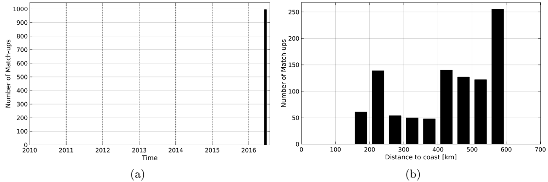
Figure 1: Number of match-ups between TSG-LEGOS-DM and SMAP-L3-RSS-V2-MONTHLY-0.25DEG-40KM SSS as a function of time (a) and as function of the distance to coast (b) over the Congo river plume Pi-MEP region and for the full satellite product period.
