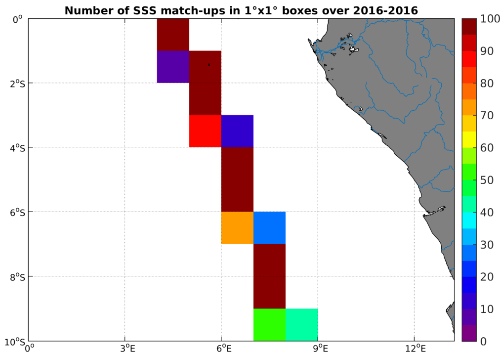
Figure 4: Number of SSS match-ups between TSG-LEGOS-DM SSS and the SMAP-L3-RSS-V2-MONTHLY-0.25DEG-40KM SSS product for the Congo river plume Pi-MEP region over 1°x1° boxes and for the full satellite product period.
