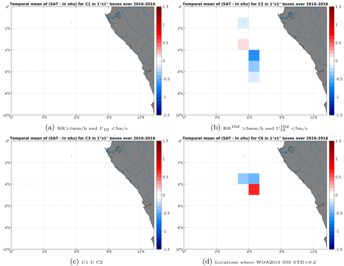
Figure 12: Temporal mean gridded over spatial boxes of size 1^\circ \times 1^\circ of \Delta SSS (SMAP-L3-RSS-V2-MONTHLY-0.25DEG-40KM - TSG-LEGOS-DM) for 4 different subdatasets corresponding to: RR > 1\text{mm/h} and U_{10} < 5\text{m/s} (a), RR^{10d} > 5\text{mm/h} and U_{10}^{10d} < 5\text{m/s} (b), C1 \cup C2 (c), Locations where WOA2013 SSS STD > 0.2 (d).
