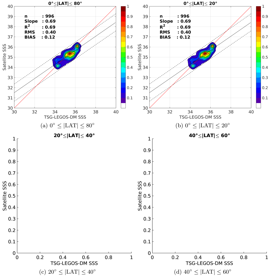
Figure 9: Contour maps of the concentration of SMAP-L3-RSS-V2-MONTHLY-0.25DEG-40KM SSS (y-axis) versus TSG-LEGOS-DM SSS (x-axis) at match-up pairs for different latitude bands. For each plot, the red line shows x=y . The black thin and dashed lines indicate a linear fit through the data cloud and the \pm 95\% confidence levels, respectively. The number match-up pairs n , the slope and R^2 coefficient of the linear fit, the root mean square (RMS) and the mean bias between satellite and in situ data are indicated for each latitude band in each plots.
