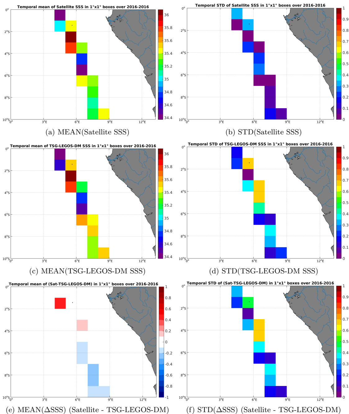
Figure 6: Temporal mean (left) and STD (right) of SSS from SMAP-L3-RSS-V2-MONTHLY-0.25DEG-40KM (top), TSG-LEGOS-DM (middle), and of \Delta SSS (Satellite - TSG-LEGOS-DM). Only match-up pairs are used to generate these maps.
