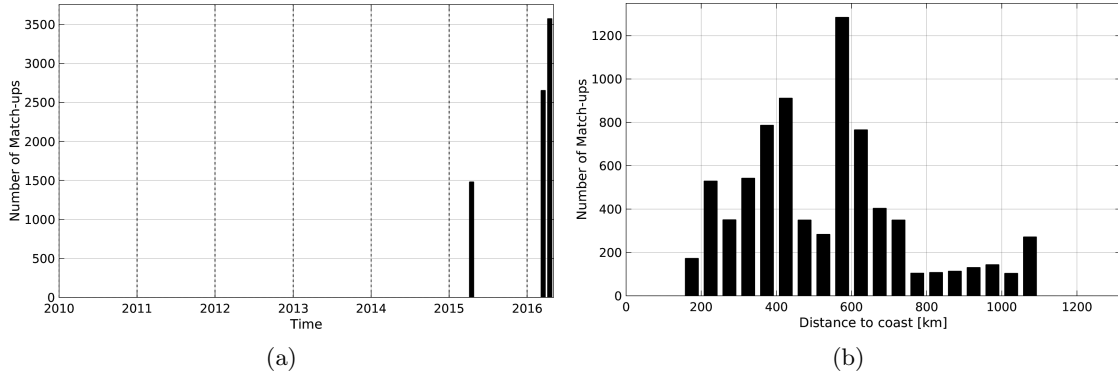
Figure 1: Number of match-ups between TSG-GOSUD-Research-vessel and SMAP-L3-RSS-V2-MONTHLY-0.25DEG-40KM SSS as a function of time (a) and as function of the distance to coast (b) over the Congo river plume Pi-MEP region and for the full satellite product period.
