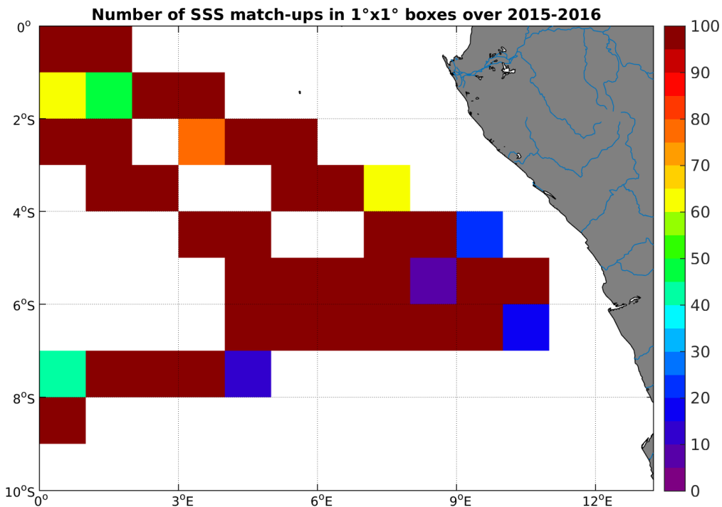
Figure 4: Number of SSS match-ups between TSG-GOSUD-Research-vessel SSS and the SMAP-L3-RSS-V2-MONTHLY-0.25DEG-40KM SSS product for the Congo river plume Pi-MEP region over 1°x1° boxes and for the full satellite product period.
