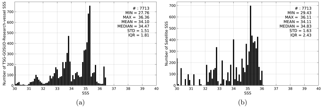
Figure 2: Histograms of SSS from TSG-GOSUD-Research-vessel (a) and SMAP-L3-RSS-V2-MONTHLY-0.25DEG-40KM (b) considering all match-up pairs per bins of 0.1 over the Congo river plume Pi-MEP region and for the full satellite product period.
