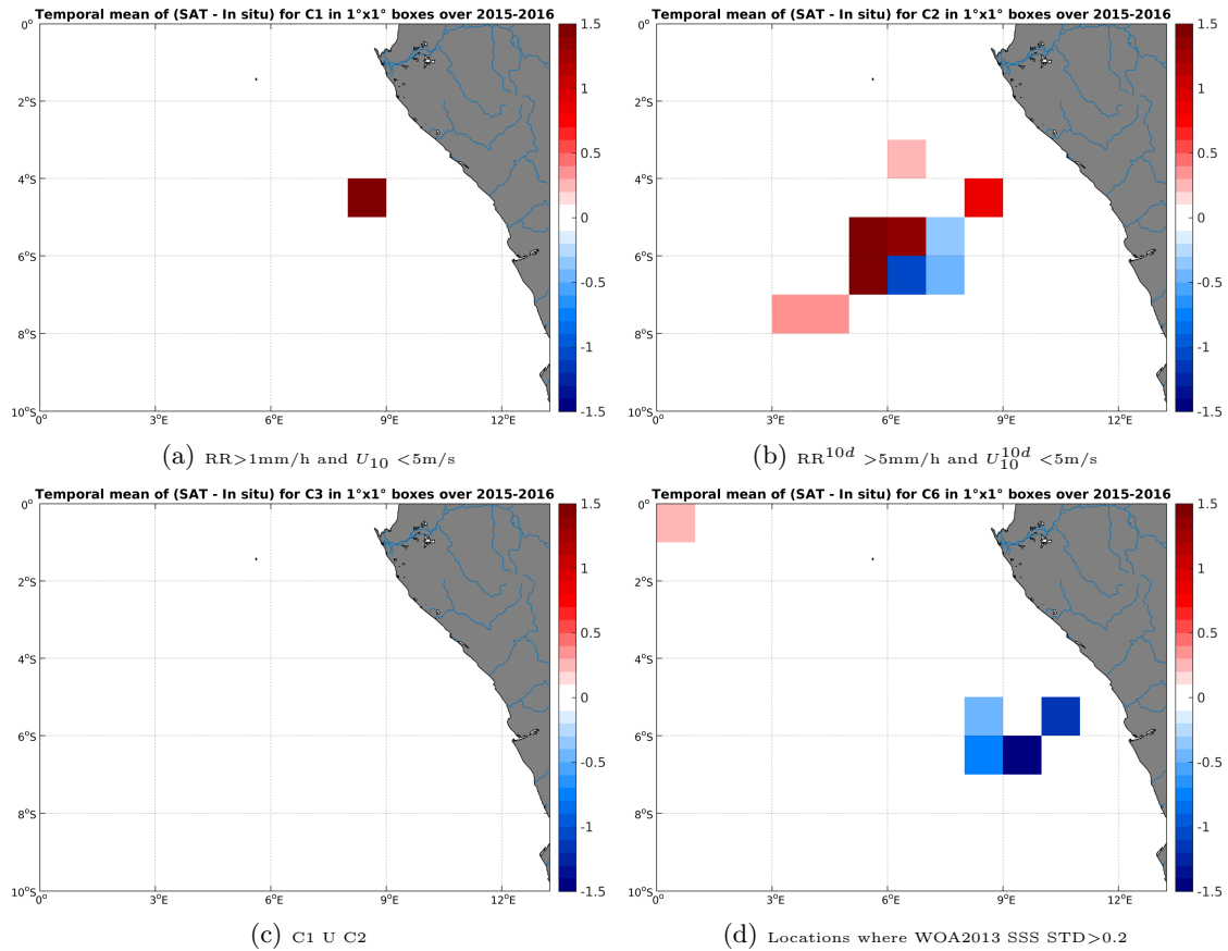
Figure 12: Temporal mean gridded over spatial boxes of size 1°x1° of \Delta SSS (SMAP-L3-RSS-V2-MONTHLY-0.25DEG-40KM - TSG-GOSUD-Research-vessel) for 4 different subdatasets corresponding to:RR>1mm/h and U_{10} < 5m/s (a), RR^{10d} > 5mm/h and U_{10}^{10d} < 5m/s (b), C1 U C2 (c),Locations where WOA2013 SSS STD>0.2 (d).
