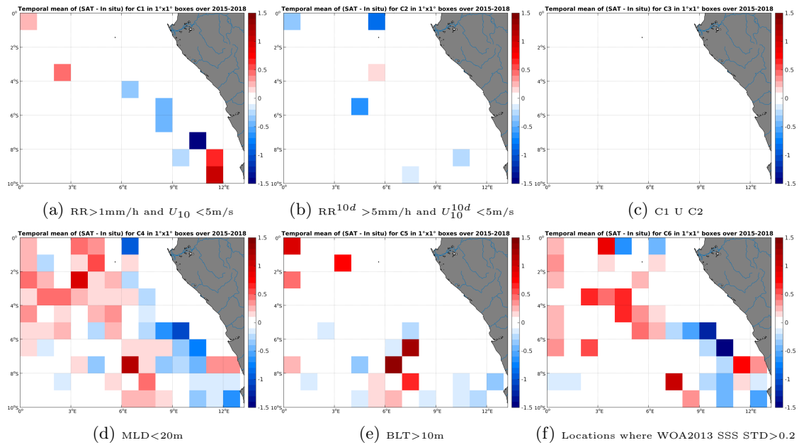
Figure 12: Temporal mean gridded over spatial boxes of size 1^\circ \times 1^\circ of \Delta SSS (SMAP-L3-RSS-V2-MONTHLY-0.25DEG-40KM - Argo) for 6 different subdatasets corresponding to:RR > 1 mm/h and U_{10} < 5 m/s (a), RR^{10d} > 5 mm/h and U_{10}^{10d} < 5 m/s (b), C1 U C2 (c),MLD < 20 m (d),BLT > 10 m (e),Locations where WOA2013 SSS STD > 0.2 (f).
