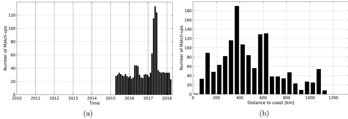
Figure 1: Number of match-ups between Argo and SMAP-L3-RSS-V2-MONTHLY-0.25DEG-40KM SSS as a function of time (a) and as function of the distance to coast (b) over the Congo river plume Pi-MEP region and for the full satellite product period.
