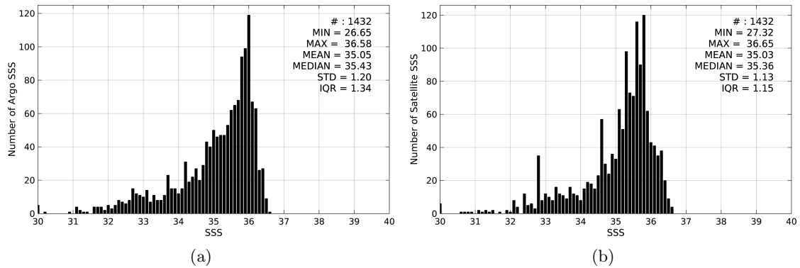
Figure 2: Histograms of SSS from Argo (a) and SMAP-L3-RSS-V2-MONTHLY-0.25DEG-40KM (b) considering all match-up pairs per bins of 0.1 over the Congo river plume Pi-MEP region and for the full satellite product period.
