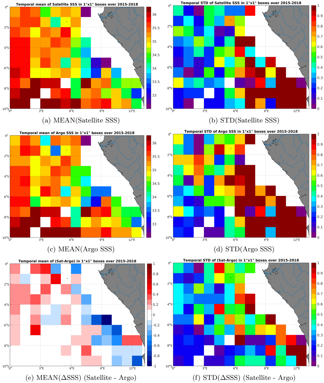
Figure 6: Temporal mean (left) and STD (right) of SSS from SMAP-L3-RSS-V2-MONTHLY-0.25DEG-40KM (top), Argo (middle), and of \Delta SSS (Satellite - Argo). Only match-up pairs are used to generate these maps.
