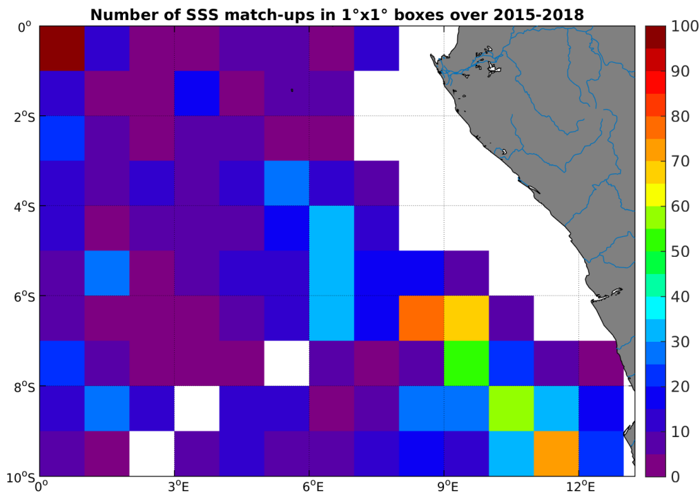
Figure 4: Number of SSS match-ups between Argo SSS and the SMAP-L3-RSS-V2-MONTHLY-0.25DEG-40KM SSS product for the Congo river plume Pi-MEP region over 1^\circ \times 1^\circ boxes and for the full satellite product period.
