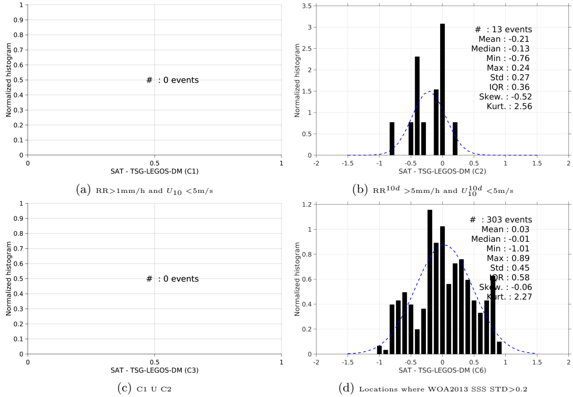
Figure 13: Normalized histogram of \Delta\text{SSS} (SMAP-L3-RSS-V2-MONTHLY-70KM - TSG-LEGOS-DM) for 6 different subdatasets corresponding to: RR > 1\text{mm/h} and U_{10} < 5\text{m/s} (a), RR^{10d} > 5\text{mm/h} and U_{10}^{10d} < 5\text{m/s} (b), C1 \cup C2 (c), Locations where WOA2013 SSS STD > 0.2 (d).
