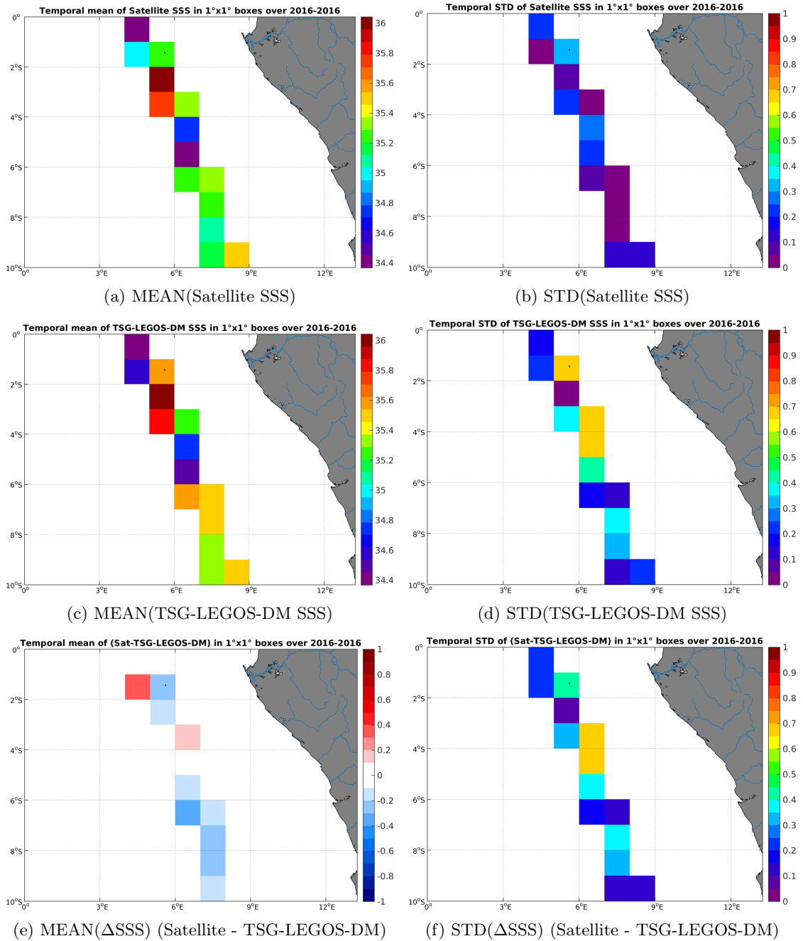
Figure 6: Temporal mean (left) and STD (right) of SSS from SMAP-L3-RSS-V2-MONTHLY-70KM (top), TSG-LEGOS-DM (middle), and of \Delta SSS (Satellite - TSG-LEGOS-DM). Only match-up pairs are used to generate these maps.
