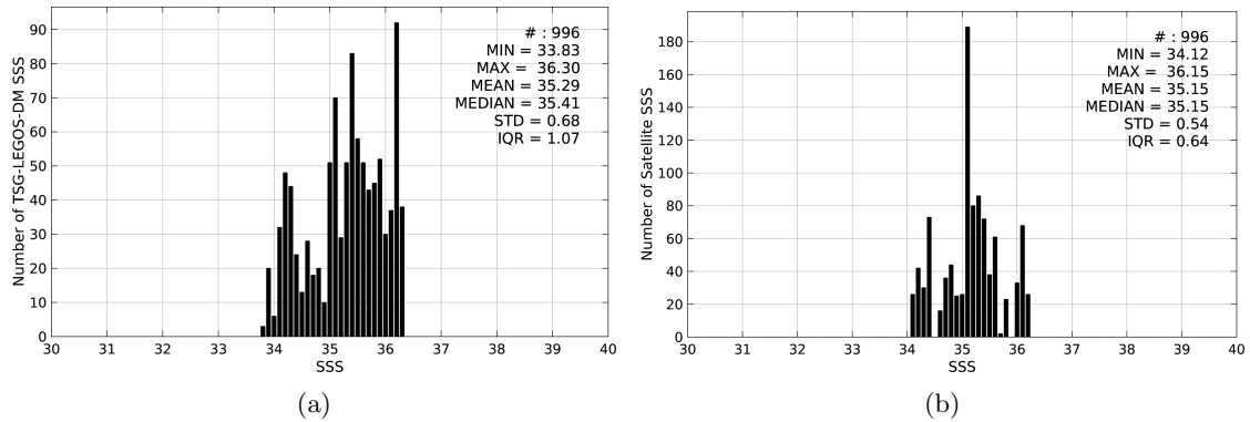
Figure 2: Histograms of SSS from TSG-LEGOS-DM (a) and SMAP-L3-RSS-V2-MONTHLY-70KM (b) considering all match-up pairs per bins of 0.1 over the Congo river plume Pi-MEP region and for the full satellite product period.
