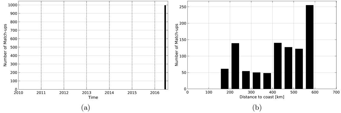
Figure 1: Number of match-ups between TSG-LEGOS-DM and SMAP-L3-RSS-V2-MONTHLY-70KM SSS as a function of time (a) and as function of the distance to coast (b) over the Congo river plume Pi-MEP region and for the full satellite product period.
