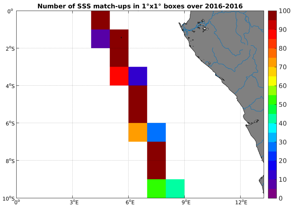
Figure 4: Number of SSS match-ups between TSG-LEGOS-DM SSS and the SMAP-L3-RSS-V2-MONTHLY-70KM SSS product for the Congo river plume Pi-MEP region over 1°x1° boxes and for the full satellite product period.
