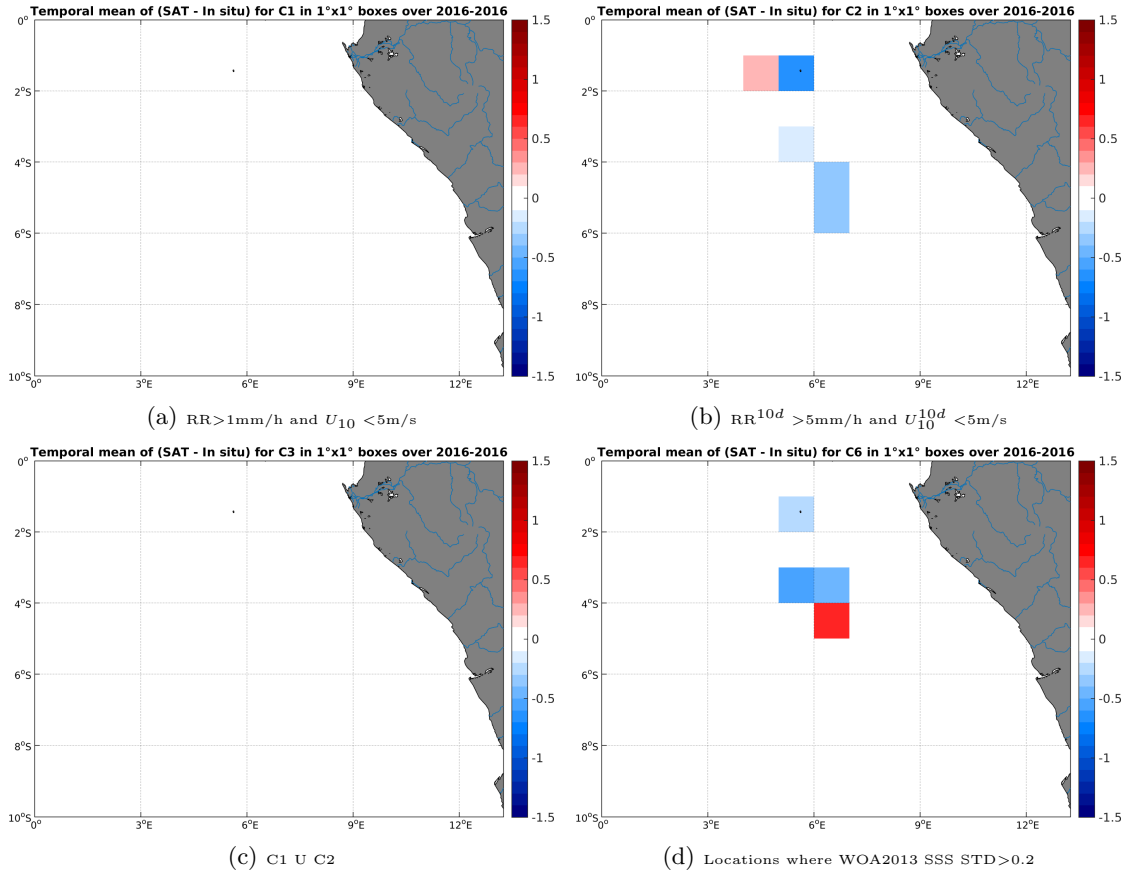
Figure 12: Temporal mean gridded over spatial boxes of size 1^\circ \times 1^\circ of \Delta SSS (SMAP-L3-RSS-V2-MONTHLY-70KM - TSG-LEGOS-DM) for 4 different subdatasets corresponding to:RR>1mm/h and U_{10} < 5\text{m/s} (a), RR^{10d} > 5\text{mm/h} and U_{10}^{10d} < 5\text{m/s} (b), C1 U C2 (c),Locations where WOA2013 SSS STD>0.2 (d).
