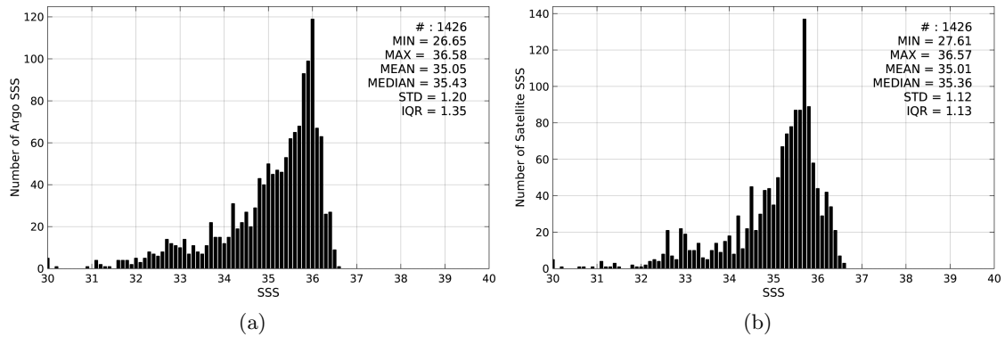
Figure 2: Histograms of SSS from Argo (a) and SMAP-L3-RSS-V2-MONTHLY-70KM (b) considering all match-up pairs per bins of 0.1 over the Congo river plume Pi-MEP region and for the full satellite product period.
