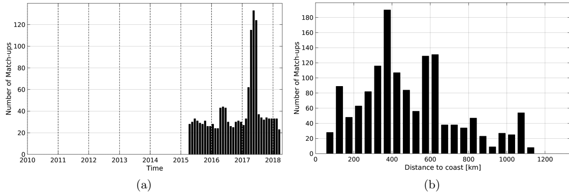
Figure 1: Number of match-ups between Argo and SMAP-L3-RSS-V2-MONTHLY-70KM SSS as a function of time (a) and as function of the distance to coast (b) over the Congo river plume Pi-MEP region and for the full satellite product period.
