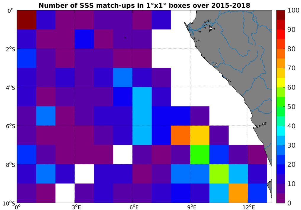
Figure 4: Number of SSS match-ups between Argos SSS and the SMAP-L3-RSS-V2-MONTHLY-70KM SSS product for the Congo river plume Pi-MEP region over 1^{\circ} \times 1^{\circ} boxes and for the full satellite product period.
