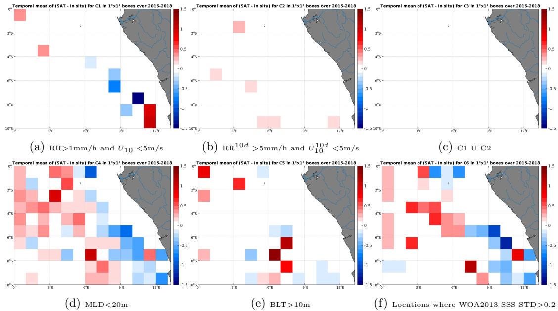
Figure 12: Temporal mean gridded over spatial boxes of size 1^\circ \times 1^\circ of \Delta SSS (SMAP-L3-RSS-V2-MONTHLY-70KM - Argo) for 6 different subdatasets corresponding to:RR >1 mm/h and U_{10} < 5 m/s (a), RR^{10d} > 5 mm/h and U_{10}^{10d} < 5 m/s (b), C1 U C2 (c),MLD <20 m (d),BLT >10 m (e),Locations where WOA2013 SSS STD >0.2 (f).
