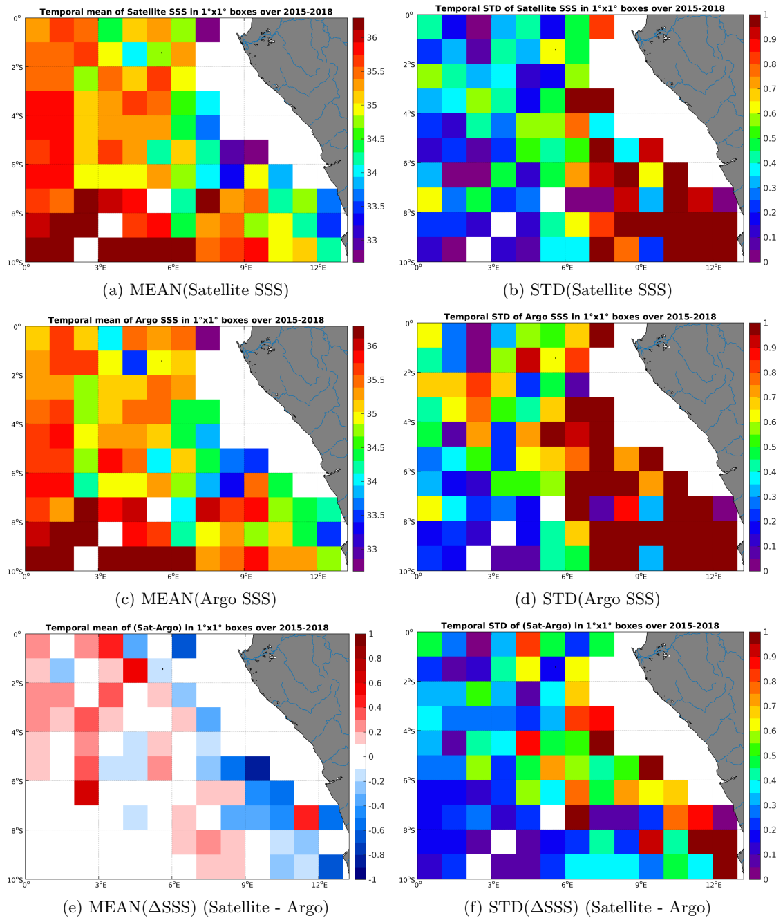
Figure 6: Temporal mean (left) and STD (right) of SSS from SMAP-L3-RSS-V2-MONTHLY-70KM (top), Argo (middle), and of \Delta SSS (Satellite - Argo). Only match-up pairs are used to generate these maps.
