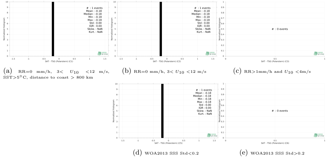
Figure 13: Normalized histogram of \Delta\text{SSS} (SMAP SSS L3 v5.0 - 8-Day running (JPL) - TSG (Polarstern)) for 5 different subdatasets corresponding to: RR=0 mm/h, 3 < U_{10} < 12 m/s, SST > 5^\circ\text{C} , distance to coast > 800 km (a), RR=0 mm/h, 3 < U_{10} < 12 m/s (b), RR > 1\text{mm/h} and U_{10} < 4\text{m/s} (c), WOA2013 SSS Std < 0.2 (d), WOA2013 SSS Std > 0.2 (e).
