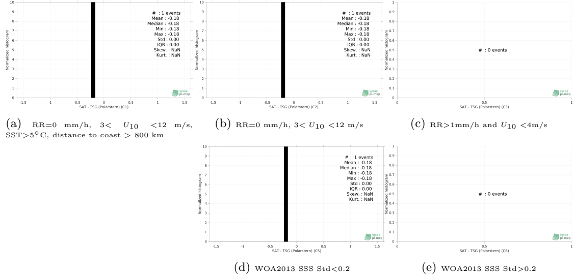
Figure 13: Normalized histogram of \Delta SSS (SMAP SSS L3 v5.0 - 8-Day running (JPL) - TSG (Polarstern)) for 5 different subdatasets corresponding to: RR=0 mm/h, 3 < U_{10} < 12 m/s, SST >5^{\circ} C, distance to coast > 800 km (a), RR=0 mm/h, 3 < U_{10} < 12 m/s (b), RR >1 mm/h and U_{10} < 4 m/s (c), WOA2013 SSS Std <0.2 (d), WOA2013 SSS Std >0.2 (e).
