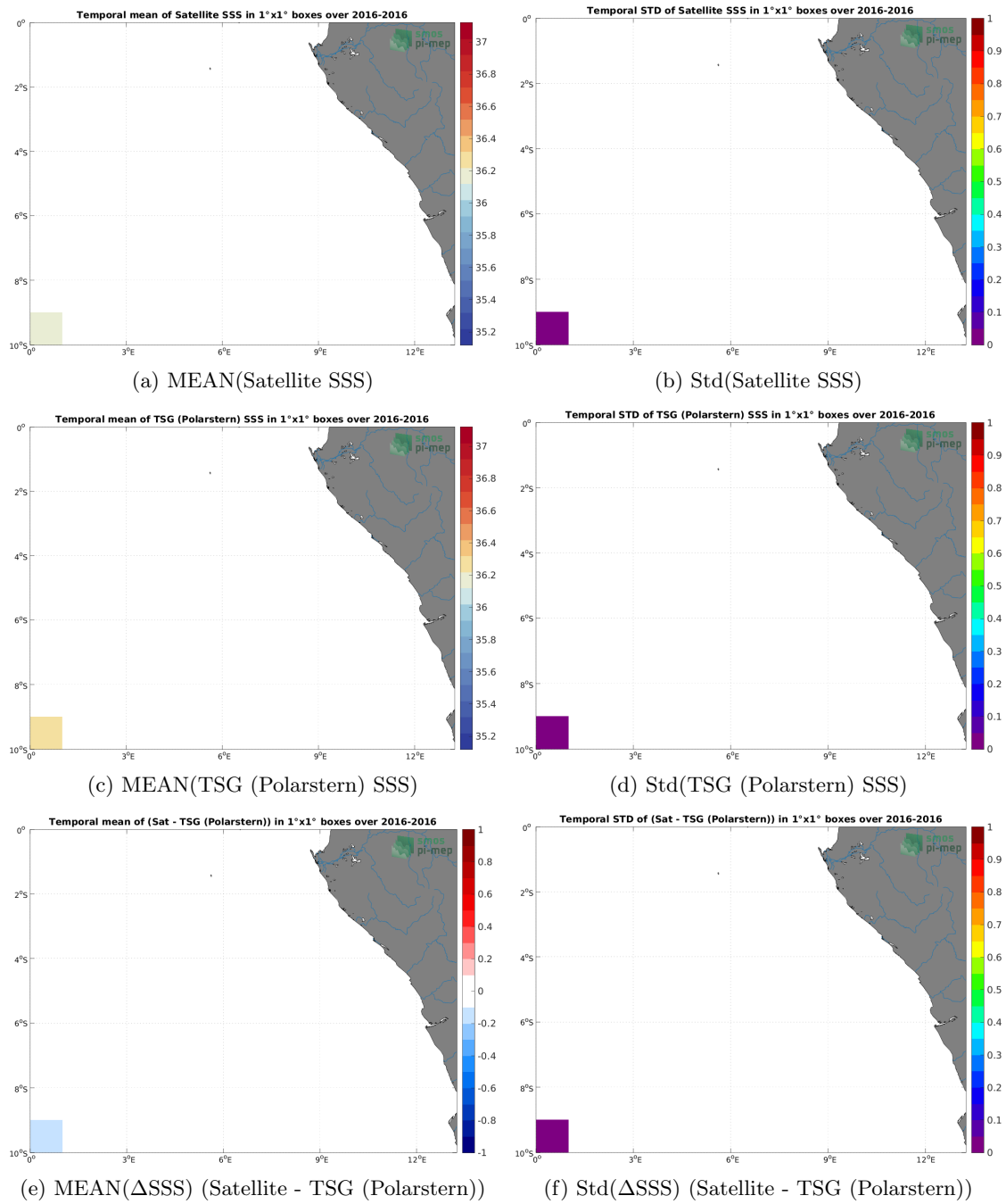
Figure 6: Temporal mean (left) and Std (right) of SSS from SMAP SSS L3 v5.0 - 8-Day running (JPL) (top), TSG (Polarstern) (middle), and of \Delta SSS (Satellite - TSG (Polarstern)). Only match-up pairs are used to generate these maps.
