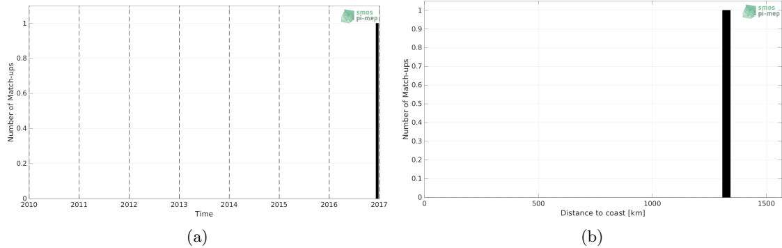
Figure 1: Number of match-ups between TSG (Polarstern) and SMAP SSS L3 v5.0 - 8-Day running (JPL) SSS as a function of time (a) and as function of the distance to coast (b) over the Congo river plume Pi-MEP region and for the full satellite product period.
