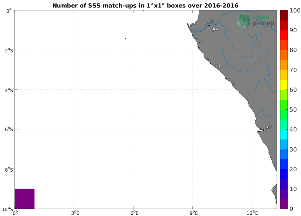
Figure 4: Number of SSS match-ups between TSG (Polarstern) SSS and the SMAP SSS L3 v5.0 - 8-Day running (JPL) SSS product for the Congo river plume Pi-MEP region over 1^\circ \times 1^\circ boxes and for the full satellite product period.
