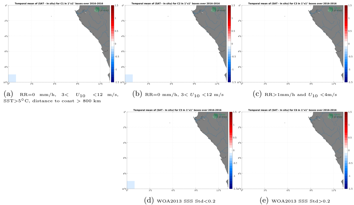
Figure 12: Temporal mean gridded over spatial boxes of size 1^{\circ}\times 1^{\circ} of \Delta\text{SSS} (SMAP SSS L3 v5.0 - 8-Day running (JPL) - TSG (Polarstern)) for 5 different subdatasets corresponding to:RR=0 mm/h, 3 < U_{10} < 12 m/s, SST >5^{\circ}\text{C} , distance to coast > 800 km (a), RR=0 mm/h, 3 < U_{10} < 12 m/s (b), RR >1 mm/h and U_{10} < 4 m/s (c), WOA2013 SSS Std <0.2 (d), WOA2013 SSS Std >0.2 (e).
