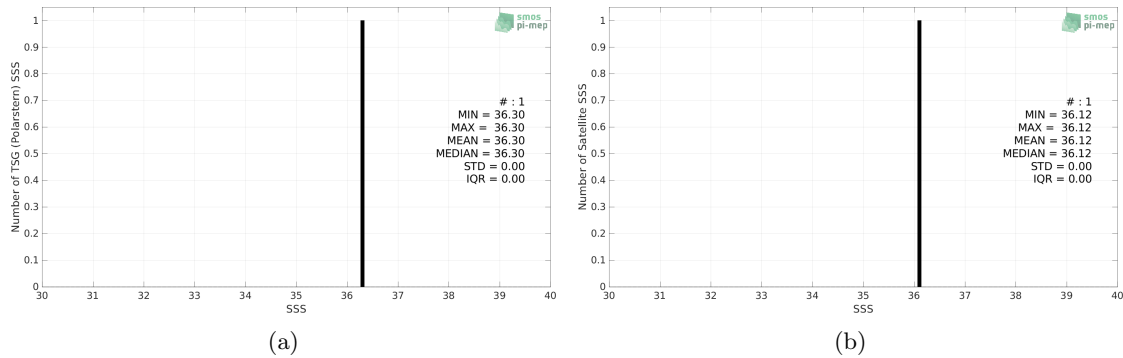
Figure 2: Histograms of SSS from TSG (Polarstern) (a) and SMAP SSS L3 v5.0 - 8-Day running (JPL) (b) considering all match-up pairs per bins of 0.1 over the Congo river plume Pi-MEP region and for the full satellite product period.
