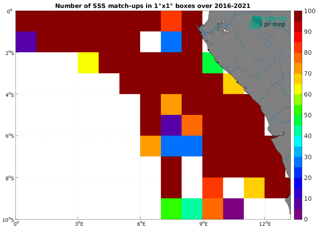
Figure 5: Number of SSS match-ups between TSG (LEGOS-DM) SSS and the SMAP SSS L3 v5.0 - 8-Day running (JPL) SSS product for the Congo river plume Pi-MEP region over 1^\circ \times 1^\circ boxes and for the full satellite product period.
