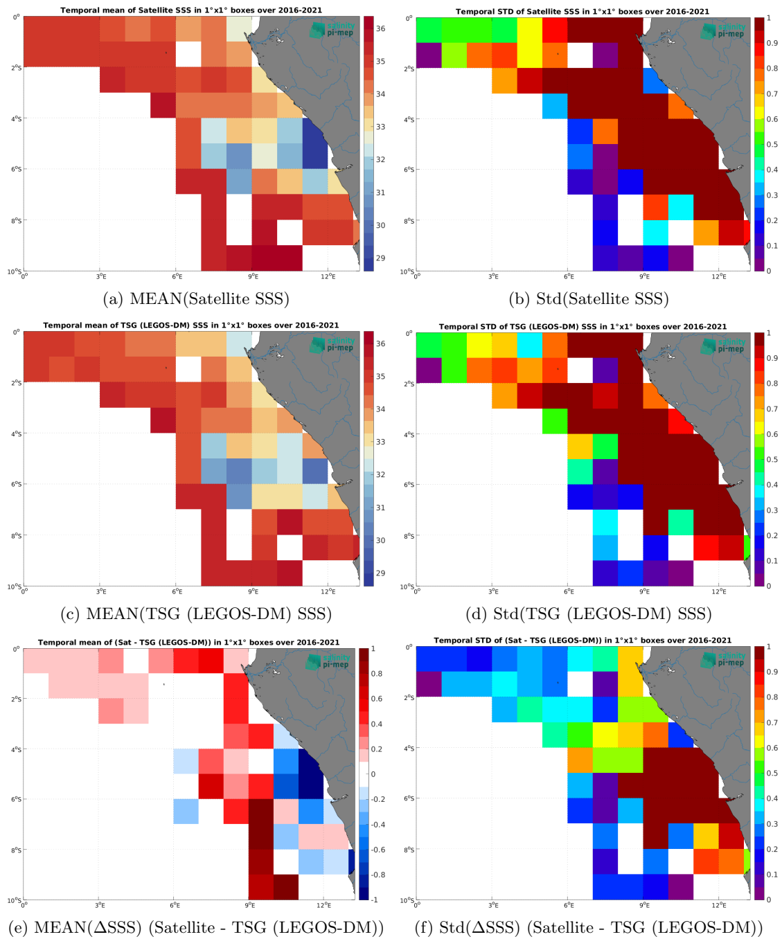
Figure 7: Temporal mean (left) and Std (right) of SSS from SMAP SSS L3 v5.0 - 8-Day running (JPL) (top), TSG (LEGOS-DM) (middle), and of \Delta SSS (Satellite - TSG (LEGOS-DM)). Only match-up pairs are used to generate these maps.
