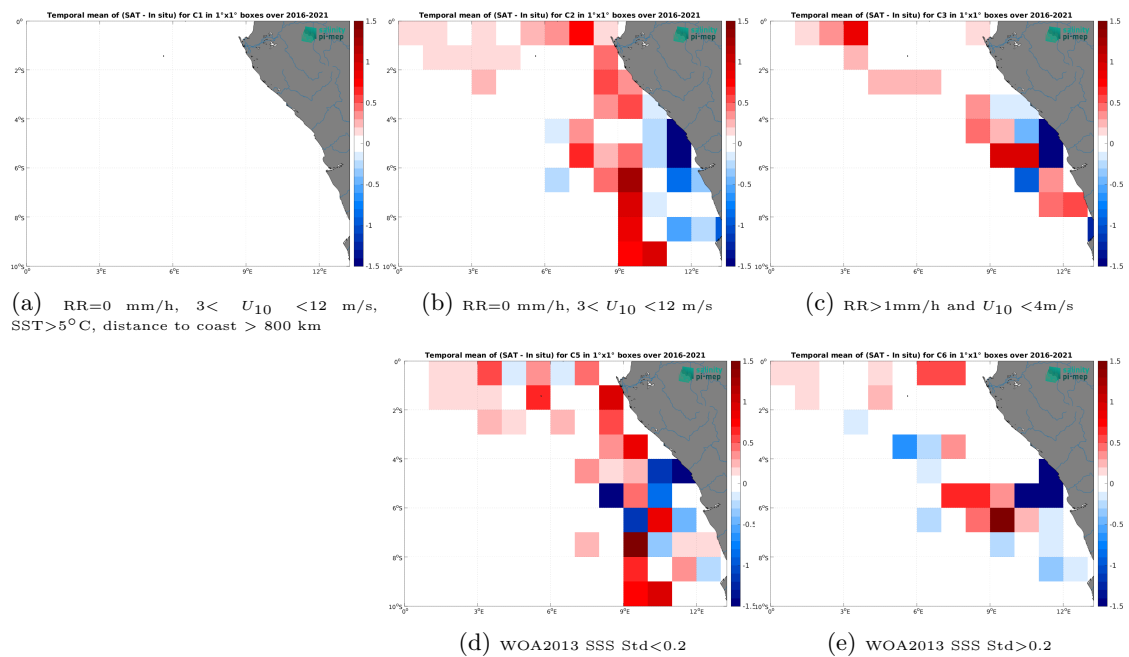
Figure 14: Temporal mean gridded over spatial boxes of size 1^\circ \times 1^\circ of \Delta SSS (SMAP SSS L3 v5.0 - 8-Day running (JPL) - TSG (LEGOS-DM)) for 5 different subdatasets corresponding to: RR=0 mm/h, 3 < U_{10} < 12 m/s, SST > 5°C, distance to coast > 800 km (a), RR=0 mm/h, 3 < U_{10} < 12 m/s (b), RR > 1 mm/h and U_{10} < 4 m/s (c), WOA2013 SSS Std < 0.2 (d), WOA2013 SSS Std > 0.2 (e).
