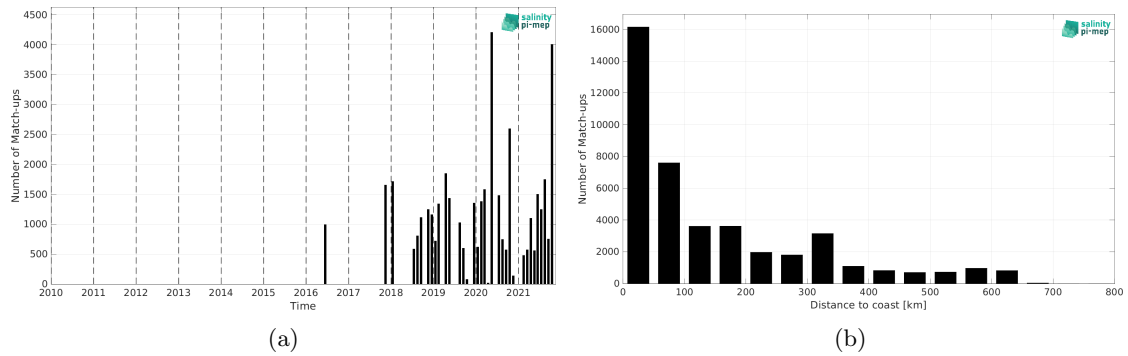
Figure 2: Number of match-ups between TSG (LEGOS-DM) and SMAP SSS L3 v5.0 - 8-Day running (JPL) SSS as a function of time (a) and as function of the distance to coast (b) over the Congo river plume Pi-MEP region and for the full satellite product period.
