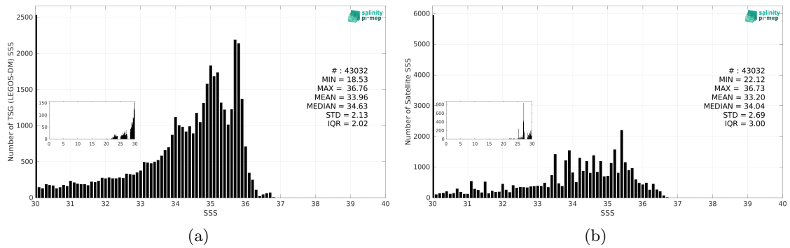
Figure 3: Histograms of SSS from TSG (LEGOS-DM) (a) and SMAP SSS L3 v5.0 - 8-Day running (JPL) (b) considering all match-up pairs per bins of 0.1 over the Congo river plume Pi-MEP region and for the full satellite product period.
