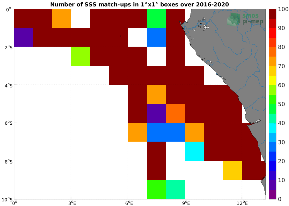
Figure 4: Number of SSS match-ups between TSG (LEGOS-DM) SSS and the SMAP SSS L3 v5.0 - 8-Day running (JPL) SSS product for the Congo river plume Pi-MEP region over 1^{\circ} \times 1^{\circ} boxes and for the full satellite product period.
