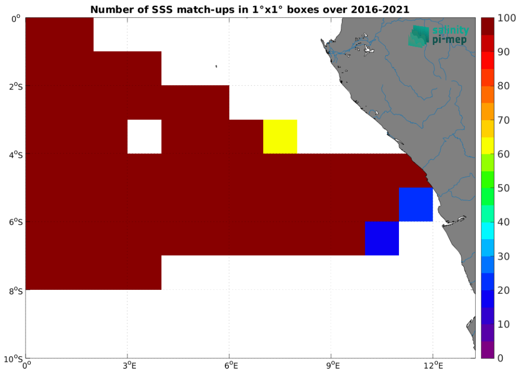
Figure 5: Number of SSS match-ups between TSG (GOSUD-Research-vessel) SSS and the SMAP SSS L3 v5.0 - 8-Day running (JPL) SSS product for the Congo river plume Pi-MEP region over 1^\circ \times 1^\circ boxes and for the full satellite product period.
