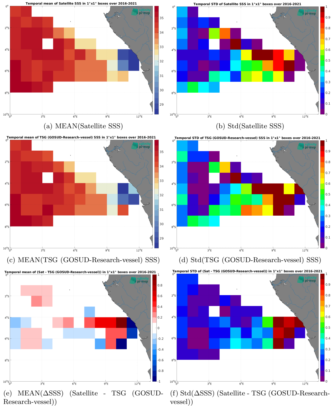
Figure 7: Temporal mean (left) and Std (right) of SSS from SMAP SSS L3 v5.0 - 8-Day running (JPL) (top), TSG (GOSUD-Research-vessel) (middle), and of \Delta SSS (Satellite - TSG (GOSUD-Research-vessel)). Only match-up pairs are used to generate these maps.
