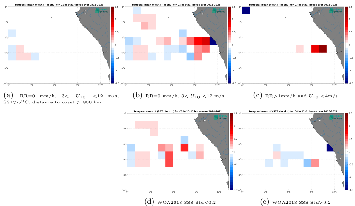
Figure 14: Temporal mean gridded over spatial boxes of size 1^\circ \times 1^\circ of \Delta SSS (SMAP SSS L3 v5.0 - 8-Day running (JPL) - TSG (GOSUD-Research-vessel)) for 5 different subdatasets corresponding to:RR=0 mm/h, 3 < U_{10} < 12 m/s, SST>5°C, distance to coast > 800 km (a), RR=0 mm/h, 3 < U_{10} < 12 m/s (b), RR>1mm/h and U_{10} < 4 m/s (c), WOA2013 SSS Std<0.2 (d), WOA2013 SSS Std>0.2 (e).
