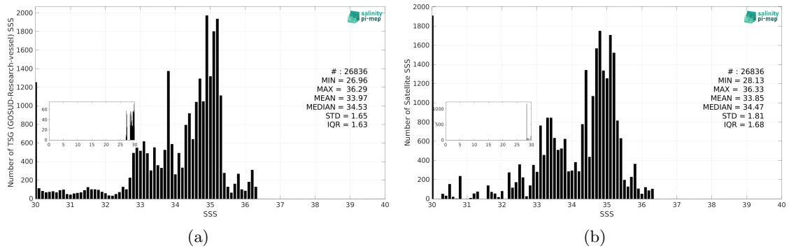
Figure 3: Histograms of SSS from TSG (GOSUD-Research-vessel) (a) and SMAP SSS L3 v5.0 - 8-Day running (JPL) (b) considering all match-up pairs per bins of 0.1 over the Congo river plume Pi-MEP region and for the full satellite product period.
