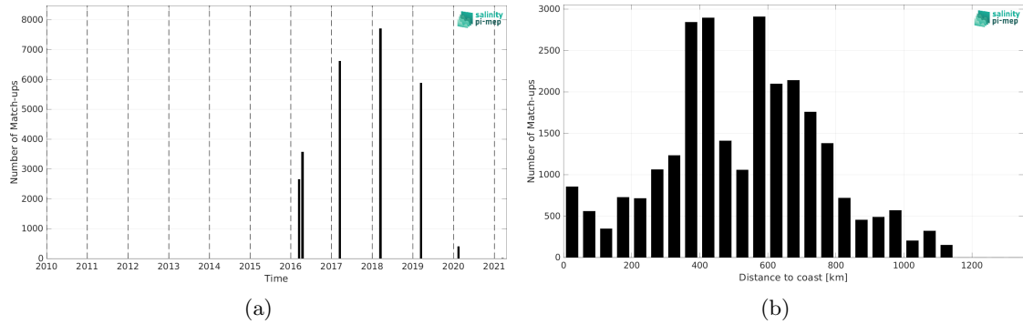
Figure 2: Number of match-ups between TSG (GOSUD-Research-vessel) and SMAP SSS L3 v5.0 - 8-Day running (JPL) SSS as a function of time (a) and as function of the distance to coast (b) over the Congo river plume Pi-MEP region and for the full satellite product period.
