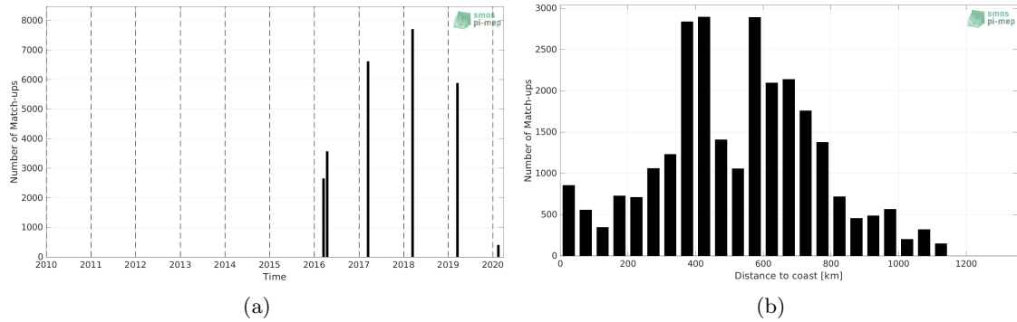
Figure 1: Number of match-ups between TSG (GOSUD-Research-vessel) and SMAP SSS L3 v5.0 - 8-Day running (JPL) SSS as a function of time (a) and as function of the distance to coast (b) over the Congo river plume Pi-MEP region and for the full satellite product period.
