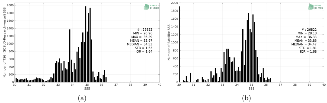
Figure 2: Histograms of SSS from TSG (GOSUD-Research-vessel) (a) and SMAP SSS L3 v5.0 - 8-Day running (JPL) (b) considering all match-up pairs per bins of 0.1 over the Congo river plume Pi-MEP region and for the full satellite product period.
