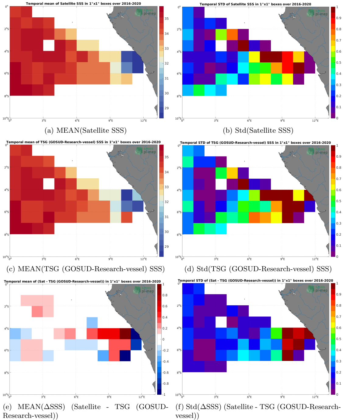
Figure 6: Temporal mean (left) and Std (right) of SSS from SMAP SSS L3 v5.0 - 8-Day running (JPL) (top), TSG (GOSUD-Research-vessel) (middle), and of \Delta SSS (Satellite - TSG (GOSUD-Research-vessel)). Only match-up pairs are used to generate these maps.
