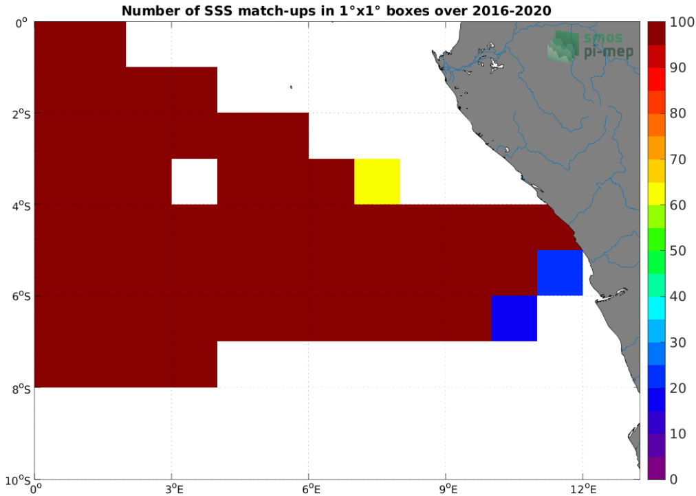
Figure 4: Number of SSS match-ups between TSG (GOSUD-Research-vessel) SSS and the SMAP SSS L3 v5.0 - 8-Day running (JPL) SSS product for the Congo river plume Pi-MEP region over 1^\circ \times 1^\circ boxes and for the full satellite product period.
