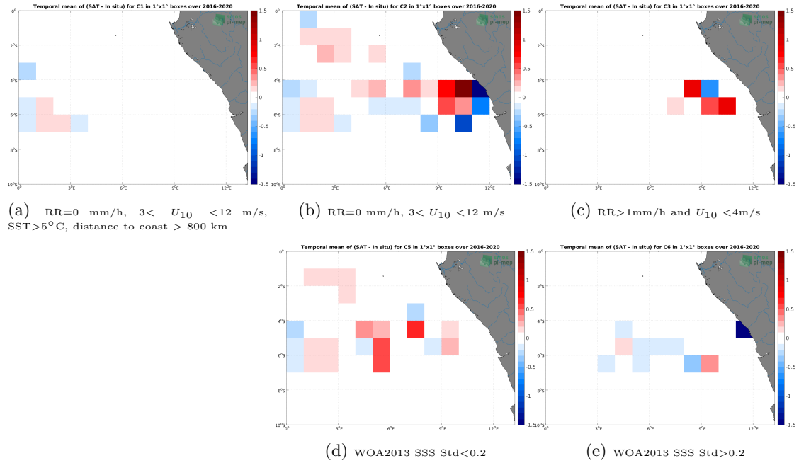
Figure 12: Temporal mean gridded over spatial boxes of size 1^{\circ}\times 1^{\circ} of \Delta SSS (SMAP SSS L3 v5.0 - 8-Day running (JPL) - TSG (GOSUD-Research-vessel)) for 5 different subdatasets corresponding to:RR=0 mm/h, 3 < U_{10} < 12 m/s, SST >5^{\circ}\text{C} , distance to coast > 800 km (a), RR=0 mm/h, 3 < U_{10} < 12 m/s (b), RR >1 mm/h and U_{10} < 4 m/s (c), WOA2013 SSS Std <0.2 (d), WOA2013 SSS Std >0.2 (e).
