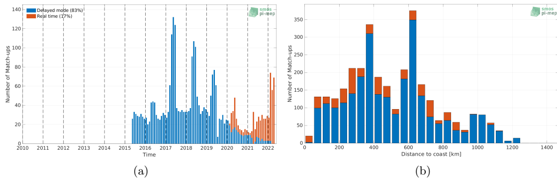
Figure 1: Number of match-ups between Argo and SMAP SSS L3 v5.0 - 8-Day running (JPL) SSS as a function of time (a) and as function of the distance to coast (b) over the Congo river plume Pi-MEP region and for the full satellite product period.
