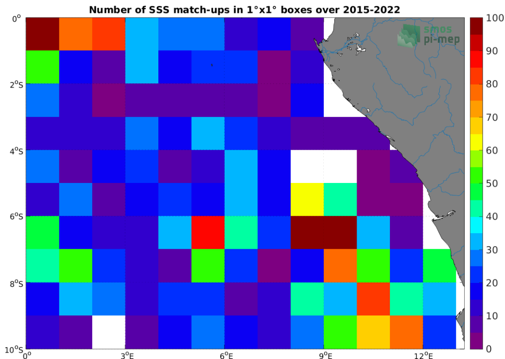
Figure 4: Number of SSS match-ups between Argo SSS and the SMAP SSS L3 v5.0 - 8-Day running (JPL) SSS product for the Congo river plume Pi-MEP region over 1^\circ \times 1^\circ boxes and for the full satellite product period.
