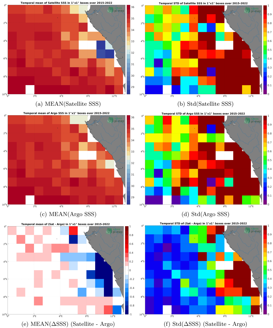
Figure 6: Temporal mean (left) and Std (right) of SSS from SMAP SSS L3 v5.0 - 8-Day running (JPL) (top), Argo (middle), and of \Delta SSS (Satellite - Argo). Only match-up pairs are used to generate these maps.
