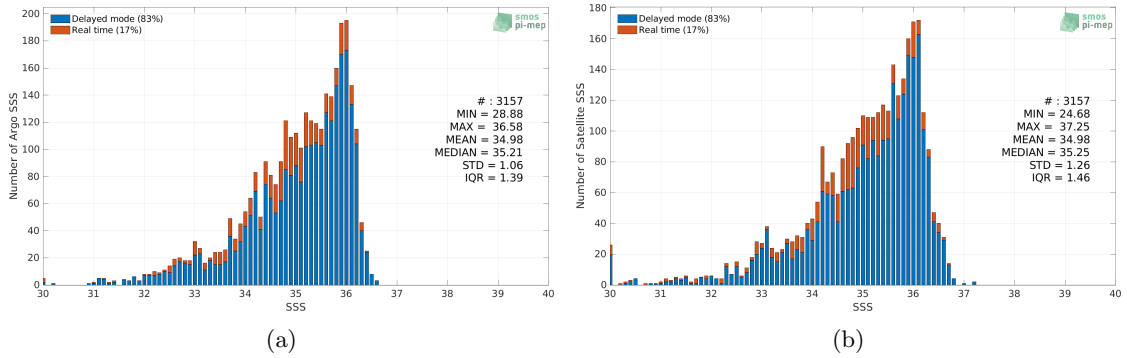
Figure 2: Histograms of SSS from Argo (a) and SMAP SSS L3 v5.0 - 8-Day running (JPL) (b) considering all match-up pairs per bins of 0.1 over the Congo river plume Pi-MEP region and for the full satellite product period.
