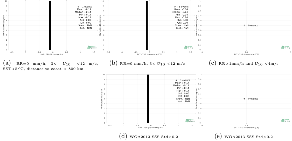
Figure 13: Normalized histogram of \Delta SSS (SMAP SSS L3 v5.0 - Monthly (JPL) - TSG (Polarstern)) for 5 different subdatasets corresponding to: RR=0 mm/h, 3 < U_{10} < 12 m/s, SST >5^{\circ} C, distance to coast > 800 km (a), RR=0 mm/h, 3 < U_{10} < 12 m/s (b), RR >1 mm/h and U_{10} < 4 m/s (c), WOA2013 SSS Std <0.2 (d), WOA2013 SSS Std >0.2 (e).
