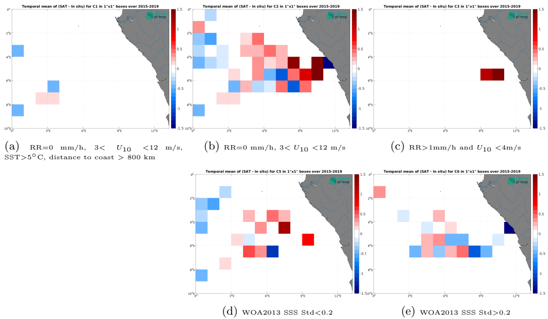
Figure 14: Temporal mean gridded over spatial boxes of size 1^\circ \times 1^\circ of \Delta SSS (SMAP SSS L3 v5.0 - Monthly (JPL) - TSG (GOSUD-Research-vessel)) for 5 different subdatasets corresponding to:RR=0 mm/h, 3 < U_{10} < 12 m/s, SST>5°C, distance to coast > 800 km (a), RR=0 mm/h, 3 < U_{10} < 12 m/s (b), RR>1mm/h and U_{10} < 4 m/s (c), WOA2013 SSS Std<0.2 (d), WOA2013 SSS Std>0.2 (e).
