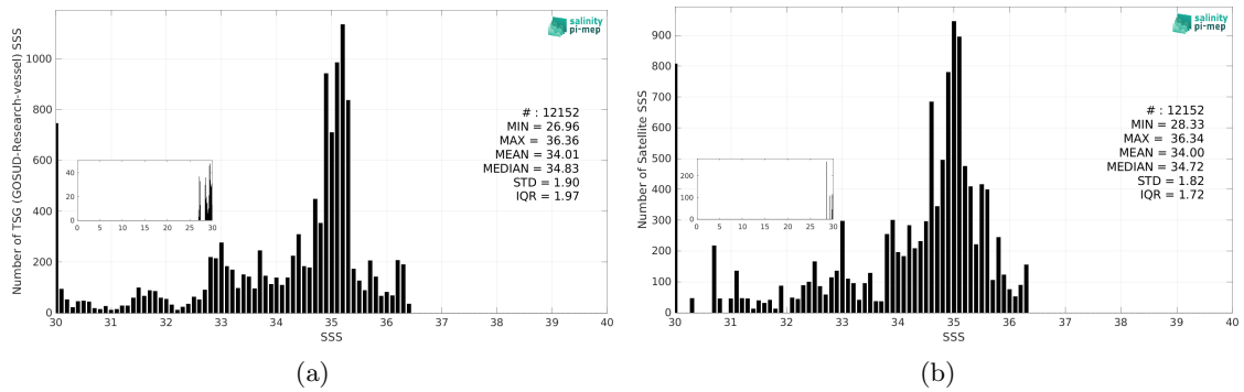
Figure 3: Histograms of SSS from TSG (GOSUD-Research-vessel) (a) and SMAP SSS L3 v5.0 - Monthly (JPL) (b) considering all match-up pairs per bins of 0.1 over the Congo river plume Pi-MEP region and for the full satellite product period.
