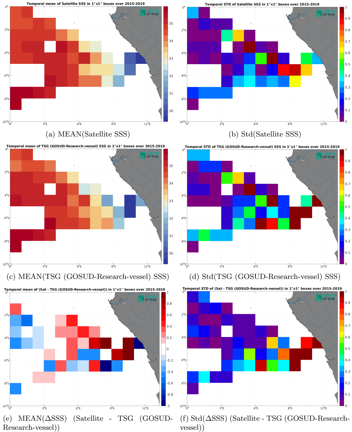
Figure 7: Temporal mean (left) and Std (right) of SSS from SMAP SSS L3 v5.0 - Monthly (JPL) (top), TSG (GOSUD-Research-vessel) (middle), and of \Delta SSS (Satellite - TSG (GOSUD-Research-vessel)). Only match-up pairs are used to generate these maps.
