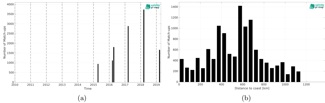
Figure 2: Number of match-ups between TSG (GOSUD-Research-vessel) and SMAP SSS L3 v5.0 - Monthly (JPL) SSS as a function of time (a) and as function of the distance to coast (b) over the Congo river plume Pi-MEP region and for the full satellite product period.
