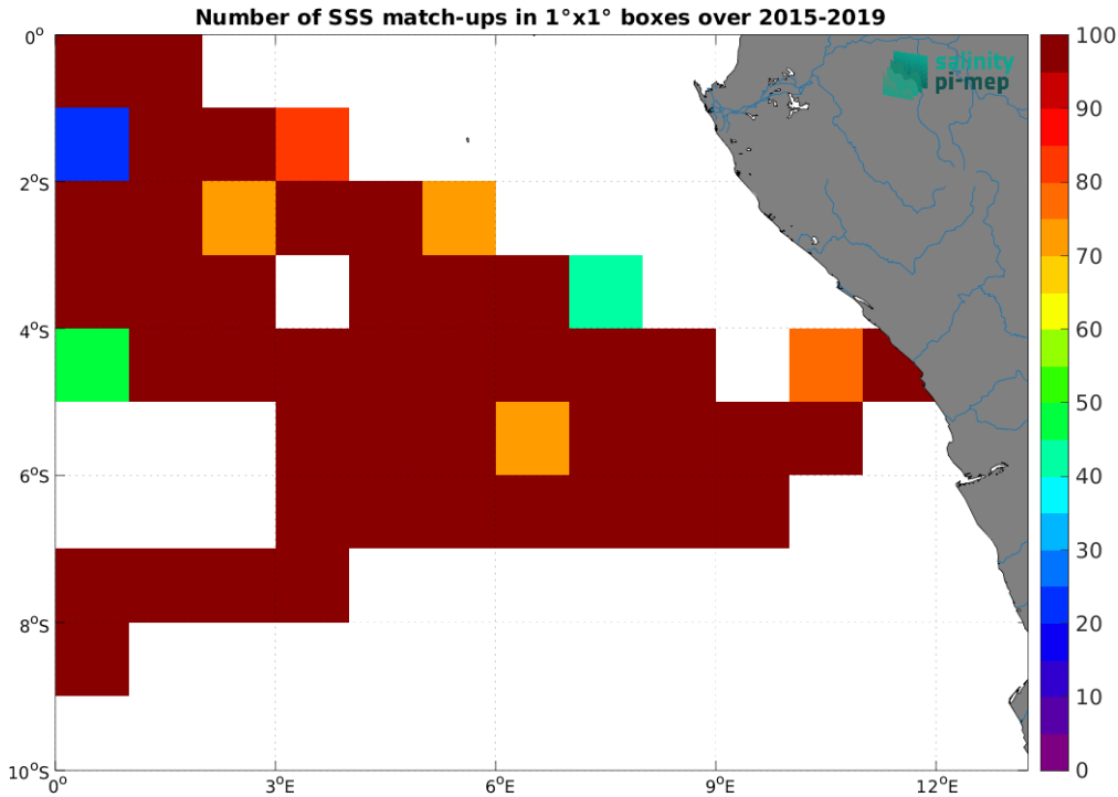
Figure 5: Number of SSS match-ups between TSG (GOSUD-Research-vessel) SSS and the SMAP SSS L3 v5.0 - Monthly (JPL) SSS product for the Congo river plume Pi-MEP region over 1^\circ \times 1^\circ boxes and for the full satellite product period.
