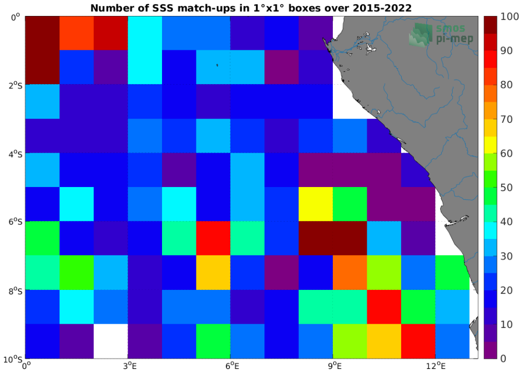
Figure 4: Number of SSS match-ups between Argo SSS and the SMAP SSS L3 v5.0 - Monthly (JPL) SSS product for the Congo river plume Pi-MEP region over 1^{\circ} \times 1^{\circ} boxes and for the full satellite product period.
