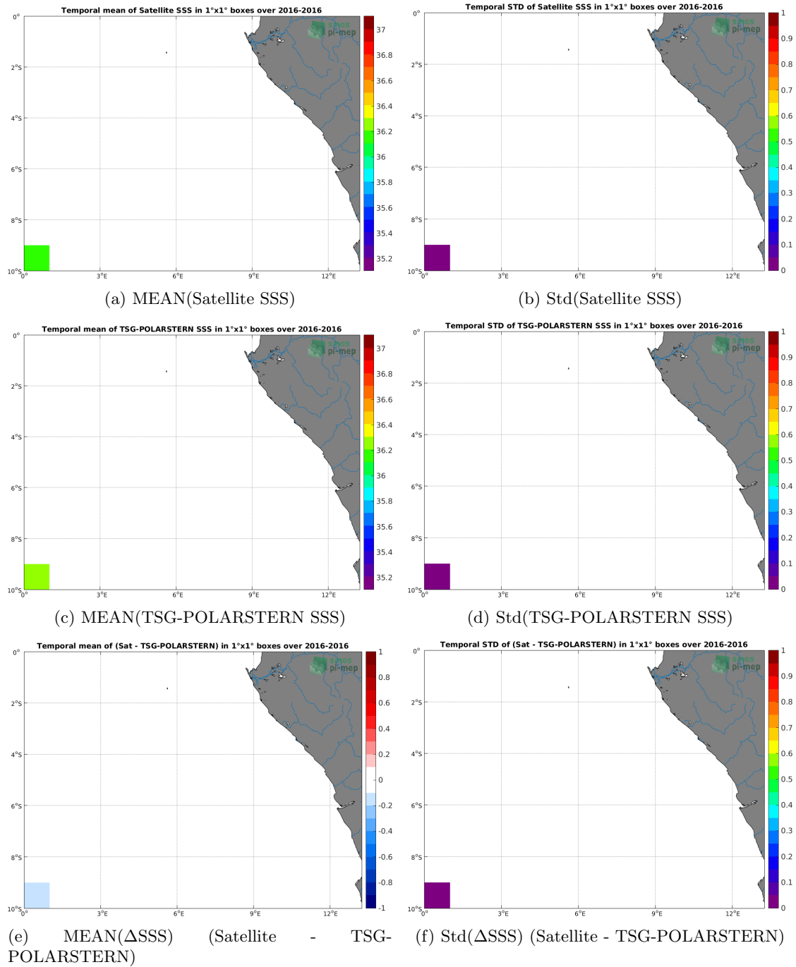
Figure 6: Temporal mean (left) and Std (right) of SSS from SMAP-L3-JPL-V4.3-8DAY-RUNNING-60KM (top), TSG-POLARSTERN (middle), and of \Delta SSS (Satellite - TSG-POLARSTERN). Only match-up pairs are used to generate these maps.
