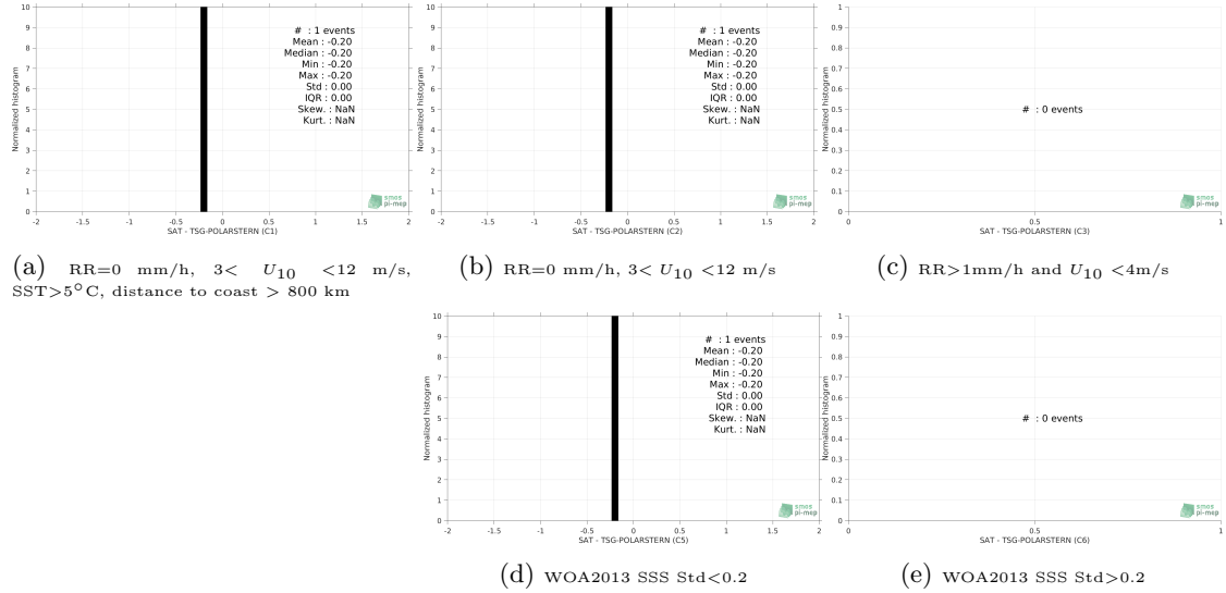
Figure 13: Normalized histogram of \Delta\text{SSS} (SMAP-L3-JPL-V4.3-8DAY-RUNNING-60KM - TSG-POLARSTERN) for 5 different subdatasets corresponding to: RR=0 mm/h, 3 < U_{10} < 12 m/s, SST > 5^\circ\text{C} , distance to coast > 800 km (a), RR=0 mm/h, 3 < U_{10} < 12 m/s (b), RR > 1\text{mm/h} and U_{10} < 4\text{m/s} (c), WOA2013 SSS Std < 0.2 (d), WOA2013 SSS Std > 0.2 (e).
