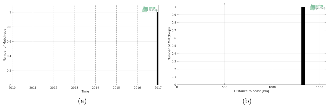
Figure 1: Number of match-ups between TSG-POLARSTERN and SMAP-L3-JPL-V4.3-8DAY-RUNNING-60KM SSS as a function of time (a) and as function of the distance to coast (b) over the Congo river plume Pi-MEP region and for the full satellite product period.
