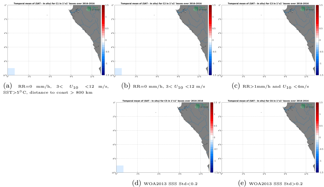
Figure 12: Temporal mean gridded over spatial boxes of size 1^\circ \times 1^\circ of \Delta SSS (SMAP-L3-JPL-V4.3-8DAY-RUNNING-60KM - TSG-POLARSTERN) for 5 different subdatasets corresponding to:RR=0 mm/h, 3 < U_{10} < 12 m/s, SST > 5^\circ\text{C} , distance to coast > 800 km (a), RR=0 mm/h, 3 < U_{10} < 12 m/s (b), RR > 1 mm/h and U_{10} < 4 m/s (c), WOA2013 SSS Std < 0.2 (d), WOA2013 SSS Std > 0.2 (e).
