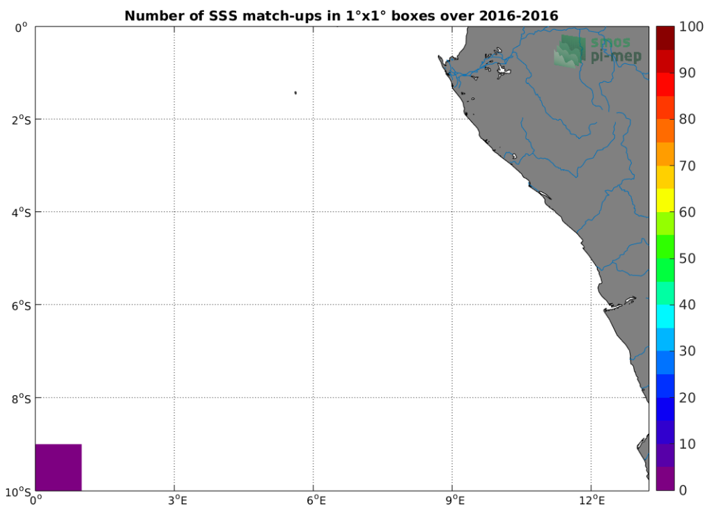
Figure 4: Number of SSS match-ups between TSG-POLARSTERN SSS and the SMAP-L3-JPL-V4.3-8DAY-RUNNING-60KM SSS product for the Congo river plume Pi-MEP region over 1°x1° boxes and for the full satellite product period.
