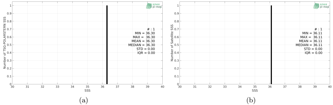
Figure 2: Histograms of SSS from TSG-POLARSTERN (a) and SMAP-L3-JPL-V4.3-8DAY-RUNNING-60KM (b) considering all match-up pairs per bins of 0.1 over the Congo river plume Pi-MEP region and for the full satellite product period.
