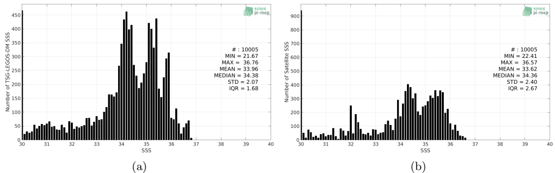
Figure 2: Histograms of SSS from TSG-LEGOS-DM (a) and SMAP-L3-JPL-V4.3-8DAY-RUNNING-60KM (b) considering all match-up pairs per bins of 0.1 over the Congo river plume Pi-MEP region and for the full satellite product period.
