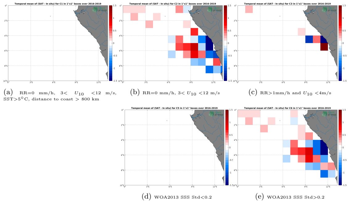
Figure 12: Temporal mean gridded over spatial boxes of size 1^\circ \times 1^\circ of \Delta SSS (SMAP-L3-JPL-V4.3-8DAY-RUNNING-60KM - TSG-LEGOS-DM) for 5 different subdatasets corresponding to:RR=0 mm/h, 3 < U_{10} < 12 m/s, SST >5^\circ C, distance to coast > 800 km (a), RR=0 mm/h, 3 < U_{10} < 12 m/s (b), RR >1 mm/h and U_{10} < 4 m/s (c), WOA2013 SSS Std <0.2 (d), WOA2013 SSS Std >0.2 (e).
