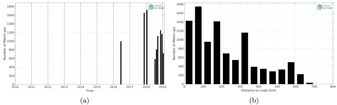
Figure 1: Number of match-ups between TSG-LEGOS-DM and SMAP-L3-JPL-V4.3-8DAY-RUNNING-60KM SSS as a function of time (a) and as function of the distance to coast (b) over the Congo river plume Pi-MEP region and for the full satellite product period.
