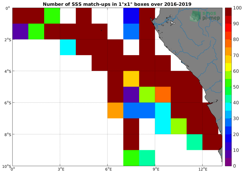
Figure 4: Number of SSS match-ups between TSG-LEGOS-DM SSS and the SMAP-L3-JPL-V4.3-8DAY-RUNNING-60KM SSS product for the Congo river plume Pi-MEP region over 1°x1° boxes and for the full satellite product period.
