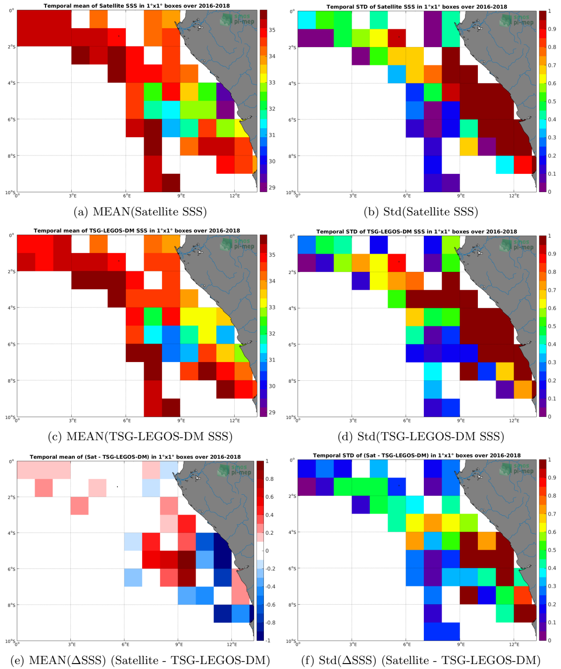
Figure 6: Temporal mean (left) and Std (right) of SSS from SMAP-L3-JPL-V4.3-8DAY-RUNNING-60KM (top), TSG-LEGOS-DM (middle), and of \Delta SSS (Satellite - TSG-LEGOS-DM). Only match-up pairs are used to generate these maps.
