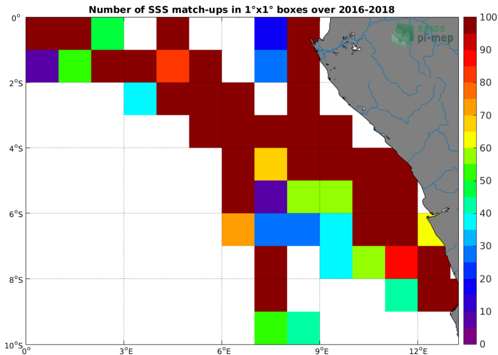
Figure 4: Number of SSS match-ups between TSG-LEGOS-DM SSS and the SMAP-L3-JPL-V4.3-8DAY-RUNNING-60KM SSS product for the Congo river plume Pi-MEP region over 1^\circ \times 1^\circ boxes and for the full satellite product period.
