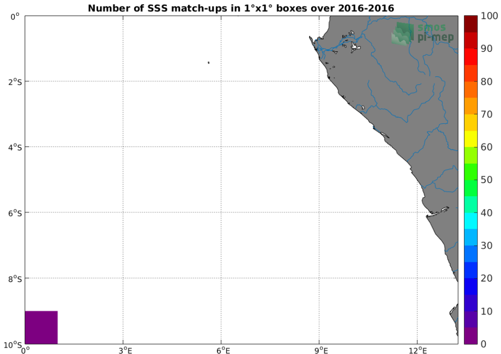
Figure 4: Number of SSS match-ups between TSG-POLARSTERN SSS and the SMAP-L3-JPL-V4.2-8DAY-RUNNING-60KM SSS product for the Congo river plume Pi-MEP region over 1°x1° boxes and for the full satellite product period.
