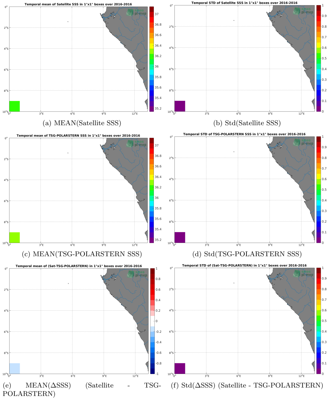
Figure 6: Temporal mean (left) and Std (right) of SSS from SMAP-L3-JPL-V4.2-8DAY-RUNNING-60KM (top), TSG-POLARSTERN (middle), and of \Delta SSS (Satellite - TSG-POLARSTERN). Only match-up pairs are used to generate these maps.
