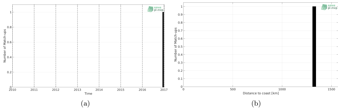
Figure 1: Number of match-ups between TSG-POLARSTERN and SMAP-L3-JPL-V4.2-8DAY-RUNNING-60KM SSS as a function of time (a) and as function of the distance to coast (b) over the Congo river plume Pi-MEP region and for the full satellite product period.
