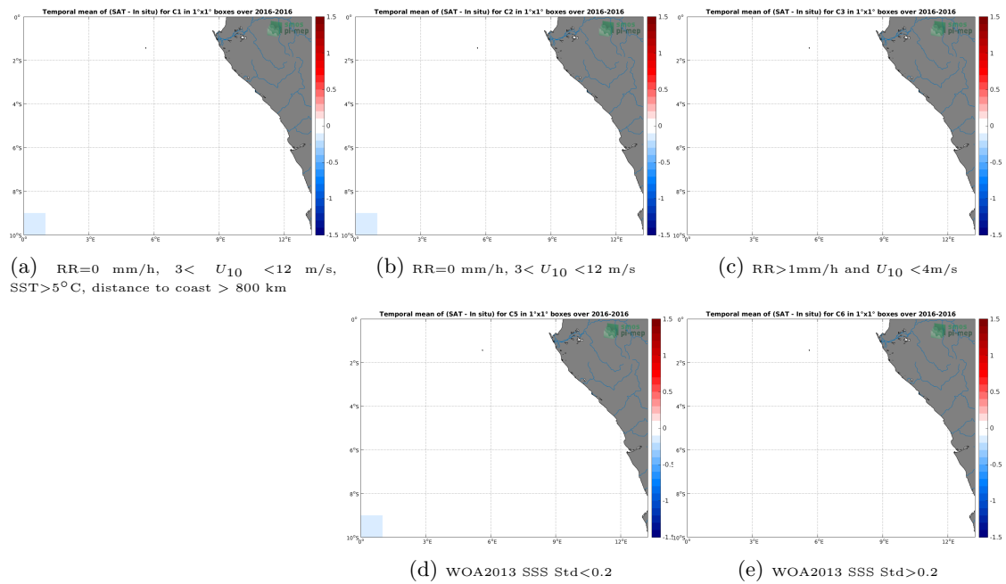
Figure 12: Temporal mean gridded over spatial boxes of size 1^\circ \times 1^\circ of \Delta SSS (SMAP-L3-JPL-V4.2-8DAY-RUNNING-60KM - TSG-POLARSTERN) for 5 different subdatasets corresponding to:RR=0 mm/h, 3 < U_{10} < 12 m/s, SST >5^\circ C, distance to coast > 800 km (a), RR=0 mm/h, 3 < U_{10} < 12 m/s (b), RR >1 mm/h and U_{10} < 4 m/s (c), WOA2013 SSS Std <0.2 (d), WOA2013 SSS Std >0.2 (e).
