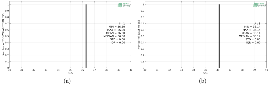
Figure 2: Histograms of SSS from TSG-POLARSTERN (a) and SMAP-L3-JPL-V4.2-8DAY-RUNNING-60KM (b) considering all match-up pairs per bins of 0.1 over the Congo river plume Pi-MEP region and for the full satellite product period.
