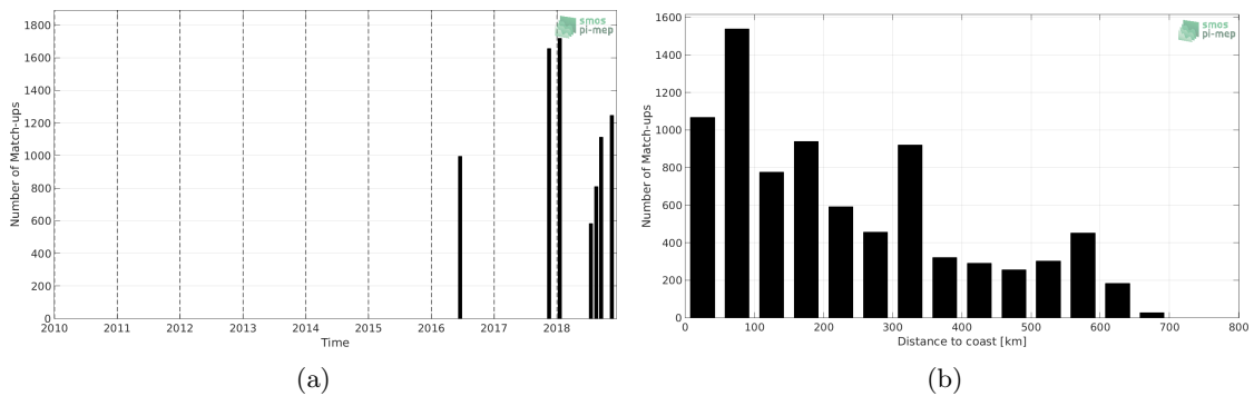
Figure 1: Number of match-ups between TSG-LEGOS-DM and SMAP-L3-JPL-V4.2-8DAY-RUNNING-60KM SSS as a function of time (a) and as function of the distance to coast (b) over the Congo river plume Pi-MEP region and for the full satellite product period.
