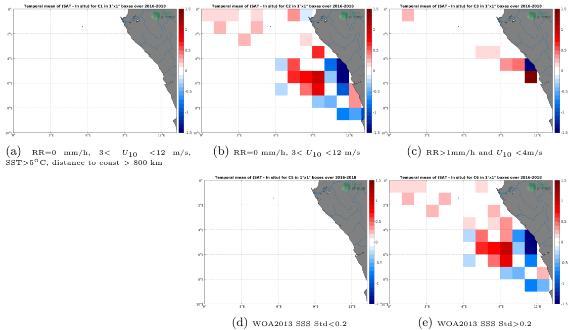
Figure 12: Temporal mean gridded over spatial boxes of size 1^\circ \times 1^\circ of \Delta SSS (SMAP-L3-JPL-V4.2-8DAY-RUNNING-60KM - TSG-LEGOS-DM) for 5 different subdatasets corresponding to:RR=0 mm/h, 3 < U_{10} < 12 m/s, SST > 5^\circ C , distance to coast > 800 km (a), RR=0 mm/h, 3 < U_{10} < 12 m/s (b), RR >1 mm/h and U_{10} < 4 m/s (c), WOA2013 SSS Std <0.2 (d), WOA2013 SSS Std >0.2 (e).
