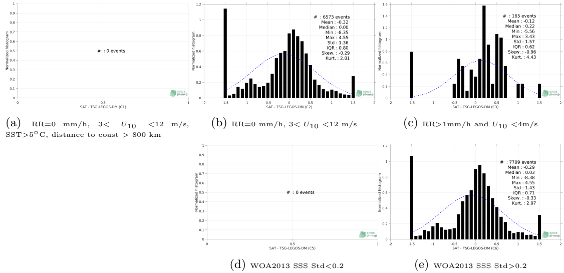
Figure 13: Normalized histogram of \Delta SSS (SMAP-L3-JPL-V4.2-8DAY-RUNNING-60KM - TSG-LEGOS-DM) for 5 different subdatasets corresponding to: RR=0 mm/h, 3 < U_{10} < 12 m/s, SST>5°C, distance to coast > 800 km (a), RR=0 mm/h, 3 < U_{10} < 12 m/s (b), RR>1mm/h and U_{10} < 4 m/s (c), WOA2013 SSS Std<0.2 (d), WOA2013 SSS Std>0.2 (e).
