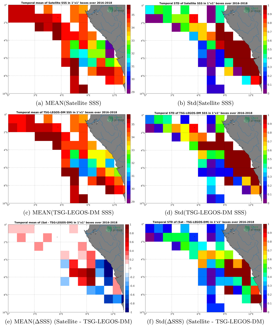
Figure 6: Temporal mean (left) and Std (right) of SSS from SMAP-L3-JPL-V4.2-8DAY-RUNNING-60KM (top), TSG-LEGOS-DM (middle), and of \Delta SSS (Satellite - TSG-LEGOS-DM). Only match-up pairs are used to generate these maps.
