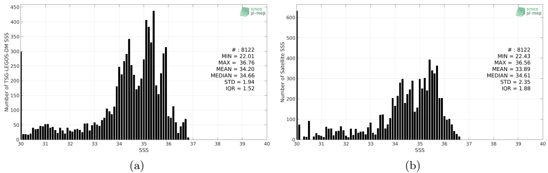
Figure 2: Histograms of SSS from TSG-LEGOS-DM (a) and SMAP-L3-JPL-V4.2-8DAY-RUNNING-60KM (b) considering all match-up pairs per bins of 0.1 over the Congo river plume Pi-MEP region and for the full satellite product period.
