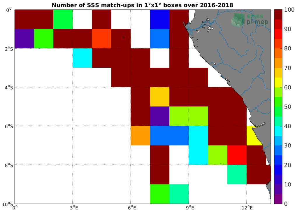
Figure 4: Number of SSS match-ups between TSG-LEGOS-DM SSS and the SMAP-L3-JPL-V4.2-8DAY-RUNNING-60KM SSS product for the Congo river plume Pi-MEP region over 1°x1° boxes and for the full satellite product period.
