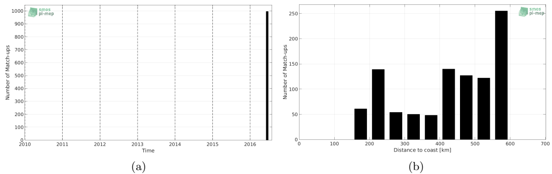
Figure 1: Number of match-ups between TSG-LEGOS-DM and SMAP-L3-JPL-V4-8DAY-RUNNING-60KM SSS as a function of time (a) and as function of the distance to coast (b) over the Congo river plume Pi-MEP region and for the full satellite product period.
