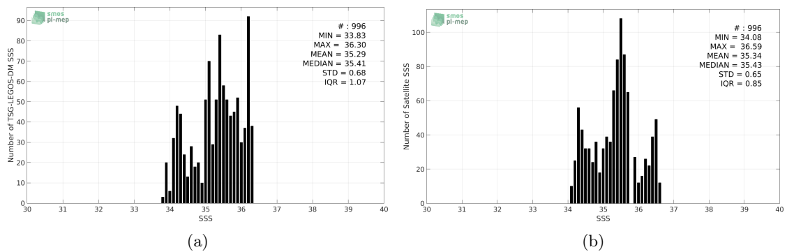
Figure 2: Histograms of SSS from TSG-LEGOS-DM (a) and SMAP-L3-JPL-V4-8DAY-RUNNING-60KM (b) considering all match-up pairs per bins of 0.1 over the Congo river plume Pi-MEP region and for the full satellite product period.
