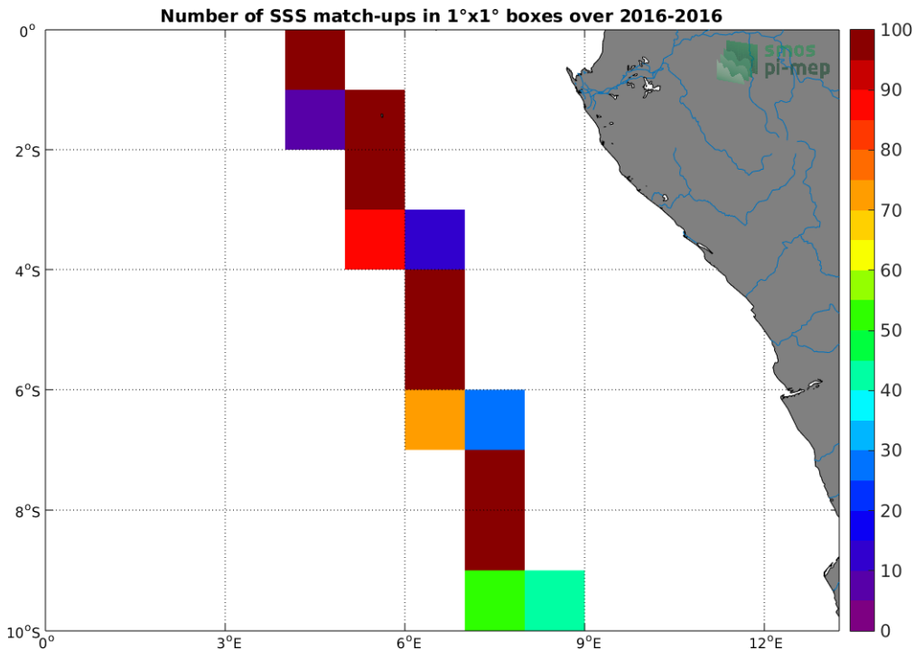
Figure 4: Number of SSS match-ups between TSG-LEGOS-DM SSS and the SMAP-L3-JPL-V4-8DAY-RUNNING-60KM SSS product for the Congo river plume Pi-MEP region over 1^{\circ} \times 1^{\circ} boxes and for the full satellite product period.
