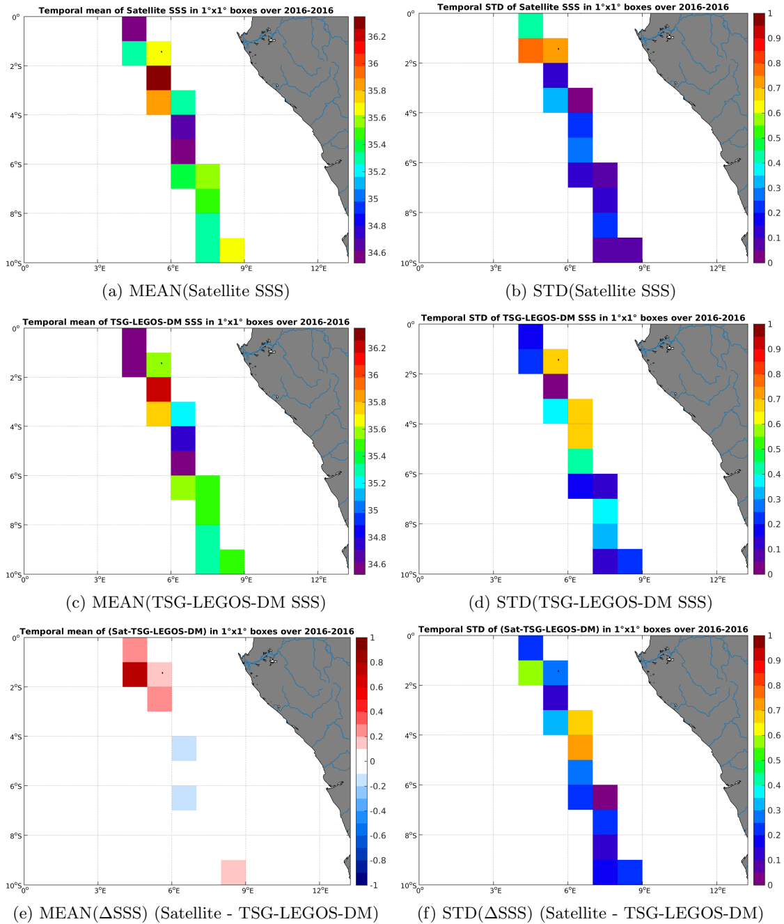
Figure 6: Temporal mean (left) and STD (right) of SSS from SMAP-L3-JPL-V4-8DAY-RUNNING-60KM (top), TSG-LEGOS-DM (middle), and of \Delta SSS (Satellite - TSG-LEGOS-DM). Only match-up pairs are used to generate these maps.
