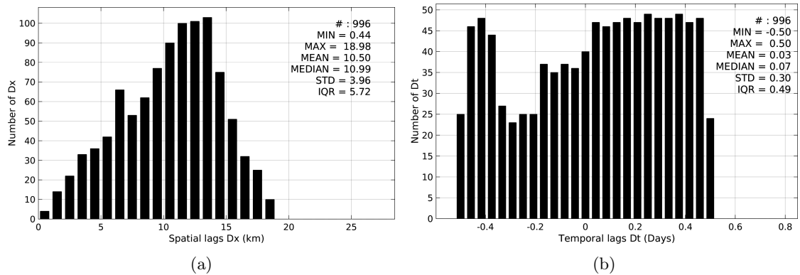
Figure 5: Histograms of the spatial (a) and temporal (b) lags between the time of the TSG-LEGOS-DM measurements and the date of the corresponding SMAP-L3-JPL-V4-8DAY-RUNNING-60KM SSS product.
