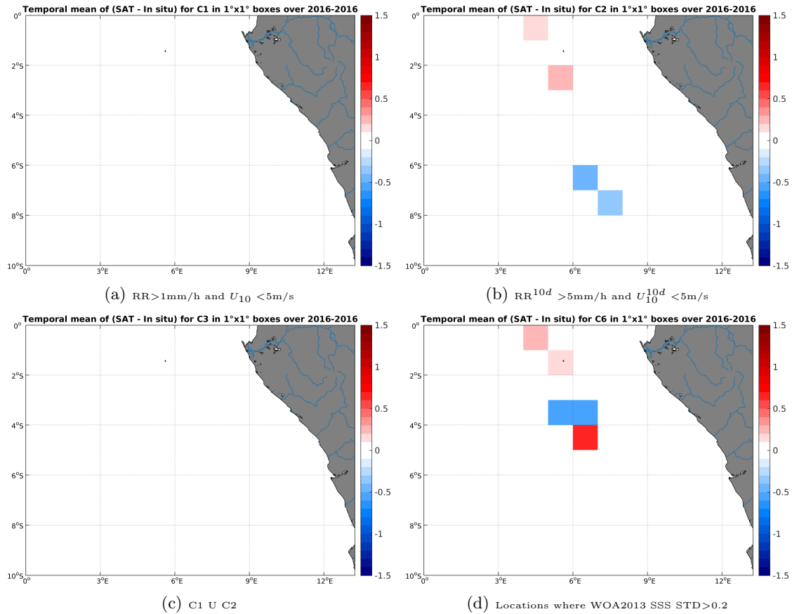
Figure 12: Temporal mean gridded over spatial boxes of size 1^\circ \times 1^\circ of \Delta SSS (SMAP-L3-JPL-V4-8DAY-RUNNING-60KM - TSG-LEGOS-DM) for 4 different subdatasets corresponding to: RR > 1\text{mm/h} and U_{10} < 5\text{m/s} (a), RR^{10d} > 5\text{mm/h} and U_{10}^{10d} < 5\text{m/s} (b), C1 \cup C2 (c), Locations where WOA2013 SSS STD > 0.2 (d).
