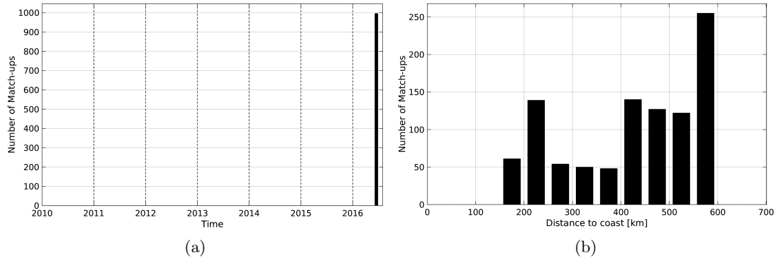
Figure 1: Number of match-ups between TSG-LEGOS-DM and SMAP-L3-JPL-V4-8DAY-RUNNING-60KM SSS as a function of time (a) and as function of the distance to coast (b) over the Congo river plume Pi-MEP region and for the full satellite product period.
