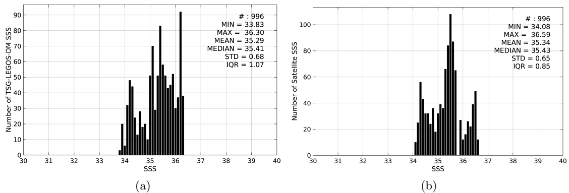
Figure 2: Histograms of SSS from TSG-LEGOS-DM (a) and SMAP-L3-JPL-V4-8DAY-RUNNING-60KM (b) considering all match-up pairs per bins of 0.1 over the Congo river plume Pi-MEP region and for the full satellite product period.
