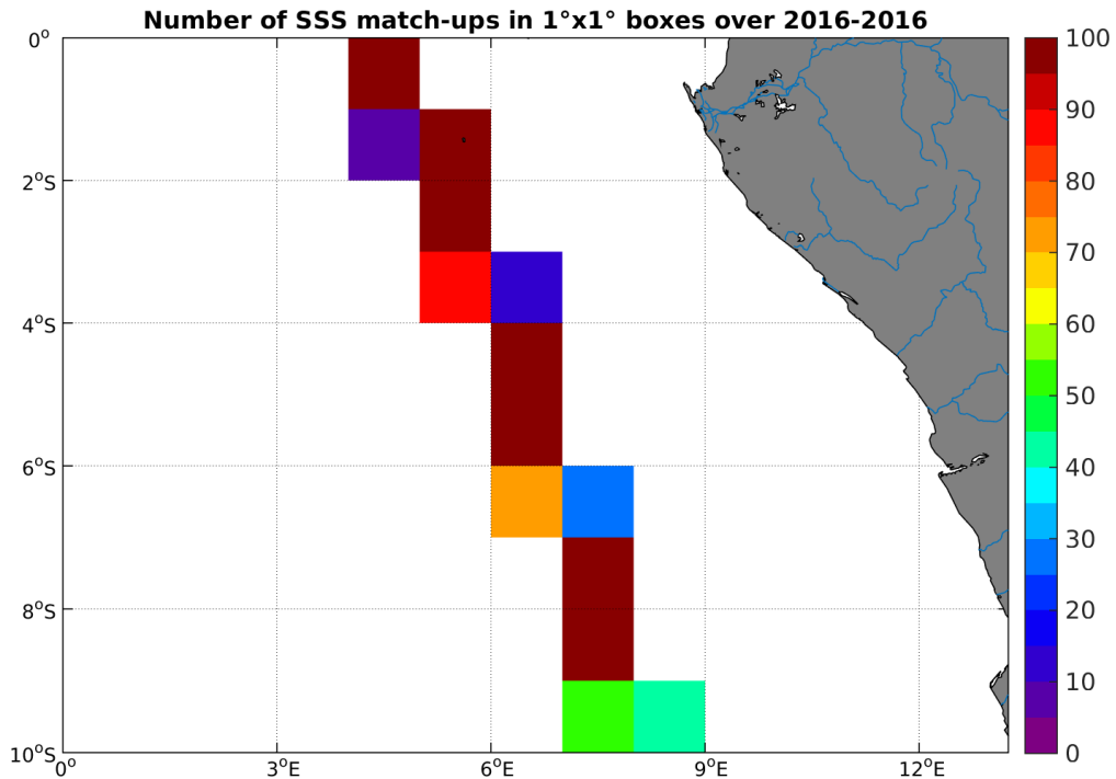
Figure 4: Number of SSS match-ups between TSG-LEGOS-DM SSS and the SMAP-L3-JPL-V4-8DAY-RUNNING-60KM SSS product for the Congo river plume Pi-MEP region over 1^\circ \times 1^\circ boxes and for the full satellite product period.
