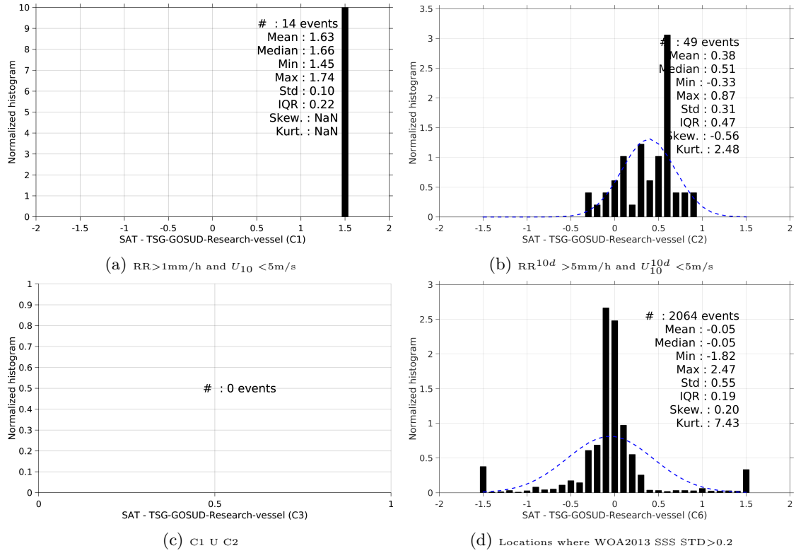
Figure 13: Normalized histogram of \Delta\text{SSS} (SMAP-L3-JPL-V4-8DAY-RUNNING-60KM - TSG-GOSUD-Research-vessel) for 6 different subdatasets corresponding to: RR > 1mm/h and U_{10} < 5\text{m/s} (a), RR^{10d} > 5\text{mm/h} and U_{10}^{10d} < 5\text{m/s} (b), C1 U C2 (c), Locations where WOA2013 SSS STD > 0.2 (d).
