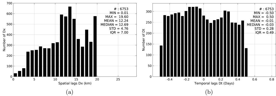
Figure 5: Histograms of the spatial (a) and temporal (b) lags between the time of the TSG-GOSUD-Research-vessel measurements and the date of the corresponding SMAP-L3-JPL-V4-8DAY-RUNNING-60KM SSS product.
