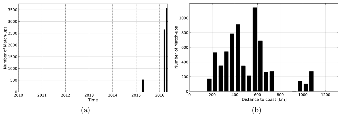
Figure 1: Number of match-ups between TSG-GOSUD-Research-vessel and SMAP-L3-JPL-V4-8DAY-RUNNING-60KM SSS as a function of time (a) and as function of the distance to coast (b) over the Congo river plume Pi-MEP region and for the full satellite product period.
