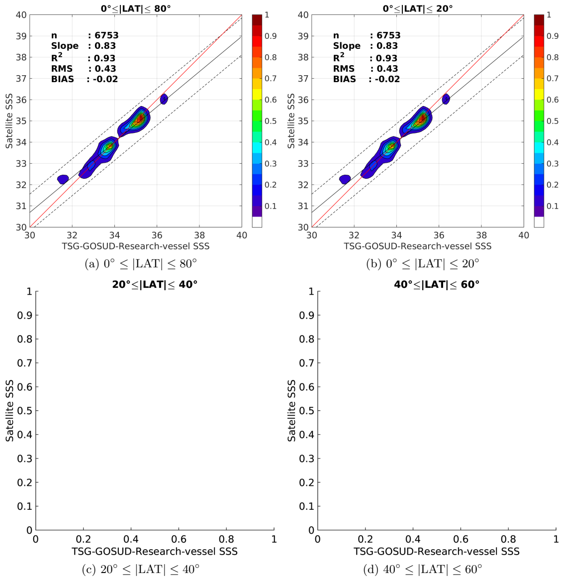
Figure 9: Contour maps of the concentration of SMAP-L3-JPL-V4-8DAY-RUNNING-60KM SSS (y-axis) versus TSG-GOSUD-Research-vessel SSS (x-axis) at match-up pairs for different latitude bands. For each plot, the red line shows x=y . The black thin and dashed lines indicate a linear fit through the data cloud and the \pm 95\% confidence levels, respectively. The number match-up pairs n , the slope and R^2 coefficient of the linear fit, the root mean square (RMS) and the mean bias between satellite and in situ data are indicated for each latitude band in each plots.
