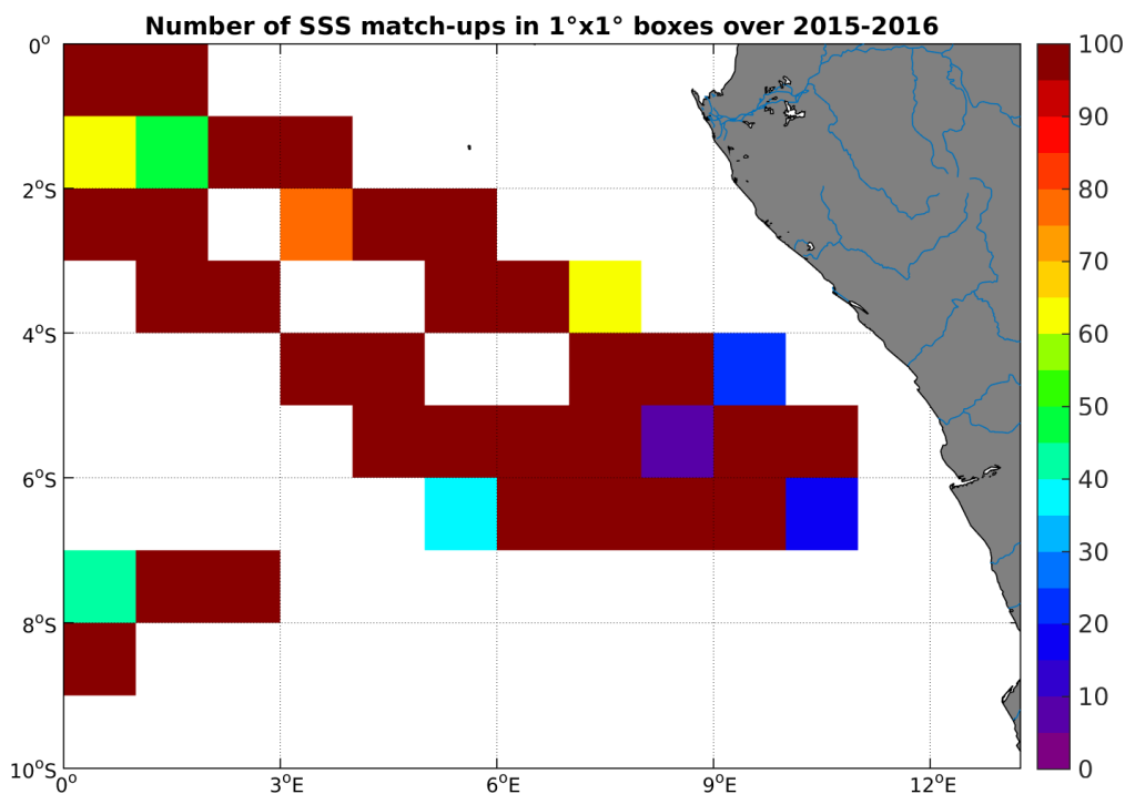
Figure 4: Number of SSS match-ups between TSG-GOSUD-Research-vessel SSS and the SMAP-L3-JPL-V4-8DAY-RUNNING-60KM SSS product for the Congo river plume Pi-MEP region over 1^\circ \times 1^\circ boxes and for the full satellite product period.
