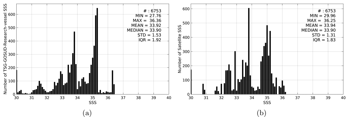
Figure 2: Histograms of SSS from TSG-GOSUD-Research-vessel (a) and SMAP-L3-JPL-V4-8DAY-RUNNING-60KM (b) considering all match-up pairs per bins of 0.1 over the Congo river plume Pi-MEP region and for the full satellite product period.
