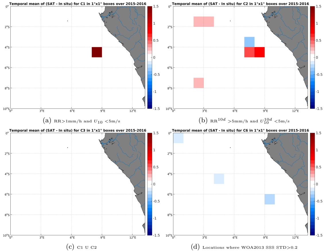
Figure 12: Temporal mean gridded over spatial boxes of size 1^\circ \times 1^\circ of \Delta SSS (SMAP-L3-JPL-V4-8DAY-RUNNING-60KM - TSG-GOSUD-Research-vessel) for 4 different subdatasets corresponding to: RR > 1\text{mm/h} and U_{10} < 5\text{m/s} (a), RR^{10d} > 5\text{mm/h} and U_{10}^{10d} < 5\text{m/s} (b), C1 U C2 (c), Locations where WOA2013 SSS STD > 0.2 (d).
