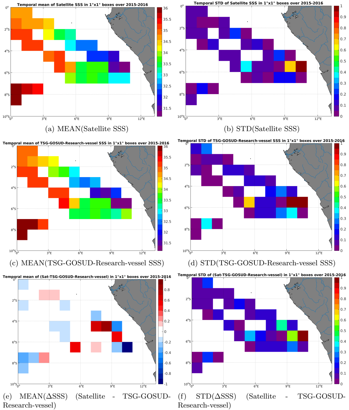
Figure 6: Temporal mean (left) and STD (right) of SSS from SMAP-L3-JPL-V4-8DAY-RUNNING-60KM (top), TSG-GOSUD-Research-vessel (middle), and of \Delta SSS (Satellite - TSG-GOSUD-Research-vessel). Only match-up pairs are used to generate these maps.
