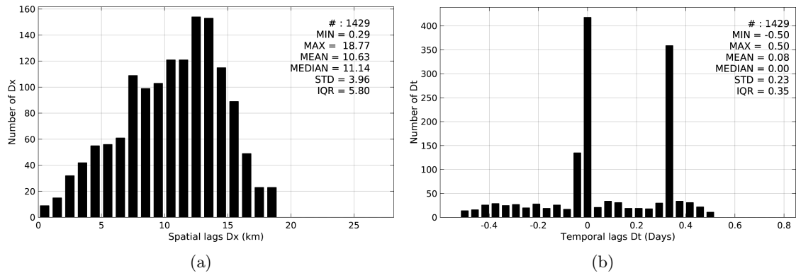
Figure 5: Histograms of the spatial (a) and temporal (b) lags between the time of the Argo measurements and the date of the corresponding SMAP-L3-JPL-V4-8DAY-RUNNING-60KM SSS product.
