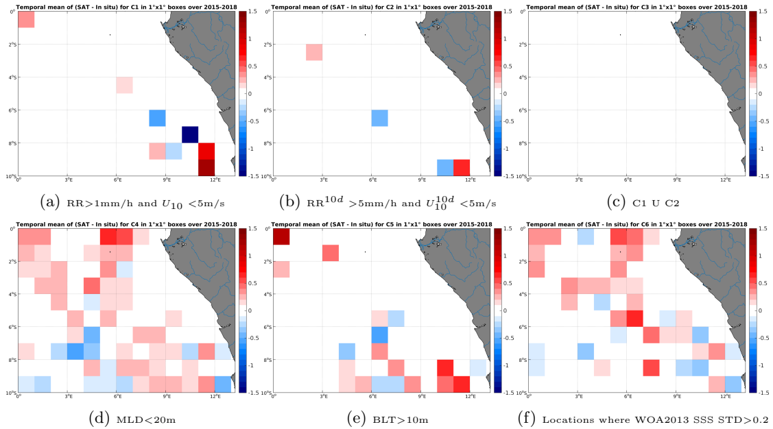
Figure 12: Temporal mean gridded over spatial boxes of size 1°x1° of \Delta SSS (SMAP-L3-JPL-V4-8DAY-RUNNING-60KM - Argo) for 6 different subdatasets corresponding to:RR>1mm/h and U_{10} < 5\text{m/s} (a), RR^{10d} > 5\text{mm/h} and U_{10}^{10d} < 5\text{m/s} (b), C1 U C2 (c),MLD<20m (d),BLT>10m (e),Locations where WOA2013 SSS STD>0.2 (f).
