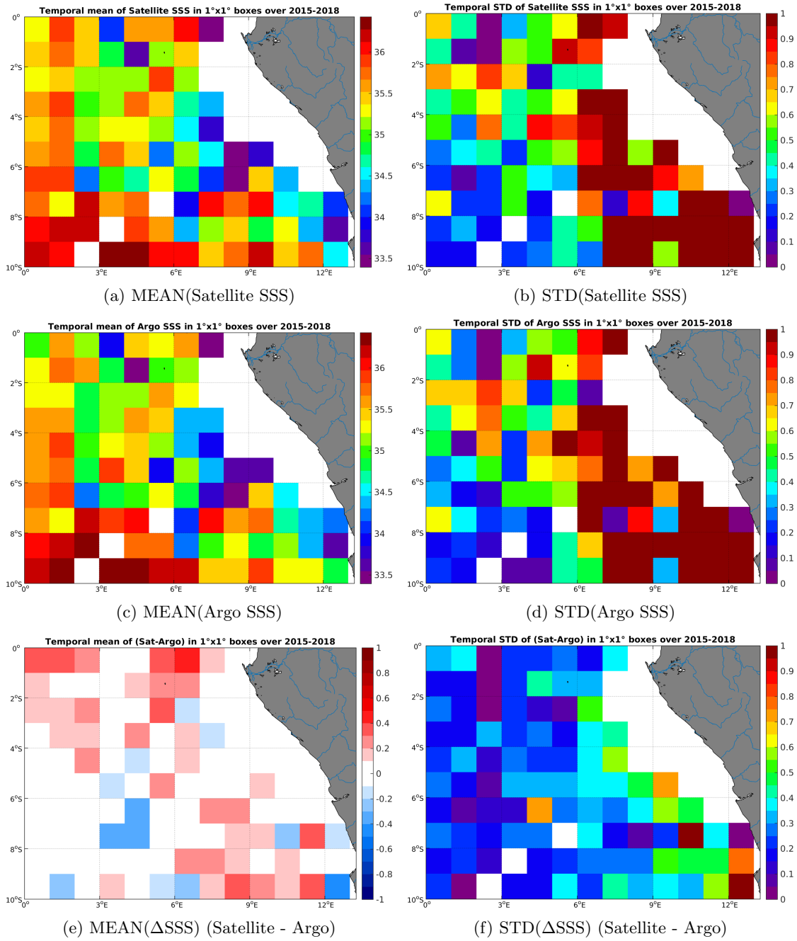
Figure 6: Temporal mean (left) and STD (right) of SSS from SMAP-L3-JPL-V4-8DAY-RUNNING-60KM (top), Argo (middle), and of \Delta SSS (Satellite - Argo). Only match-up pairs are used to generate these maps.
