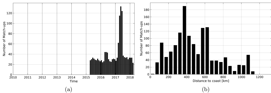
Figure 1: Number of match-ups between Argo and SMAP-L3-JPL-V4-8DAY-RUNNING-60KM SSS as a function of time (a) and as function of the distance to coast (b) over the Congo river plume Pi-MEP region and for the full satellite product period.
