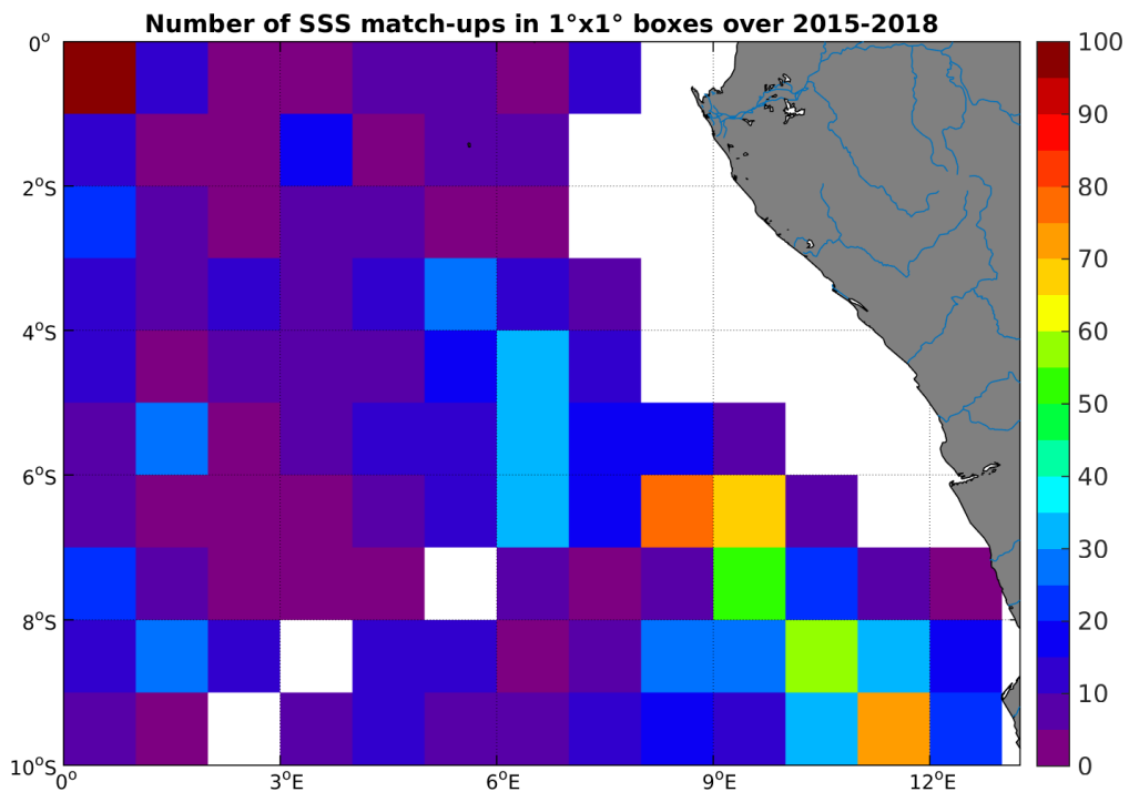
Figure 4: Number of SSS match-ups between Argo SSS and the SMAP-L3-JPL-V4-8DAY-RUNNING-60KM SSS product for the Congo river plume Pi-MEP region over 1^\circ \times 1^\circ boxes and for the full satellite product period.
