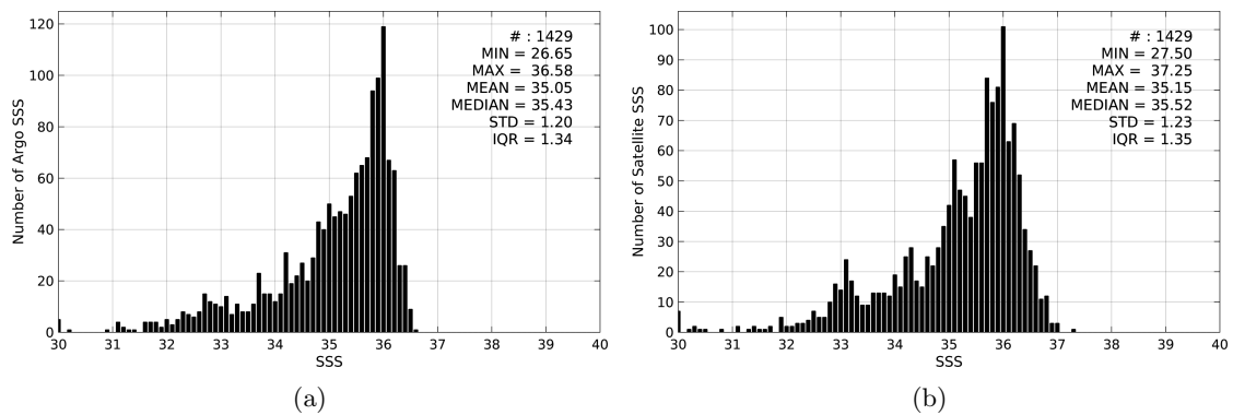
Figure 2: Histograms of SSS from Argo (a) and SMAP-L3-JPL-V4-8DAY-RUNNING-60KM (b) considering all match-up pairs per bins of 0.1 over the Congo river plume Pi-MEP region and for the full satellite product period.
