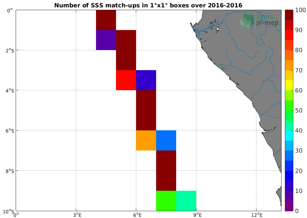
Figure 4: Number of SSS match-ups between TSG-LEGOS-DM SSS and the SMAP-L3-JPL-V4-MONTHLY-60KM SSS product for the Congo river plume Pi-MEP region over 1^\circ \times 1^\circ boxes and for the full satellite product period.
