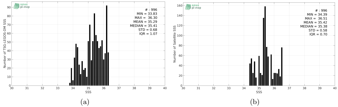
Figure 2: Histograms of SSS from TSG-LEGOS-DM (a) and SMAP-L3-JPL-V4-MONTHLY-60KM (b) considering all match-up pairs per bins of 0.1 over the Congo river plume Pi-MEP region and for the full satellite product period.
