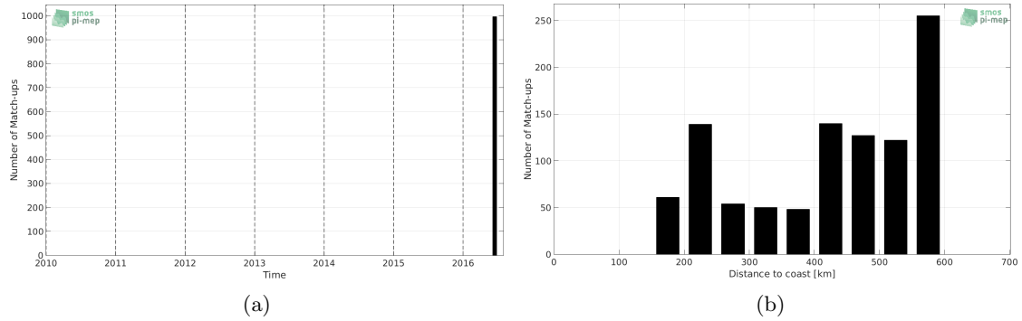
Figure 1: Number of match-ups between TSG-LEGOS-DM and SMAP-L3-JPL-V4-MONTHLY-60KM SSS as a function of time (a) and as function of the distance to coast (b) over the Congo river plume Pi-MEP region and for the full satellite product period.
