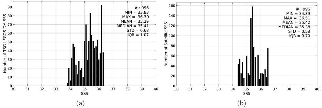
Figure 2: Histograms of SSS from TSG-LEGOS-DM (a) and SMAP-L3-JPL-V4-MONTHLY-60KM (b) considering all match-up pairs per bins of 0.1 over the Congo river plume Pi-MEP region and for the full satellite product period.
