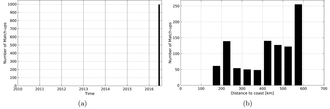
Figure 1: Number of match-ups between TSG-LEGOS-DM and SMAP-L3-JPL-V4-MONTHLY-60KM SSS as a function of time (a) and as function of the distance to coast (b) over the Congo river plume Pi-MEP region and for the full satellite product period.
