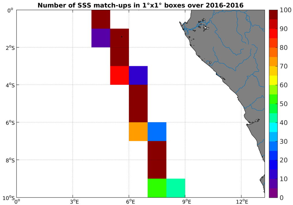
Figure 4: Number of SSS match-ups between TSG-LEGOS-DM SSS and the SMAP-L3-JPL-V4-MONTHLY-60KM SSS product for the Congo river plume Pi-MEP region over 1°x1° boxes and for the full satellite product period.
