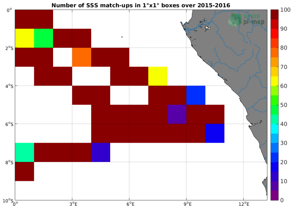
Figure 4: Number of SSS match-ups between TSG-GOSUD-Research-vessel SSS and the SMAP-L3-JPL-V4-MONTHLY-60KM SSS product for the Congo river plume Pi-MEP region over 1^\circ \times 1^\circ boxes and for the full satellite product period.
