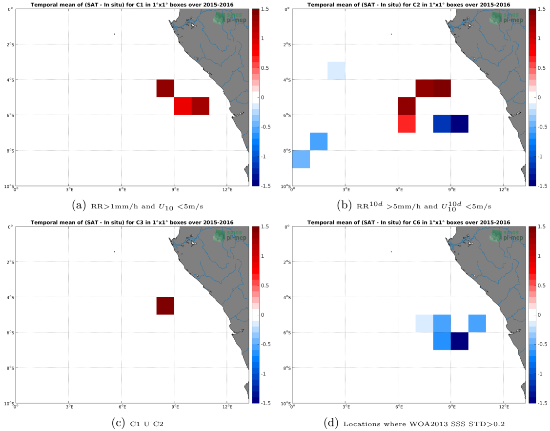
Figure 12: Temporal mean gridded over spatial boxes of size 1^\circ \times 1^\circ of \Delta SSS (SMAP-L3-JPL-V4-MONTHLY-60KM - TSG-GOSUD-Research-vessel) for 4 different subdatasets corresponding to: RR > 1\text{mm/h} and U_{10} < 5\text{m/s} (a), RR^{10d} > 5\text{mm/h} and U_{10}^{10d} < 5\text{m/s} (b), C1 \cup C2 (c), Locations where WOA2013 SSS STD > 0.2 (d).
