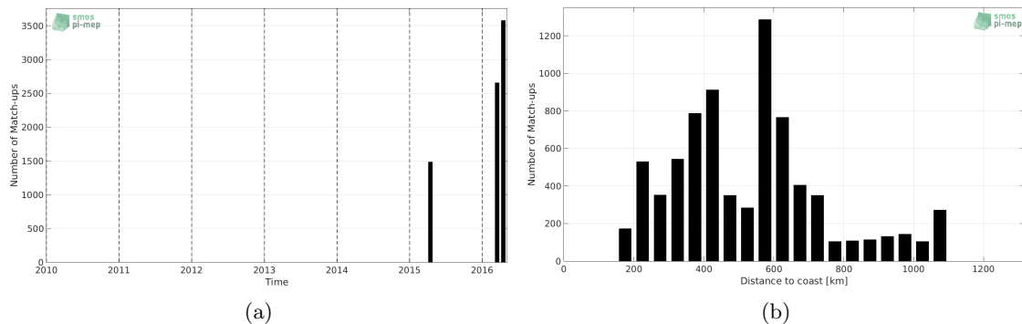
Figure 1: Number of match-ups between TSG-GOSUD-Research-vessel and SMAP-L3-JPL-V4-MONTHLY-60KM SSS as a function of time (a) and as function of the distance to coast (b) over the Congo river plume Pi-MEP region and for the full satellite product period.
