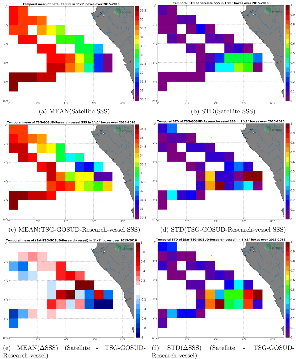
Figure 6: Temporal mean (left) and STD (right) of SSS from SMAP-L3-JPL-V4-MONTHLY-60KM (top), TSG-GOSUD-Research-vessel (middle), and of \Delta SSS (Satellite - TSG-GOSUD-Research-vessel). Only match-up pairs are used to generate these maps.
