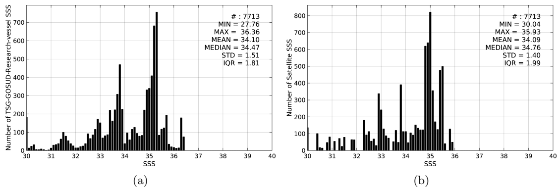
Figure 2: Histograms of SSS from TSG-GOSUD-Research-vessel (a) and SMAP-L3-JPL-V4-MONTHLY-60KM (b) considering all match-up pairs per bins of 0.1 over the Congo river plume Pi-MEP region and for the full satellite product period.
