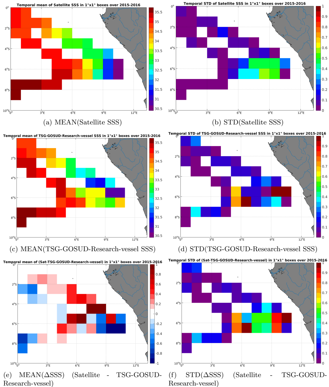
Figure 6: Temporal mean (left) and STD (right) of SSS from SMAP-L3-JPL-V4-MONTHLY-60KM (top), TSG-GOSUD-Research-vessel (middle), and of \Delta SSS (Satellite - TSG-GOSUD-Research-vessel). Only match-up pairs are used to generate these maps.
