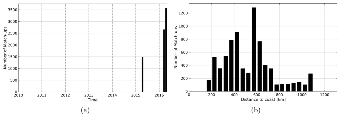
Figure 1: Number of match-ups between TSG-GOSUD-Research-vessel and SMAP-L3-JPL-V4-MONTHLY-60KM SSS as a function of time (a) and as function of the distance to coast (b) over the Congo river plume Pi-MEP region and for the full satellite product period.
