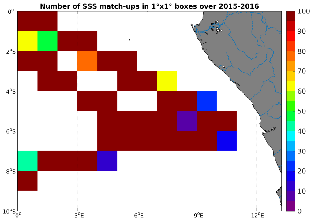
Figure 4: Number of SSS match-ups between TSG-GOSUD-Research-vessel SSS and the SMAP-L3-JPL-V4-MONTHLY-60KM SSS product for the Congo river plume Pi-MEP region over 1^{\circ} \times 1^{\circ} boxes and for the full satellite product period.
