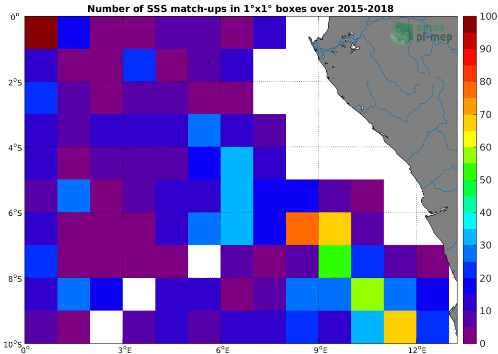
Figure 4: Number of SSS match-ups between Argo SSS and the SMAP-L3-JPL-V4-MONTHLY-60KM SSS product for the Congo river plume Pi-MEP region over 1^\circ \times 1^\circ boxes and for the full satellite product period.
