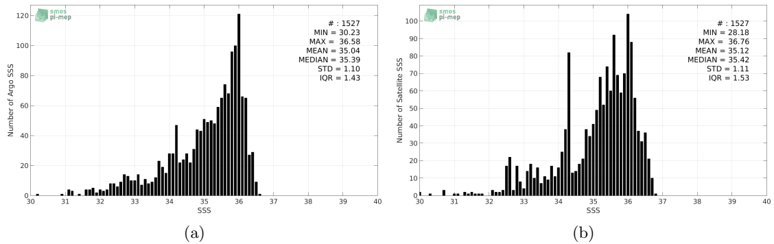
Figure 2: Histograms of SSS from Argo (a) and SMAP-L3-JPL-V4-MONTHLY-60KM (b) considering all match-up pairs per bins of 0.1 over the Congo river plume Pi-MEP region and for the full satellite product period.
