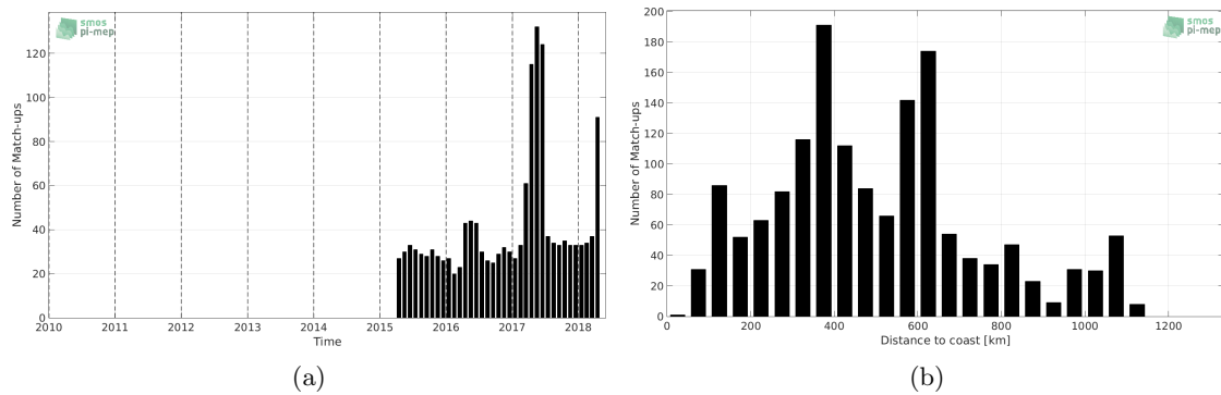
Figure 1: Number of match-ups between Argo and SMAP-L3-JPL-V4-MONTHLY-60KM SSS as a function of time (a) and as function of the distance to coast (b) over the Congo river plume Pi-MEP region and for the full satellite product period.
