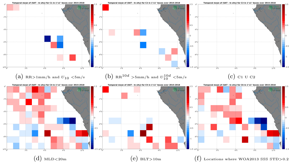
Figure 12: Temporal mean gridded over spatial boxes of size 1^\circ \times 1^\circ of \Delta\text{SSS} (SMAP-L3-JPL-V4-MONTHLY-60KM - Argo) for 6 different subdatasets corresponding to: \text{RR} > 1\text{mm/h} and U_{10} < 5\text{m/s} (a), \text{RR}^{10d} > 5\text{mm/h} and U_{10}^{10d} < 5\text{m/s} (b), C1 U C2 (c), \text{MLD} < 20\text{m} (d), \text{BLT} > 10\text{m} (e), Locations where WOA2013 SSS STD > 0.2 (f).
