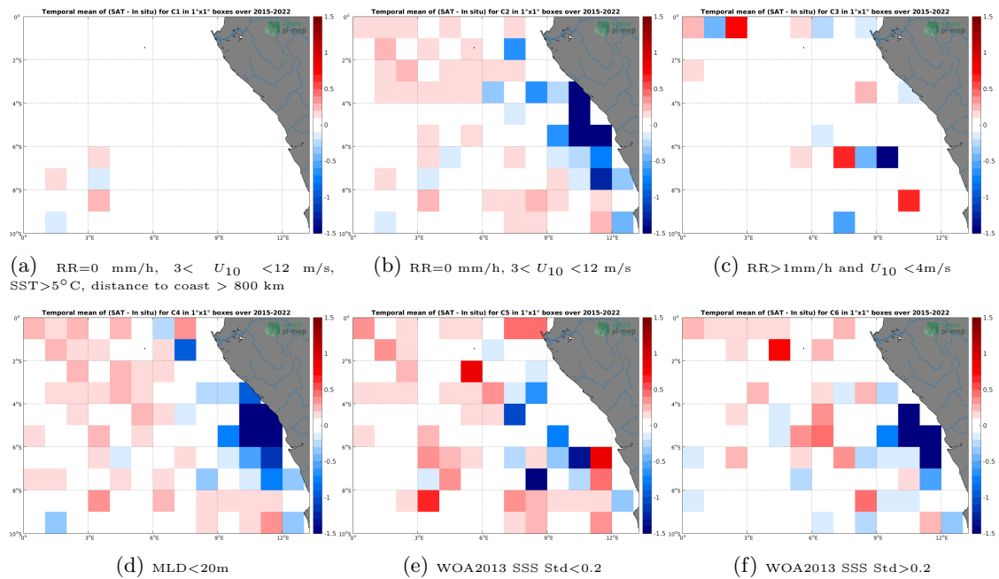
Figure 12: Temporal mean gridded over spatial boxes of size 1^\circ \times 1^\circ of \Delta SSS (SMAP SSS L2-AVERAGED v5.0 (JPL) - Argo) for 6 different subdatasets corresponding to:RR=0 mm/h, 3 < U_{10} < 12 m/s, SST >5^\circ C, distance to coast > 800 km (a), RR=0 mm/h, 3 < U_{10} < 12 m/s (b), RR >1 mm/h and U_{10} < 4 m/s (c),MLD <20 m (d),WOA2013 SSS Std <0.2 (e),WOA2013 SSS Std >0.2 (f).
