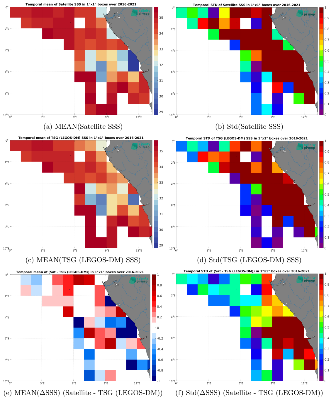
Figure 7: Temporal mean (left) and Std (right) of SSS from SMAP SSS L2 v6 (RSS) (top), TSG (LEGOS-DM) (middle), and of \Delta SSS (Satellite - TSG (LEGOS-DM)). Only match-up pairs are used to generate these maps.
