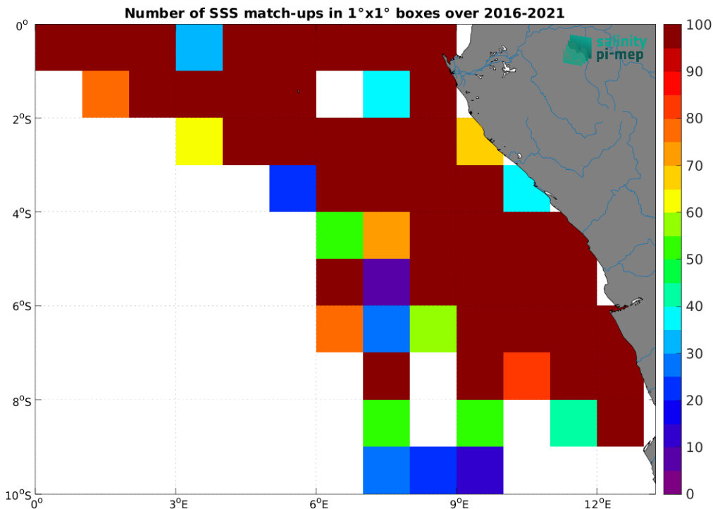
Figure 5: Number of SSS match-ups between TSG (LEGOS-DM) SSS and the SMAP SSS L2 v6 (RSS) SSS product for the Congo river plume Pi-MEP region over 1^\circ \times 1^\circ boxes and for the full satellite product period.
