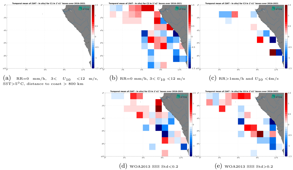
Figure 14: Temporal mean gridded over spatial boxes of size 1^\circ \times 1^\circ of \Delta SSS (SMAP SSS L2 v6 (RSS) - TSG (LEGOS-DM)) for 5 different subdatasets corresponding to:RR=0 mm/h, 3 < U_{10} < 12 m/s, SST > 5°C, distance to coast > 800 km (a), RR=0 mm/h, 3 < U_{10} < 12 m/s (b), RR > 1mm/h and U_{10} < 4 m/s (c), WOA2013 SSS Std < 0.2 (d), WOA2013 SSS Std > 0.2 (e).
