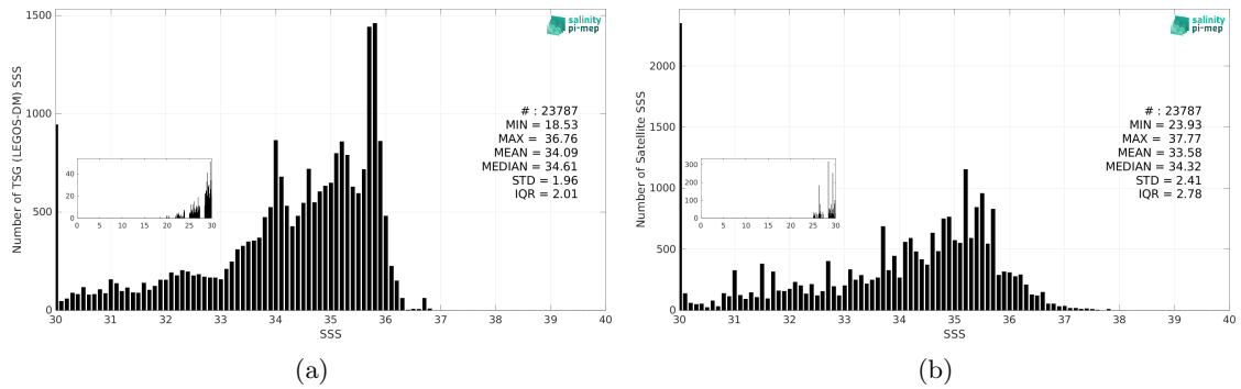
Figure 3: Histograms of SSS from TSG (LEGOS-DM) (a) and SMAP SSS L2 v6 (RSS) (b) considering all match-up pairs per bins of 0.1 over the Congo river plume Pi-MEP region and for the full satellite product period.
