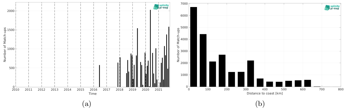
Figure 2: Number of match-ups between TSG (LEGOS-DM) and SMAP SSS L2 v6 (RSS) SSS as a function of time (a) and as function of the distance to coast (b) over the Congo river plume Pi-MEP region and for the full satellite product period.
