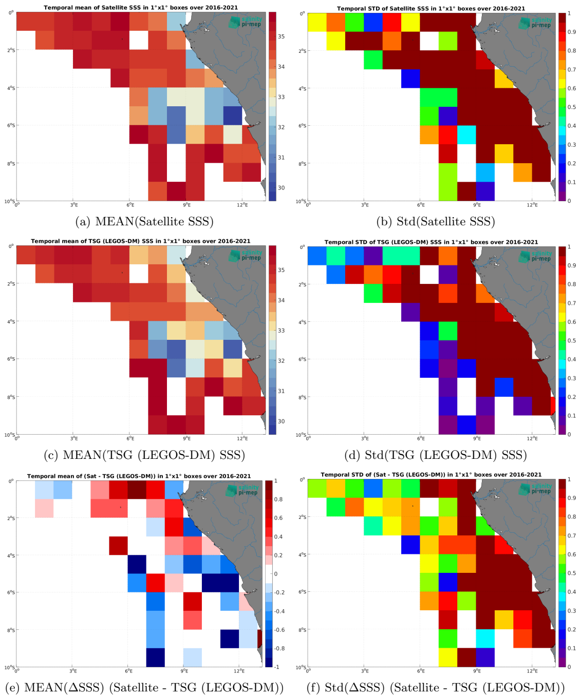
Figure 7: Temporal mean (left) and Std (right) of SSS from SMAP SSS L2 v6 - 40 km (RSS) (top), TSG (LEGOS-DM) (middle), and of \Delta SSS (Satellite - TSG (LEGOS-DM)). Only match-up pairs are used to generate these maps.
