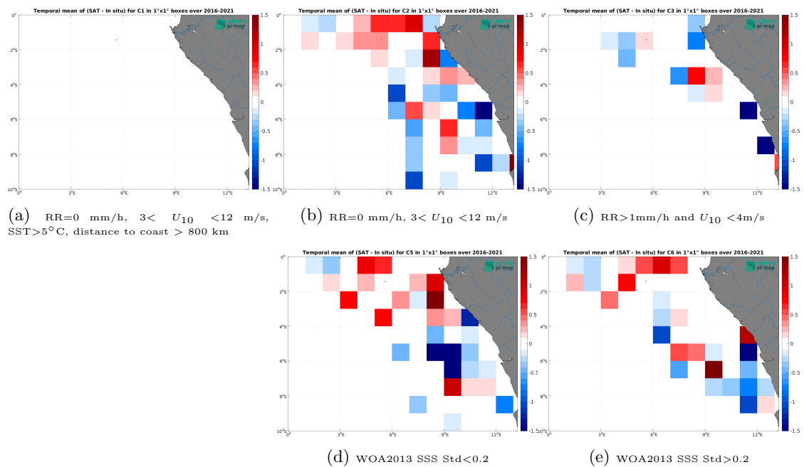
Figure 14: Temporal mean gridded over spatial boxes of size 1^\circ \times 1^\circ of \Delta SSS (SMAP SSS L2 v6 - 40 km (RSS) - TSG (LEGOS-DM)) for 5 different subdatasets corresponding to: RR=0 mm/h, 3 < U_{10} < 12 m/s, SST > 5°C, distance to coast > 800 km (a), RR=0 mm/h, 3 < U_{10} < 12 m/s (b), RR > 1mm/h and U_{10} < 4 m/s (c), WOA2013 SSS Std < 0.2 (d), WOA2013 SSS Std > 0.2 (e).
