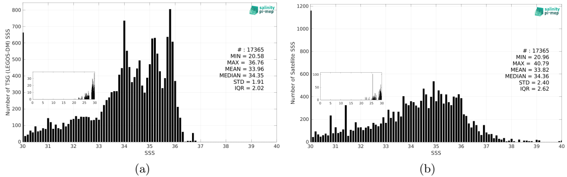
Figure 3: Histograms of SSS from TSG (LEGOS-DM) (a) and SMAP SSS L2 v6 - 40 km (RSS) (b) considering all match-up pairs per bins of 0.1 over the Congo river plume Pi-MEP region and for the full satellite product period.
