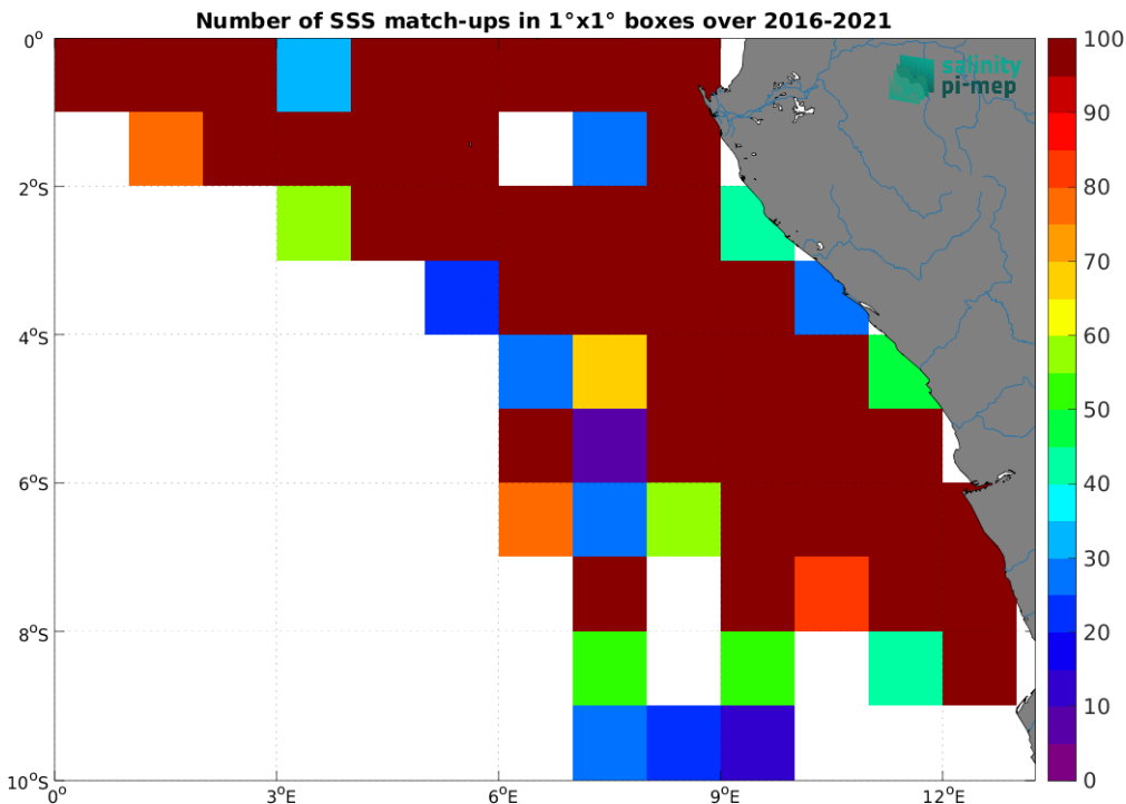
Figure 5: Number of SSS match-ups between TSG (LEGOS-DM) SSS and the SMAP SSS L2 v6 - 40 km (RSS) SSS product for the Congo river plume Pi-MEP region over 1^\circ \times 1^\circ boxes and for the full satellite product period.
