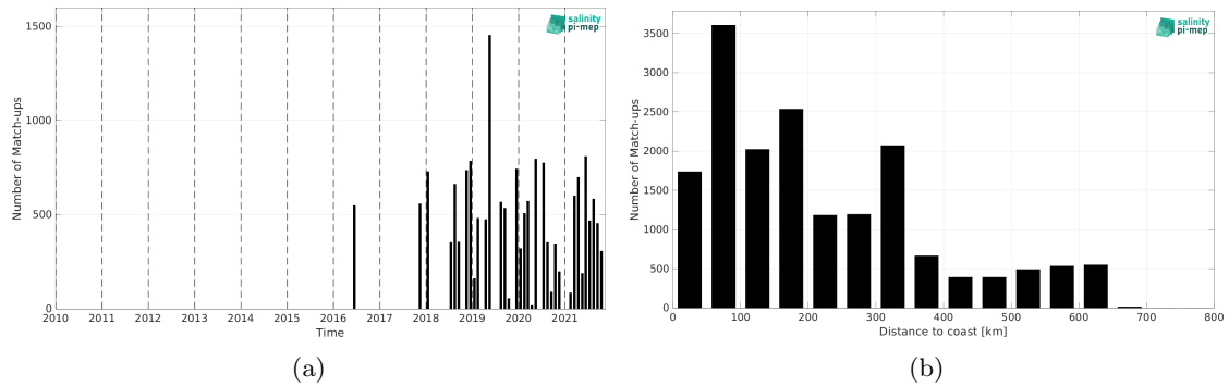
Figure 2: Number of match-ups between TSG (LEGOS-DM) and SMAP SSS L2 v6 - 40 km (RSS) SSS as a function of time (a) and as function of the distance to coast (b) over the Congo river plume Pi-MEP region and for the full satellite product period.
