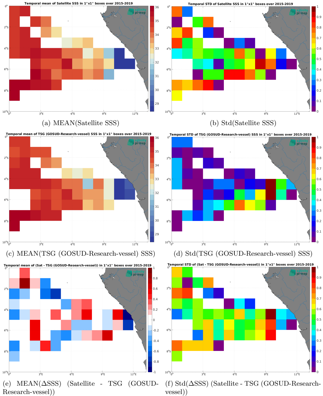
Figure 7: Temporal mean (left) and Std (right) of SSS from SMAP SSS L2 v6 - 40 km (RSS) (top), TSG (GOSUD-Research-vessel) (middle), and of \Delta SSS (Satellite - TSG (GOSUD-Research-vessel)). Only match-up pairs are used to generate these maps.
