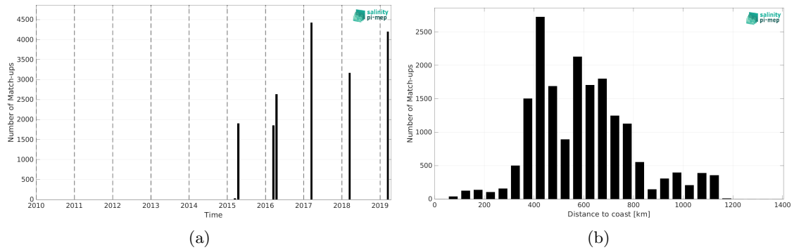
Figure 2: Number of match-ups between TSG (GOSUD-Research-vessel) and SMAP SSS L2 v6 - 40 km (RSS) SSS as a function of time (a) and as function of the distance to coast (b) over the Congo river plume Pi-MEP region and for the full satellite product period.
