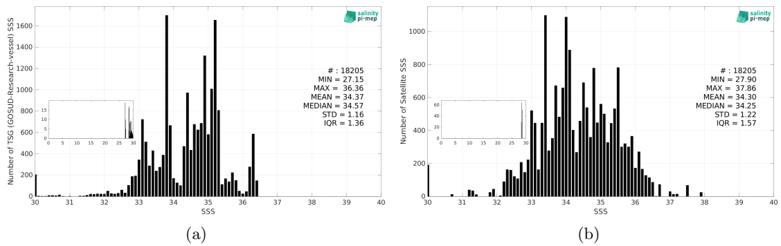
Figure 3: Histograms of SSS from TSG (GOSUD-Research-vessel) (a) and SMAP SSS L2 v6 - 40 km (RSS) (b) considering all match-up pairs per bins of 0.1 over the Congo river plume Pi-MEP region and for the full satellite product period.
