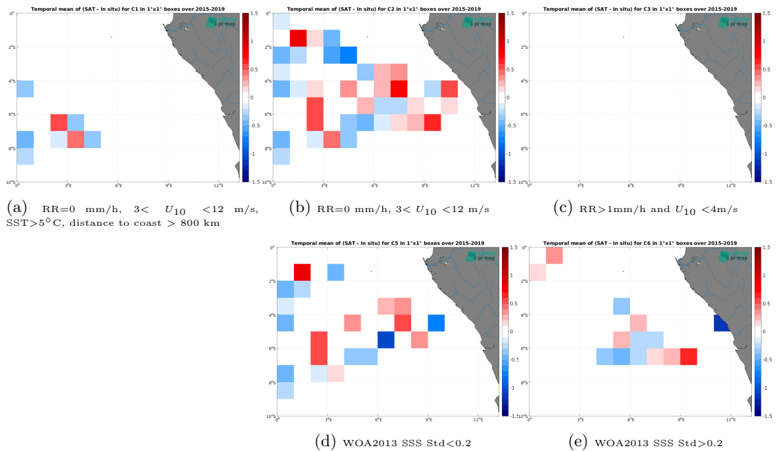
Figure 14: Temporal mean gridded over spatial boxes of size 1^\circ \times 1^\circ of \Delta SSS (SMAP SSS L2 v6 - 40 km (RSS) - TSG (GOSUD-Research-vessel)) for 5 different subdatasets corresponding to:RR=0 mm/h, 3 < U_{10} < 12 m/s, SST>5°C, distance to coast > 800 km (a), RR=0 mm/h, 3 < U_{10} < 12 m/s (b), RR>1mm/h and U_{10} < 4 m/s (c), WOA2013 SSS Std<0.2 (d), WOA2013 SSS Std>0.2 (e).
