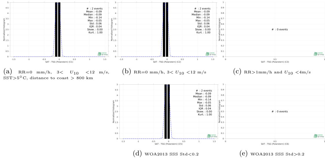
Figure 13: Normalized histogram of \Delta\text{SSS} (SMAP SSS L2 v5 (RSS) - TSG (Polarstern)) for 5 different subdatasets corresponding to: RR=0 mm/h, 3 < U_{10} < 12 m/s, SST>5°C, distance to coast > 800 km (a), RR=0 mm/h, 3 < U_{10} < 12 m/s (b), RR>1mm/h and U_{10} < 4 m/s (c), WOA2013 SSS Std<0.2 (d), WOA2013 SSS Std>0.2 (e).
