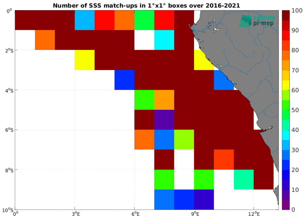
Figure 4: Number of SSS match-ups between TSG (LEGOS-DM) SSS and the SMAP SSS L2 v5 (RSS) SSS product for the Congo river plume Pi-MEP region over 1^{\circ} \times 1^{\circ} boxes and for the full satellite product period.
