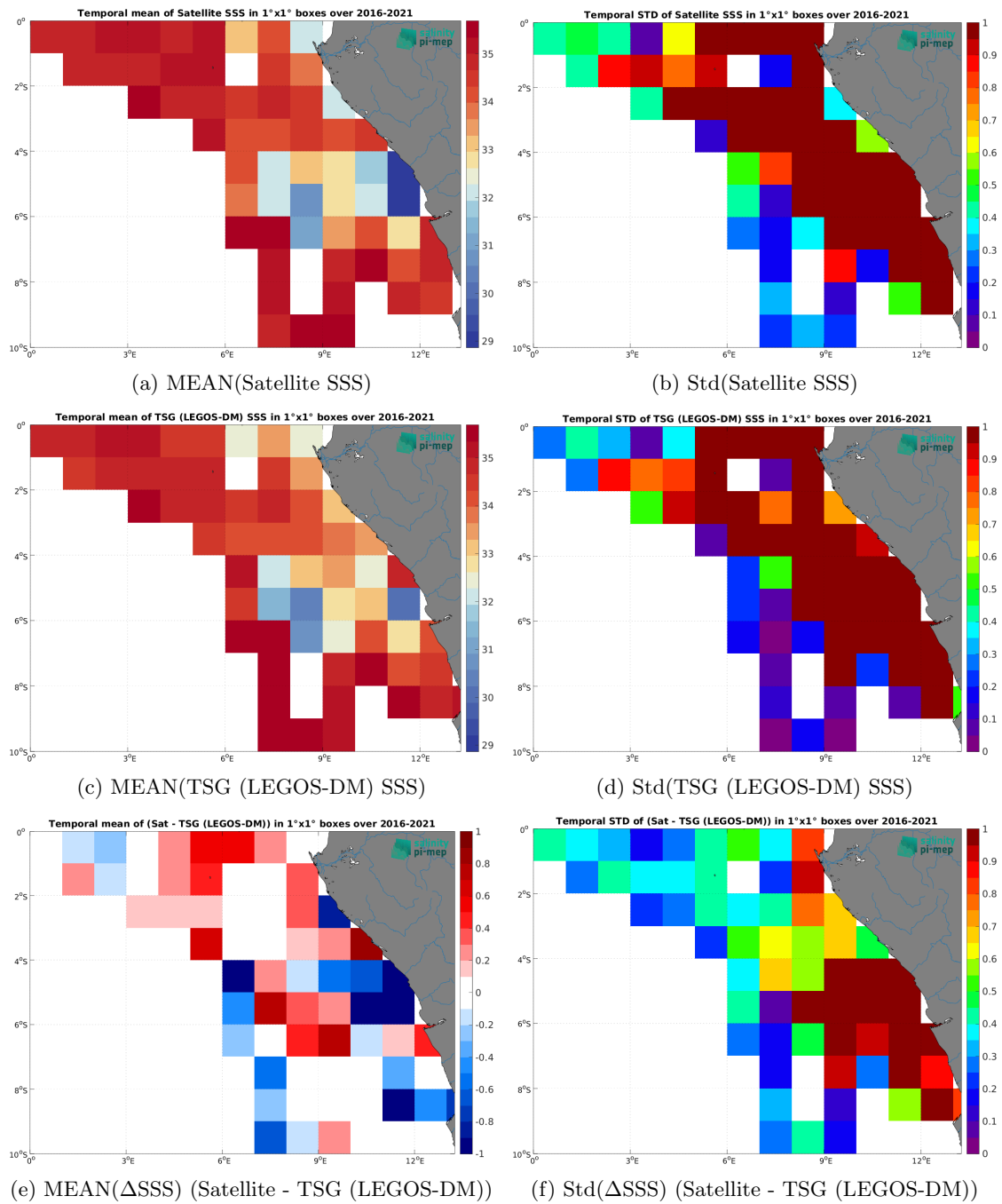
Figure 6: Temporal mean (left) and Std (right) of SSS from SMAP SSS L2 v5 (RSS) (top), TSG (LEGOS-DM) (middle), and of \Delta SSS (Satellite - TSG (LEGOS-DM)). Only match-up pairs are used to generate these maps.
