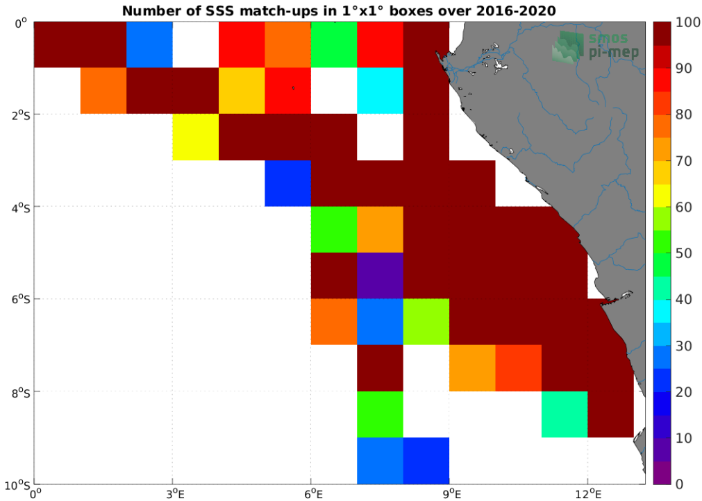
Figure 4: Number of SSS match-ups between TSG (LEGOS-DM) SSS and the SMAP SSS L2 v5 (RSS) SSS product for the Congo river plume Pi-MEP region over 1^\circ \times 1^\circ boxes and for the full satellite product period.
