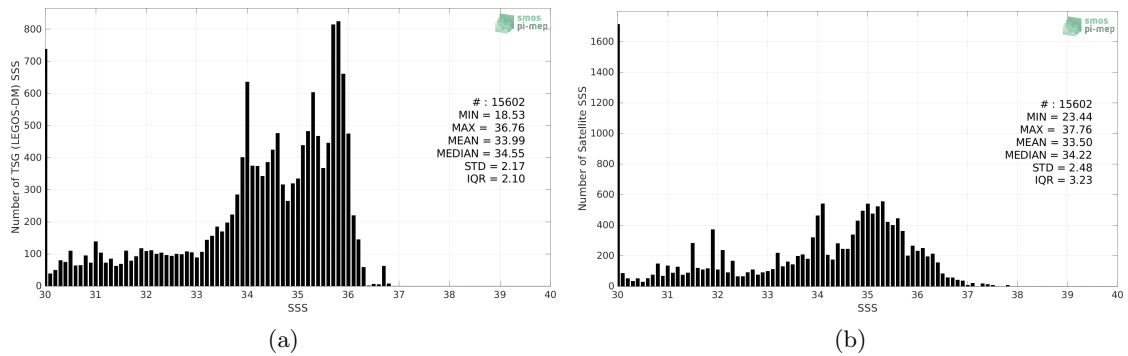
Figure 2: Histograms of SSS from TSG (LEGOS-DM) (a) and SMAP SSS L2 v5 (RSS) (b) considering all match-up pairs per bins of 0.1 over the Congo river plume Pi-MEP region and for the full satellite product period.
