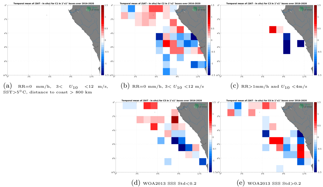
Figure 12: Temporal mean gridded over spatial boxes of size 1^\circ \times 1^\circ of \Delta SSS (SMAP SSS L2 v5 (RSS) - TSG (LEGOS-DM)) for 5 different subdatasets corresponding to:RR=0 mm/h, 3 < U_{10} < 12 m/s, SST > 5^\circ\text{C} , distance to coast > 800 km (a), RR=0 mm/h, 3 < U_{10} < 12 m/s (b), RR > 1 mm/h and U_{10} < 4 m/s (c), WOA2013 SSS Std < 0.2 (d), WOA2013 SSS Std > 0.2 (e).
