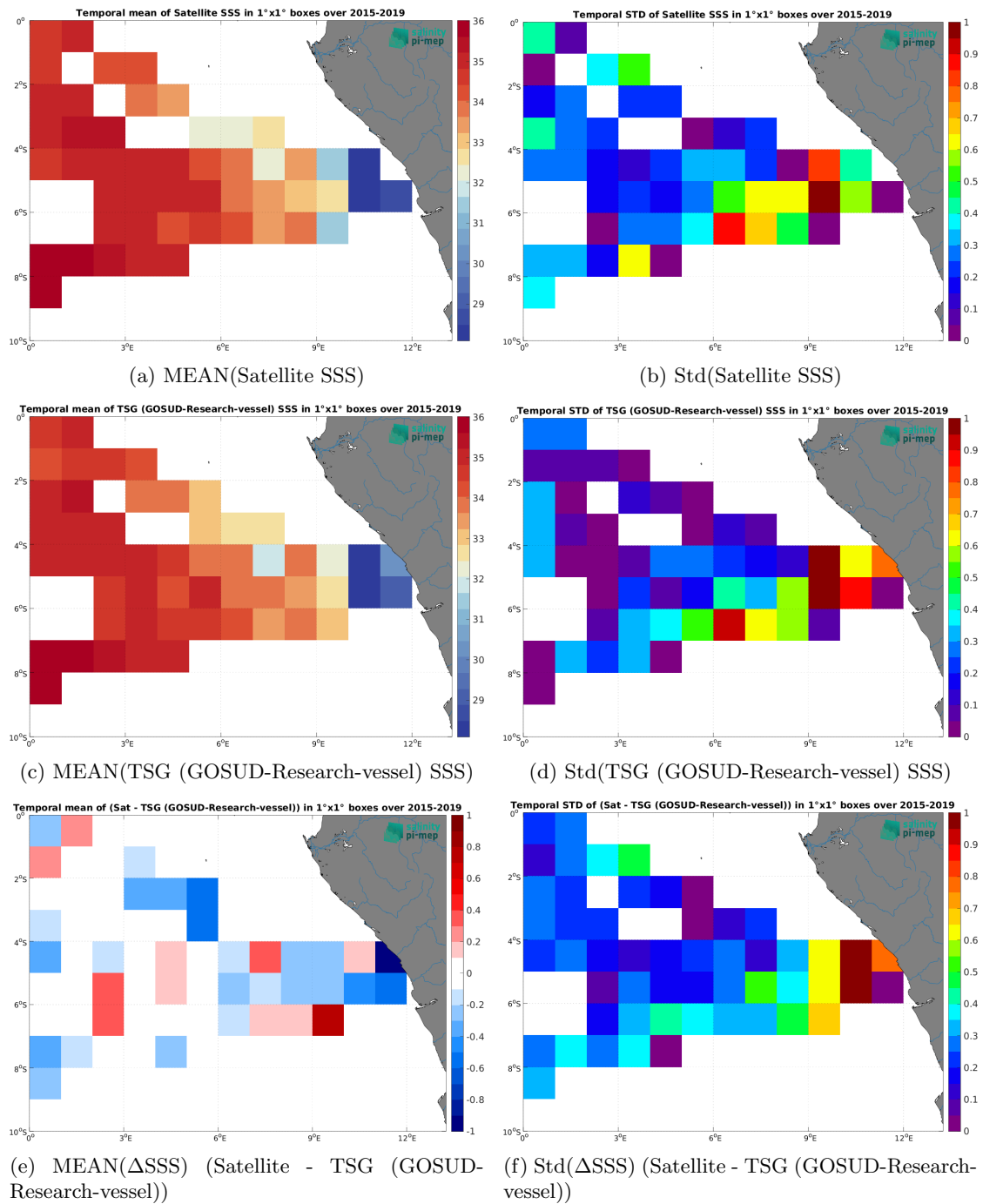
Figure 6: Temporal mean (left) and Std (right) of SSS from SMAP SSS L2 v5 (RSS) (top), TSG (GOSUD-Research-vessel) (middle), and of \Delta SSS (Satellite - TSG (GOSUD-Research-vessel)). Only match-up pairs are used to generate these maps.
