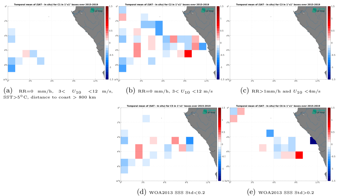
Figure 12: Temporal mean gridded over spatial boxes of size 1^\circ \times 1^\circ of \Delta SSS (SMAP SSS L2 v5 (RSS) - TSG (GOSUD-Research-vessel)) for 5 different subdatasets corresponding to:RR=0 mm/h, 3 < U_{10} < 12 m/s, SST>5°C, distance to coast > 800 km (a), RR=0 mm/h, 3 < U_{10} < 12 m/s (b), RR>1mm/h and U_{10} < 4 m/s (c), WOA2013 SSS Std<0.2 (d), WOA2013 SSS Std>0.2 (e).
