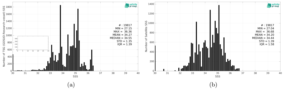
Figure 2: Histograms of SSS from TSG (GOSUD-Research-vessel) (a) and SMAP SSS L2 v5 (RSS) (b) considering all match-up pairs per bins of 0.1 over the Congo river plume Pi-MEP region and for the full satellite product period.
