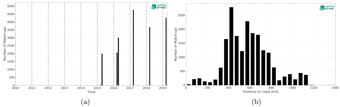
Figure 1: Number of match-ups between TSG (GOSUD-Research-vessel) and SMAP SSS L2 v5 (RSS) SSS as a function of time (a) and as function of the distance to coast (b) over the Congo river plume Pi-MEP region and for the full satellite product period.
